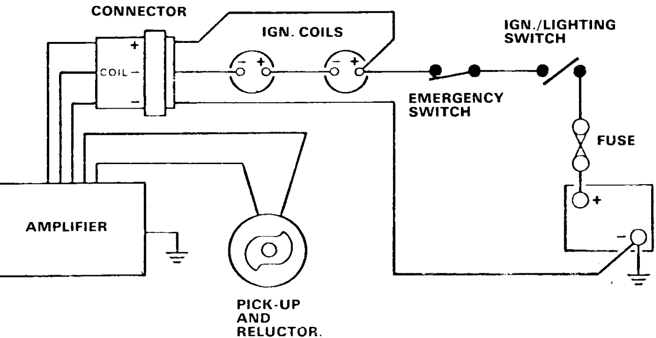
FIG. 3. IGNITION CIRCUIT
