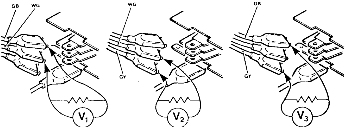
Fig. 6. ALTERNATOR AC CONTINUITY TEST
