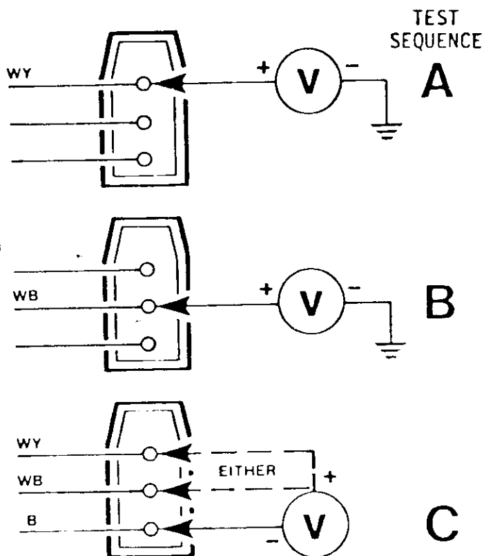
FIG. 10. AMPLIFIER MAIN HARNESS CONNECTOR, wiring tests
