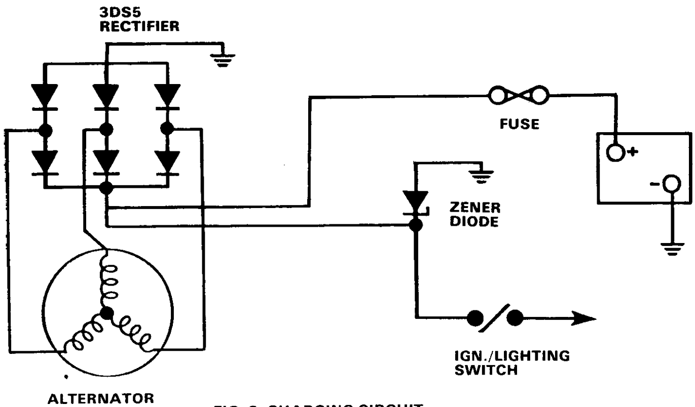
FIG. 2. CHARGING CIRCUIT
