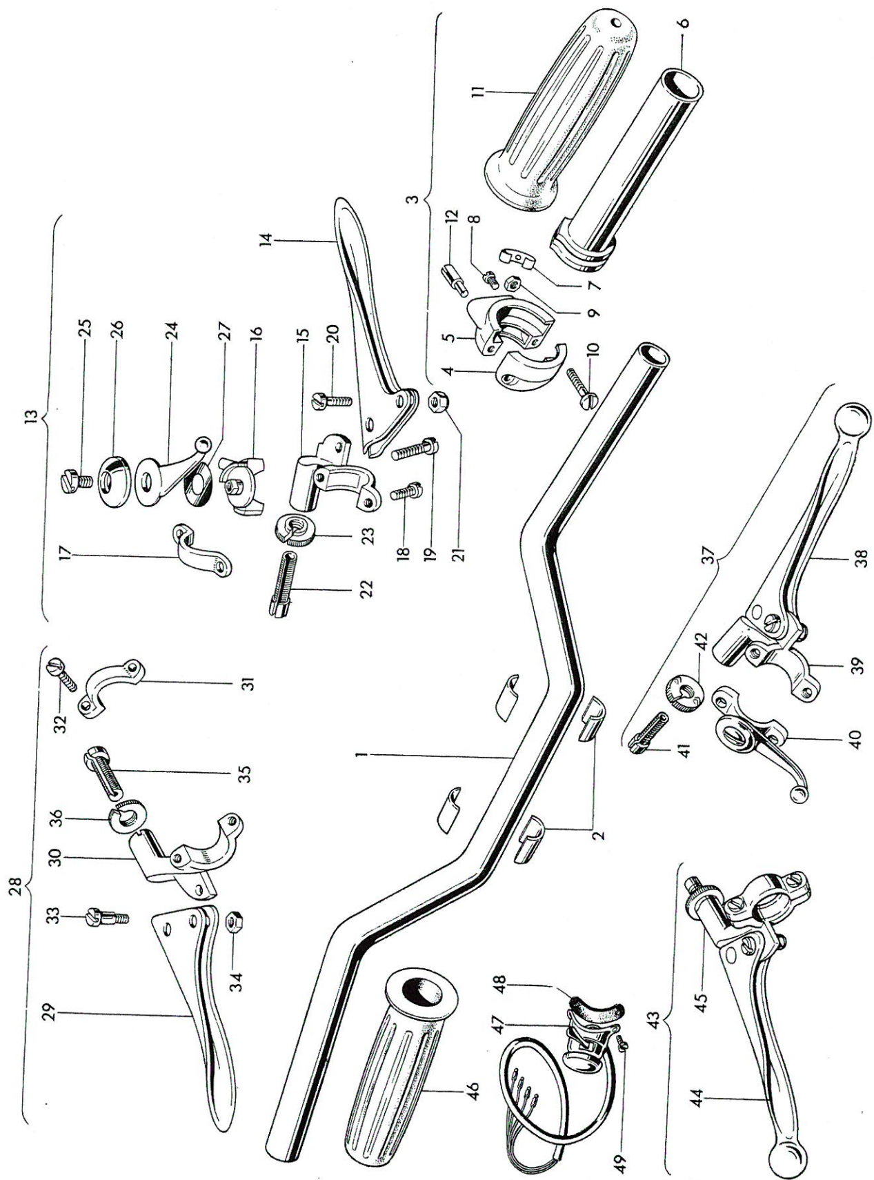
Fig. 27. HANDLEBARS AND CONTROL LEVERS
