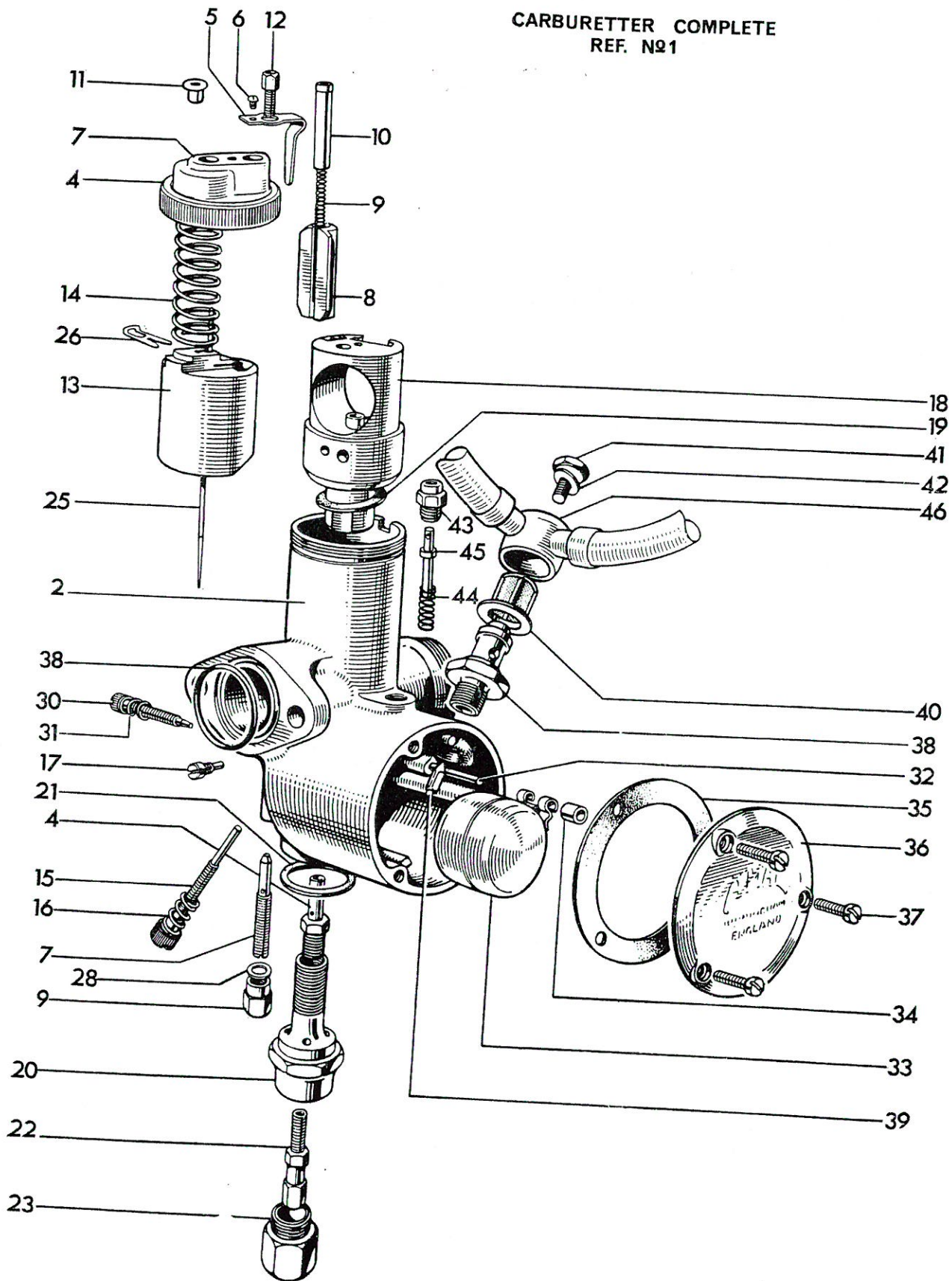
Fig. 30. AMAL CARBURETTER, TR 6
