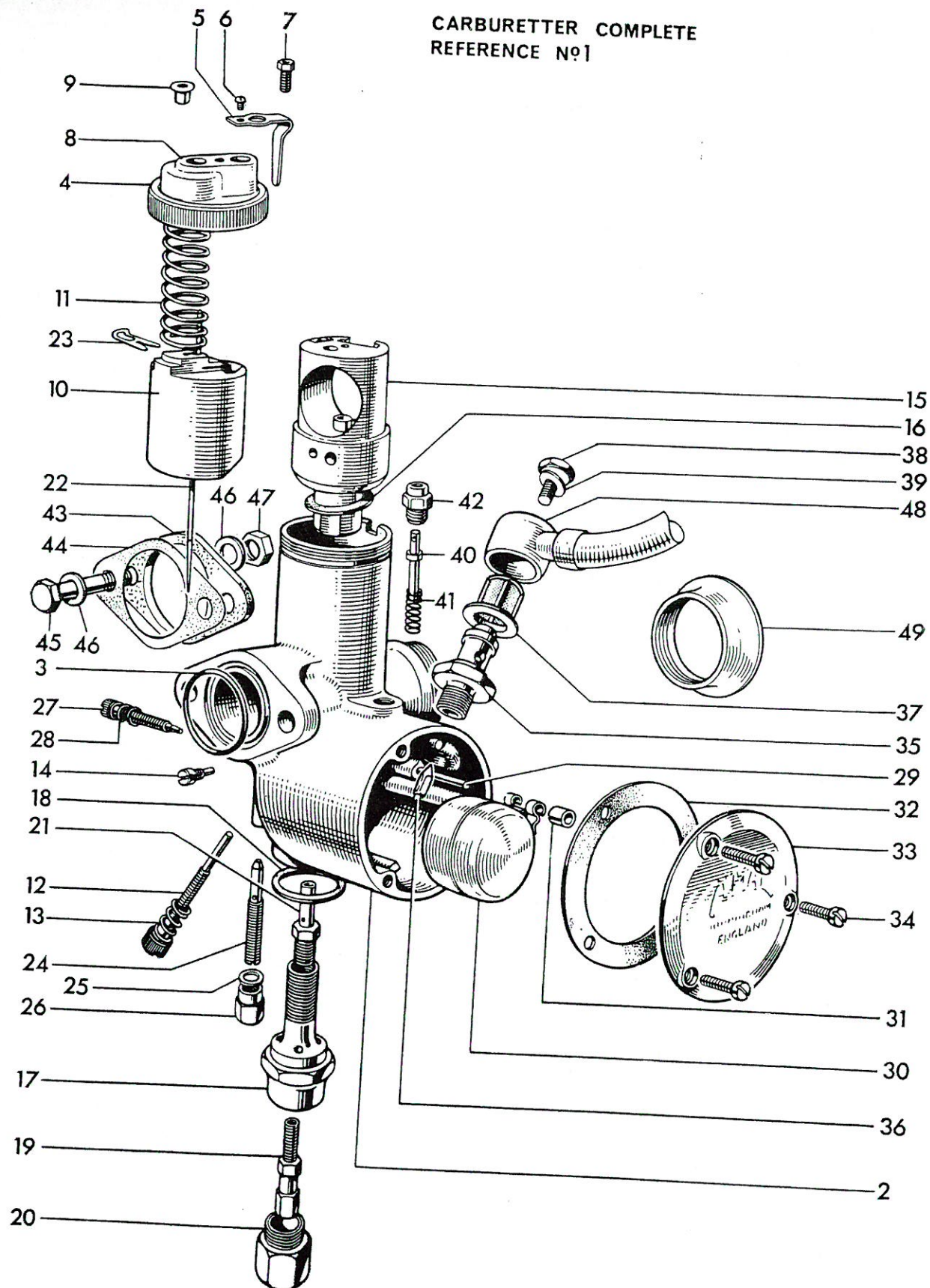
Fig. 32. AMAL CARBURETTER, T120R AND T120TT
