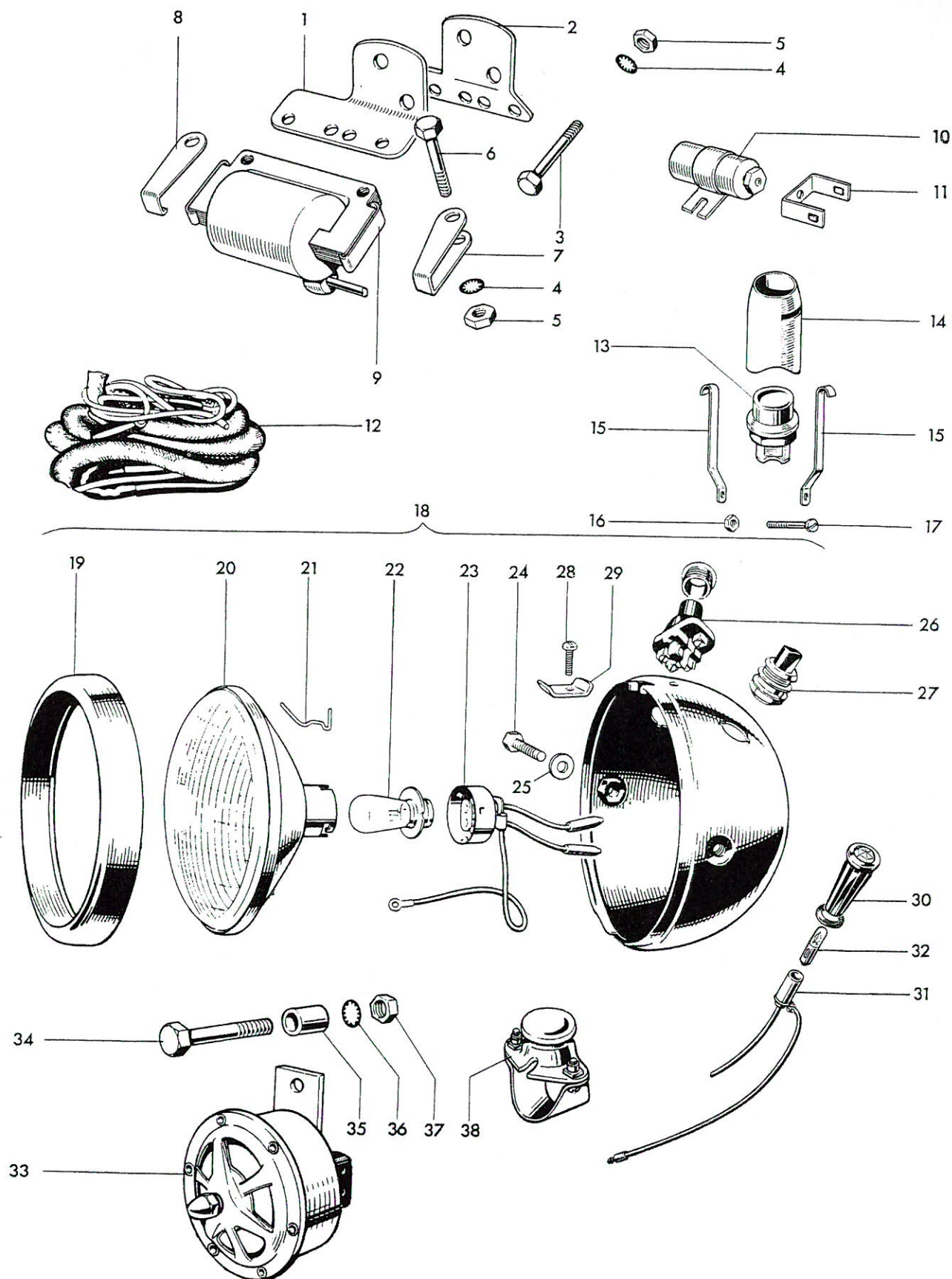
Fig. 34. A.C. MAGNETO IGNITION COILS AND DIRECT LIGHTING
