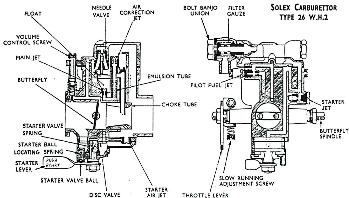
Fig. 12. SOLEX CARBURETTER.
