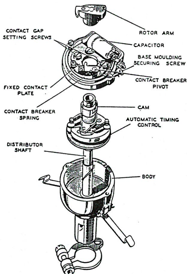
Fig. 14. DISTRIBUTOR, TYPE DKX2A.
