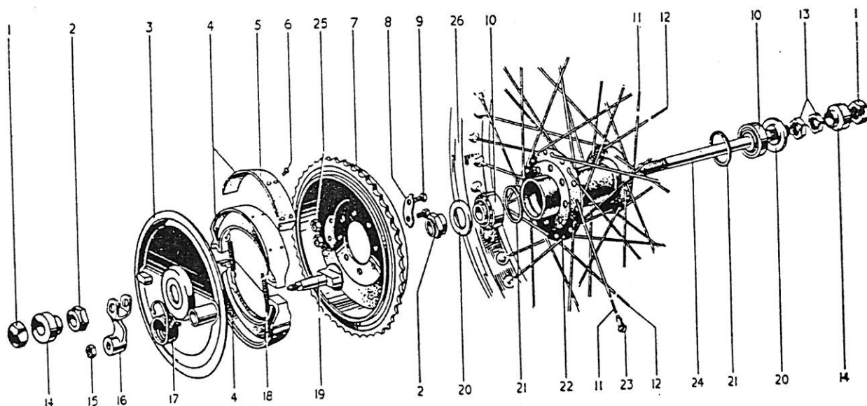
Fig. 9. REAR WHEEL.
