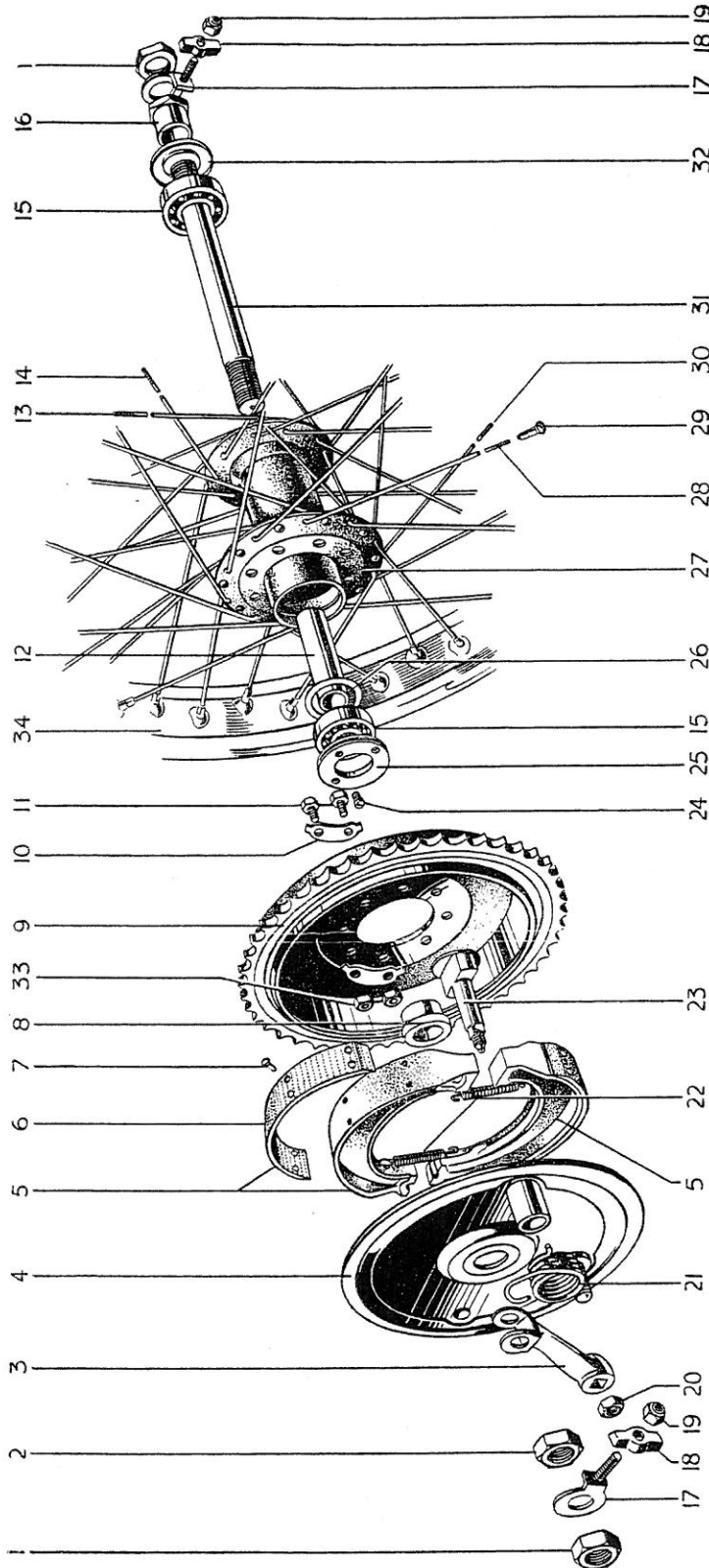
FIG. 19. REAR WHEEL
