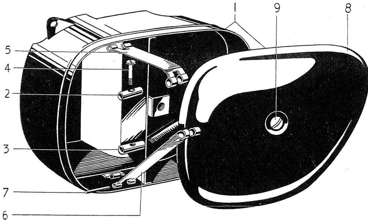
FIG. 26. BATTERY CARRIER AND TOOL BOX
