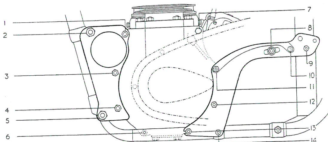
FIG. 14. ENGINE PLATE—STUDS, BOLTS, NUTS AND WASHERS
