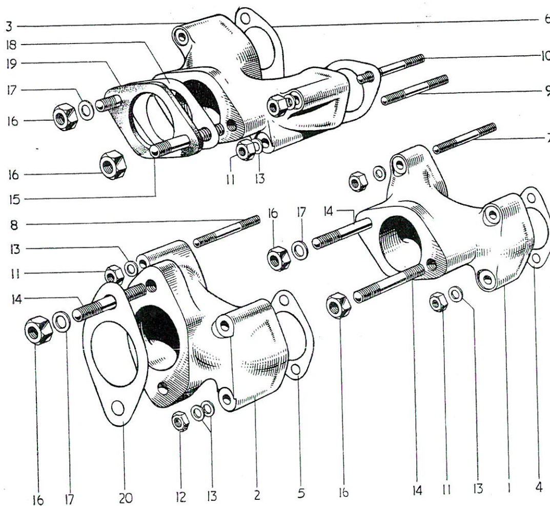
FIG. 1. INLET MANIFOLDS
