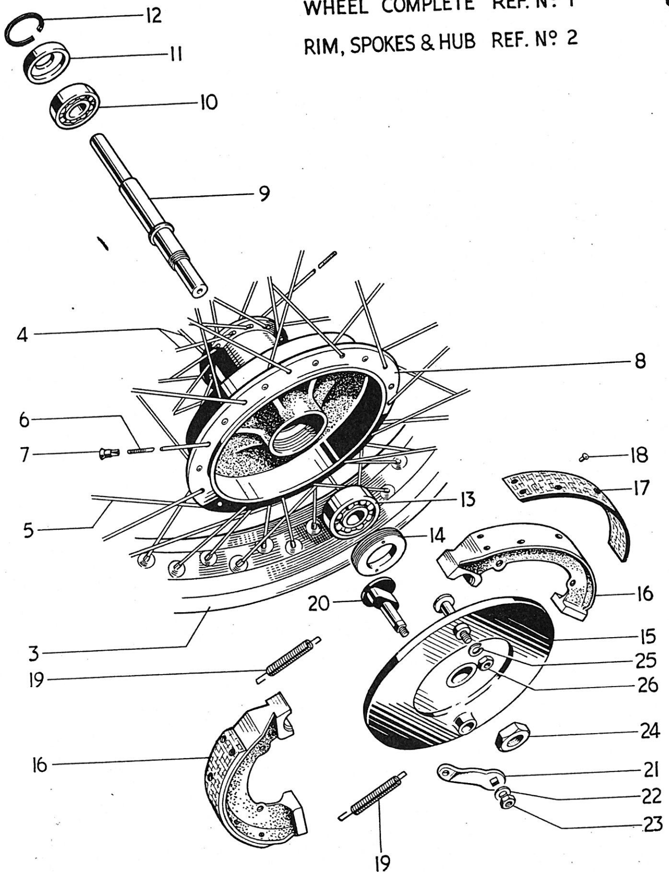
Fig. 11. FRONT WHEEL, T20.
