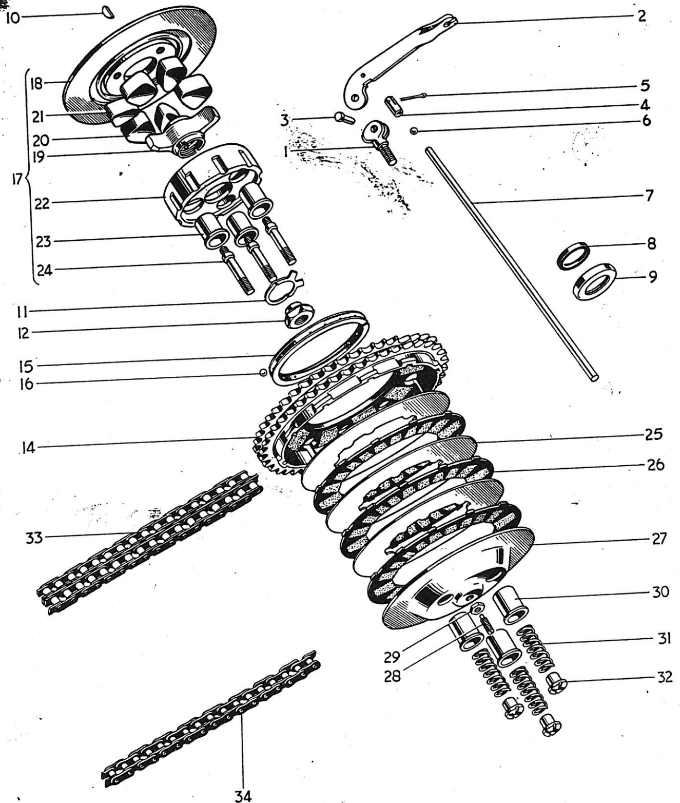
Fig. 6. CLUTCH AND CHAINS
