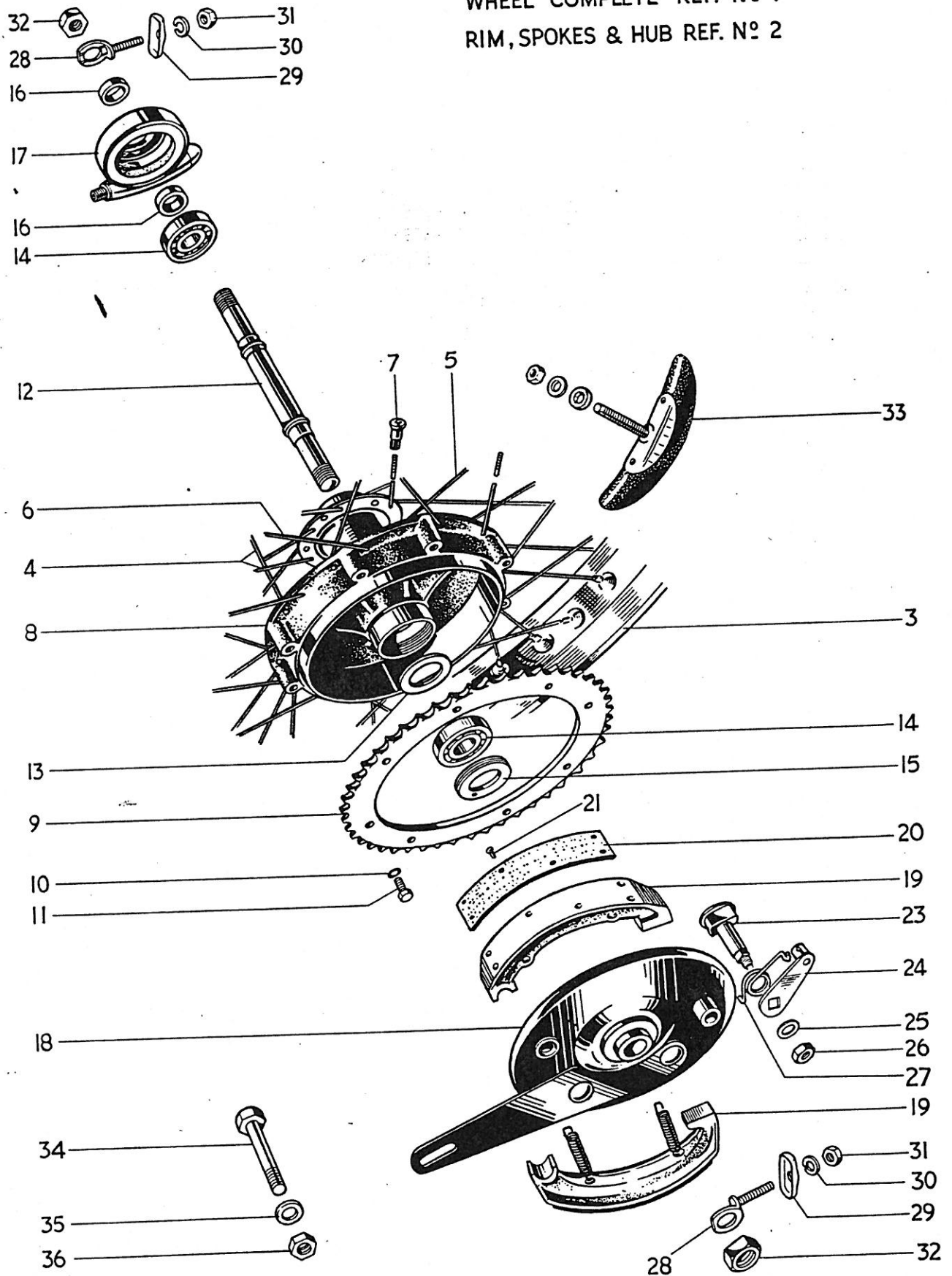
Fig. 13. REAR WHEEL
