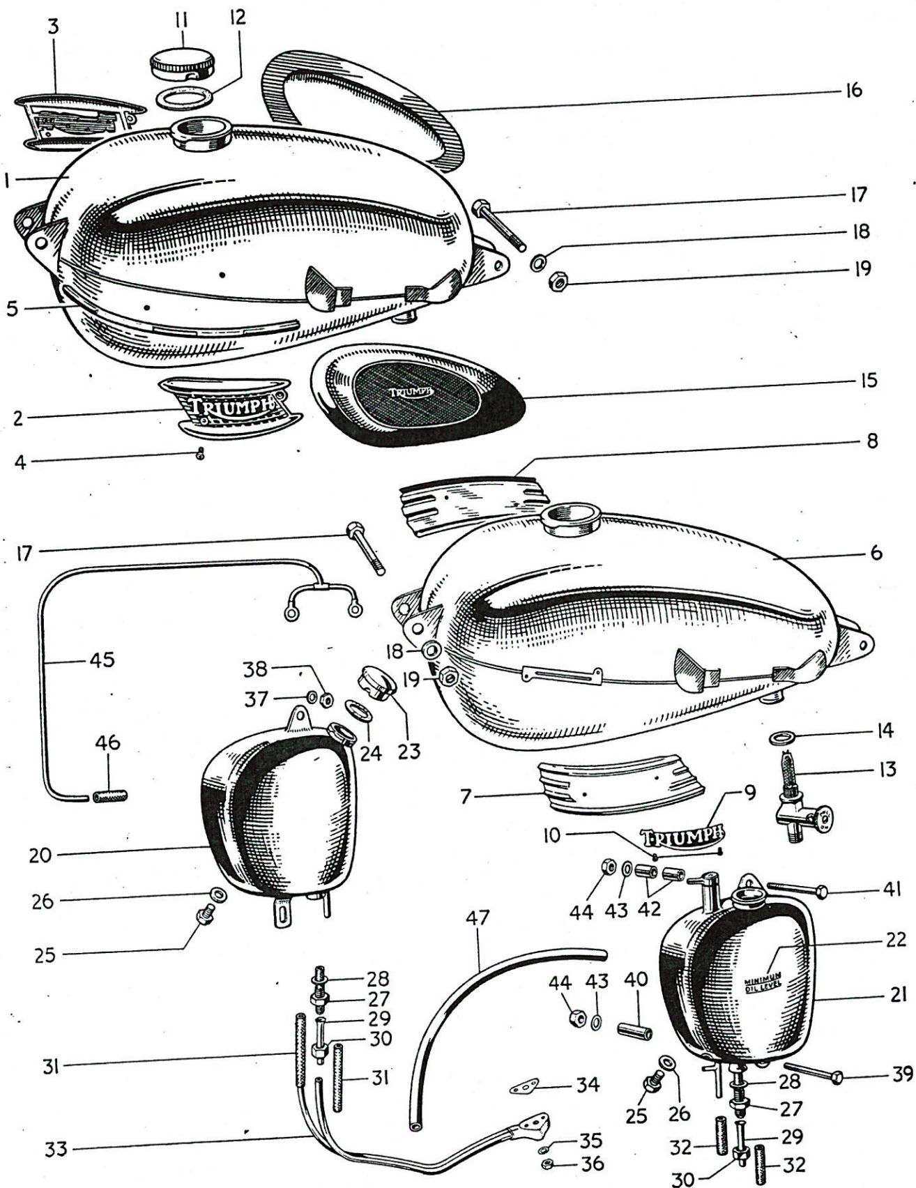
Fig. 16. PETROL AND OIL TANKS
