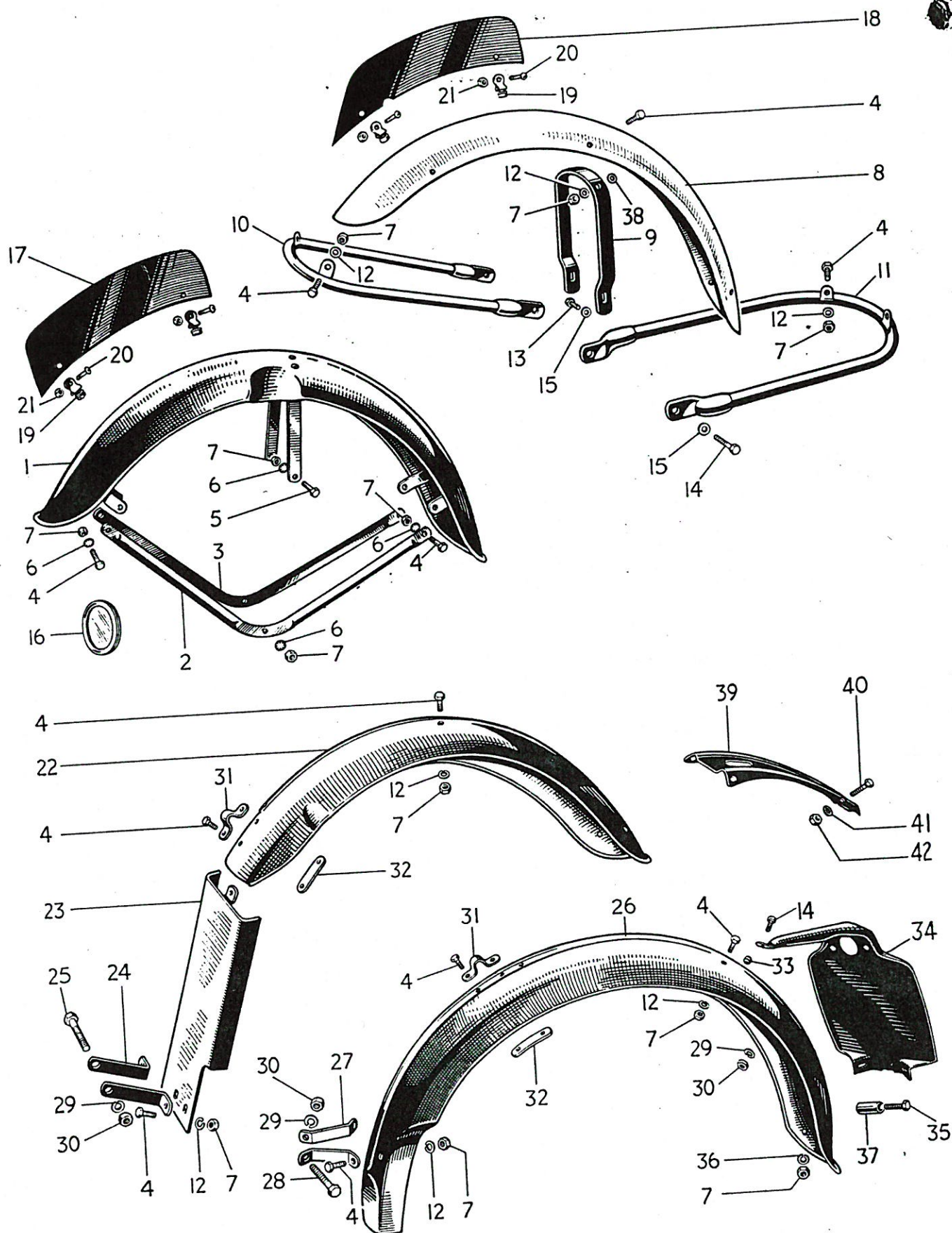
Fig. 14. MUDGUARDS AND NUMBER PLATES
