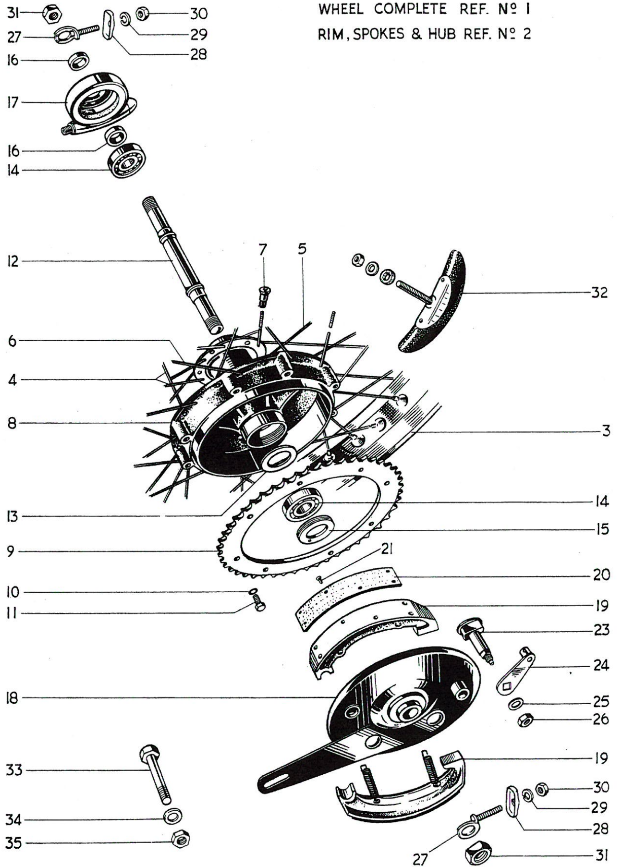
Fig. 17. REAR WHEEL.
