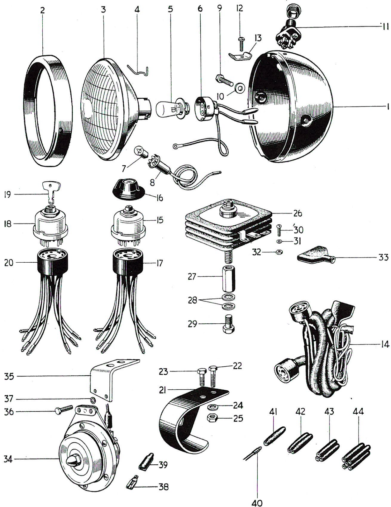
Fig. 28. T20SH ELECTRICAL EQUIPMENT.
