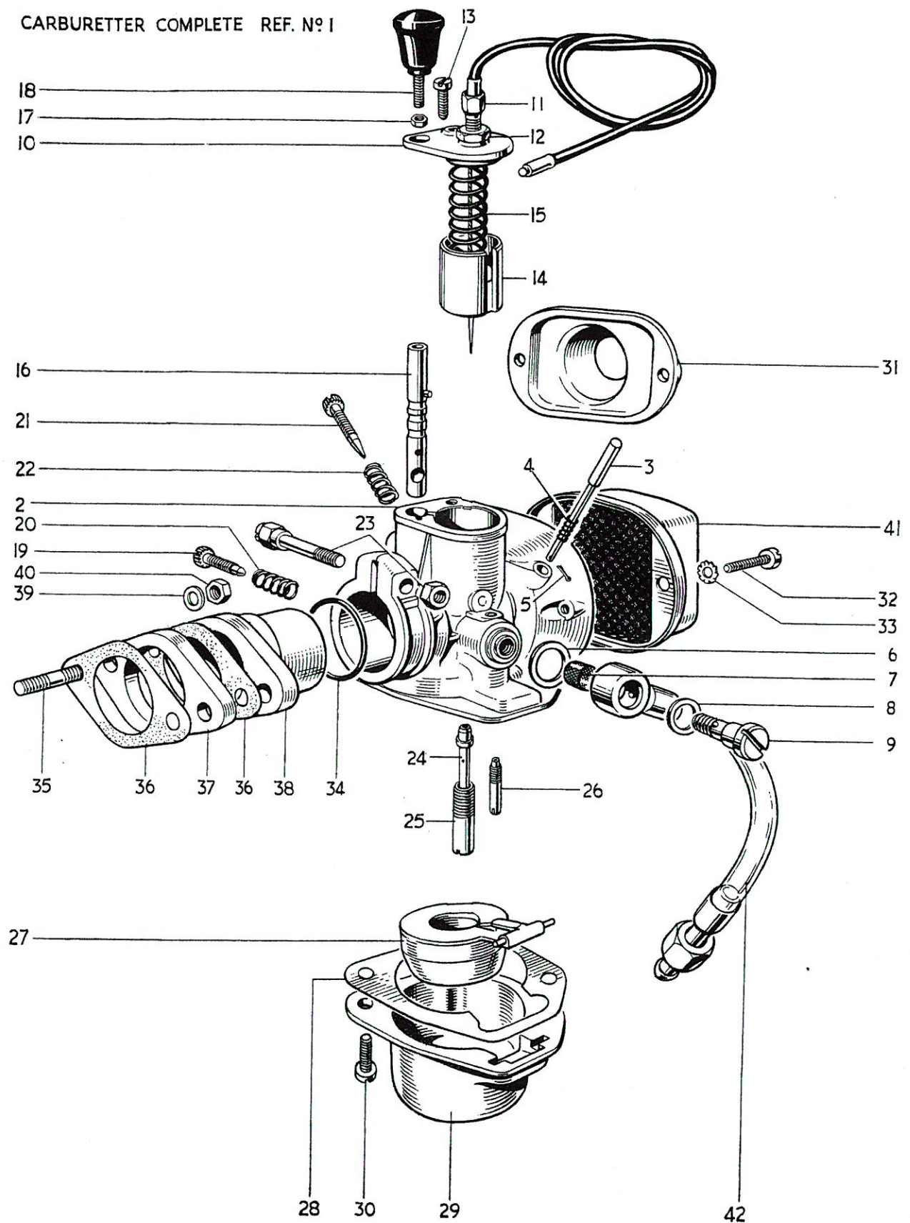
Fig. 25. ZENITH CARBURETTER.
