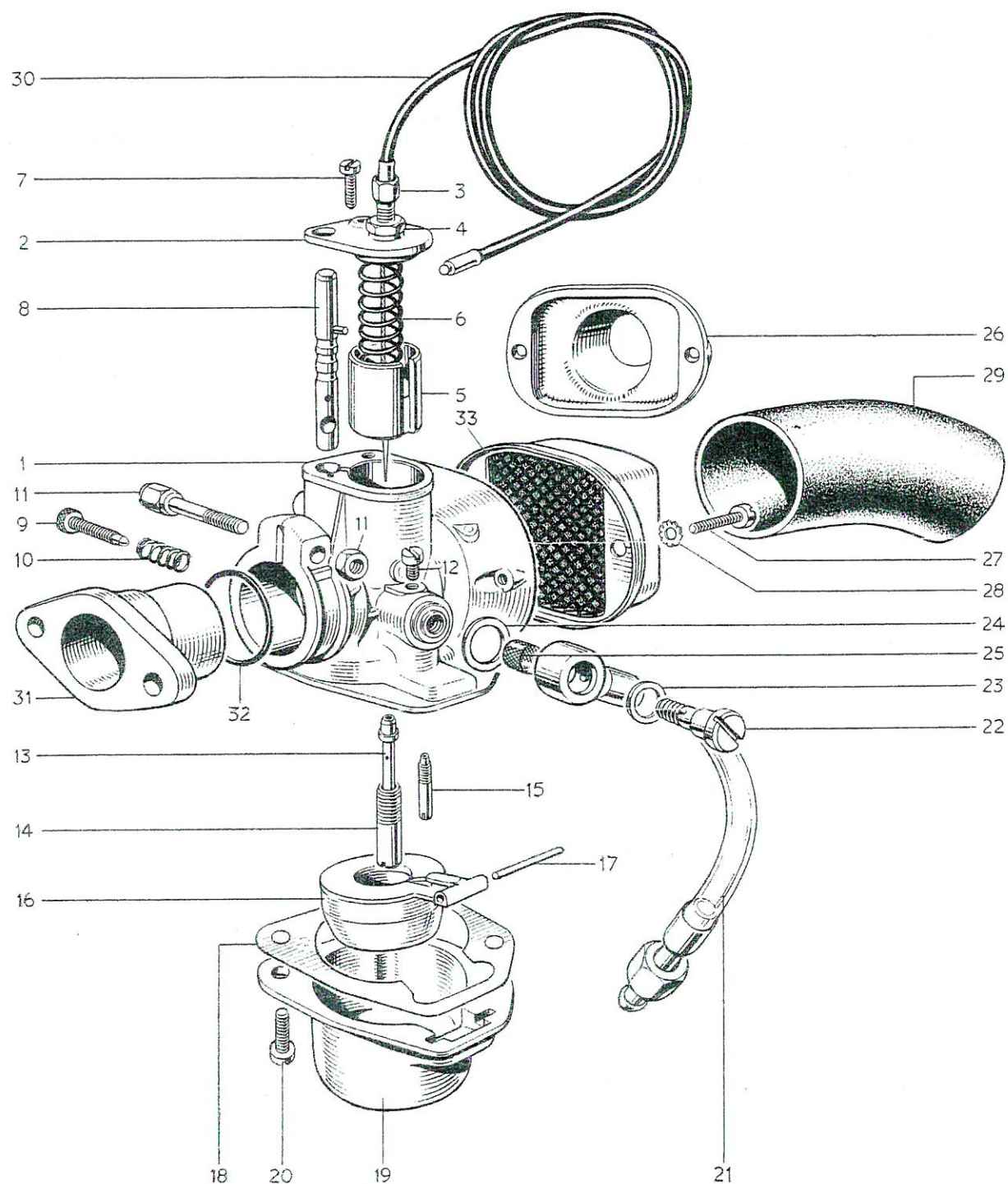
FIG. 15. ZENITH CARBURETTER
