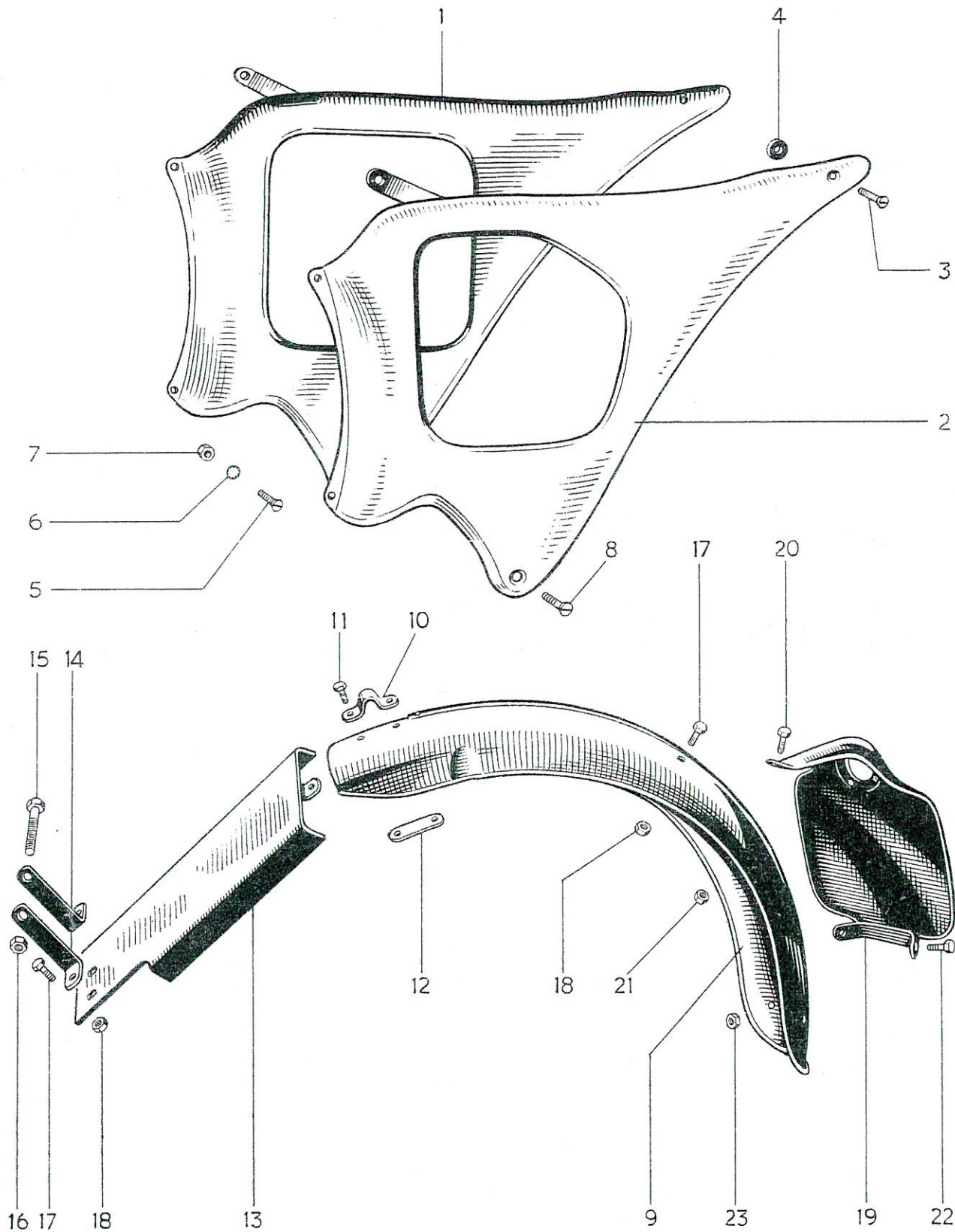
FIG. 10. REAR PANELS.
