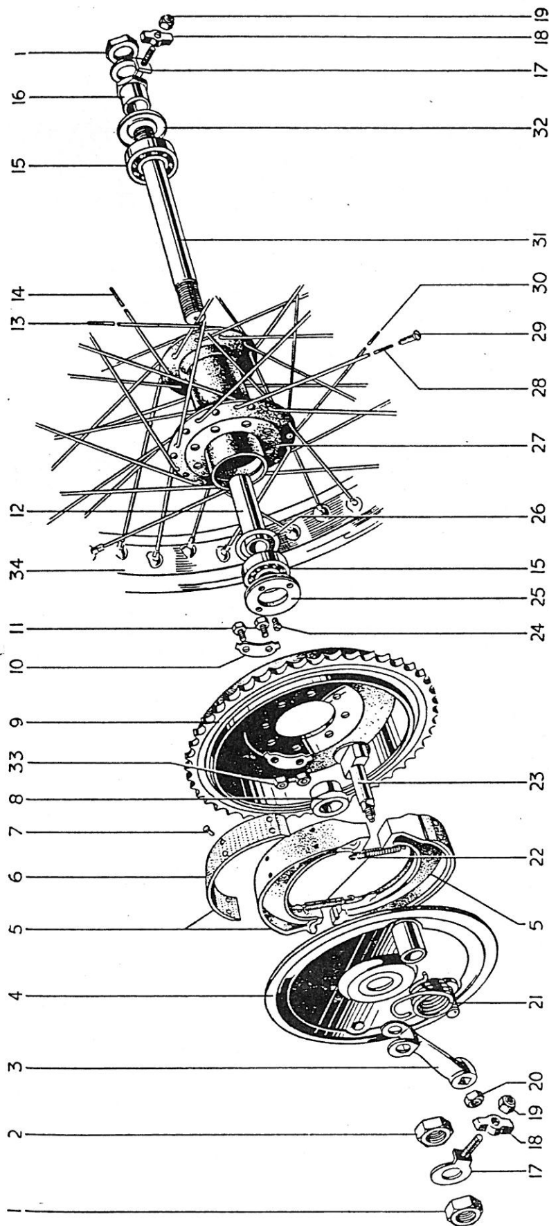
FIG. 19. REAR WHEEL
