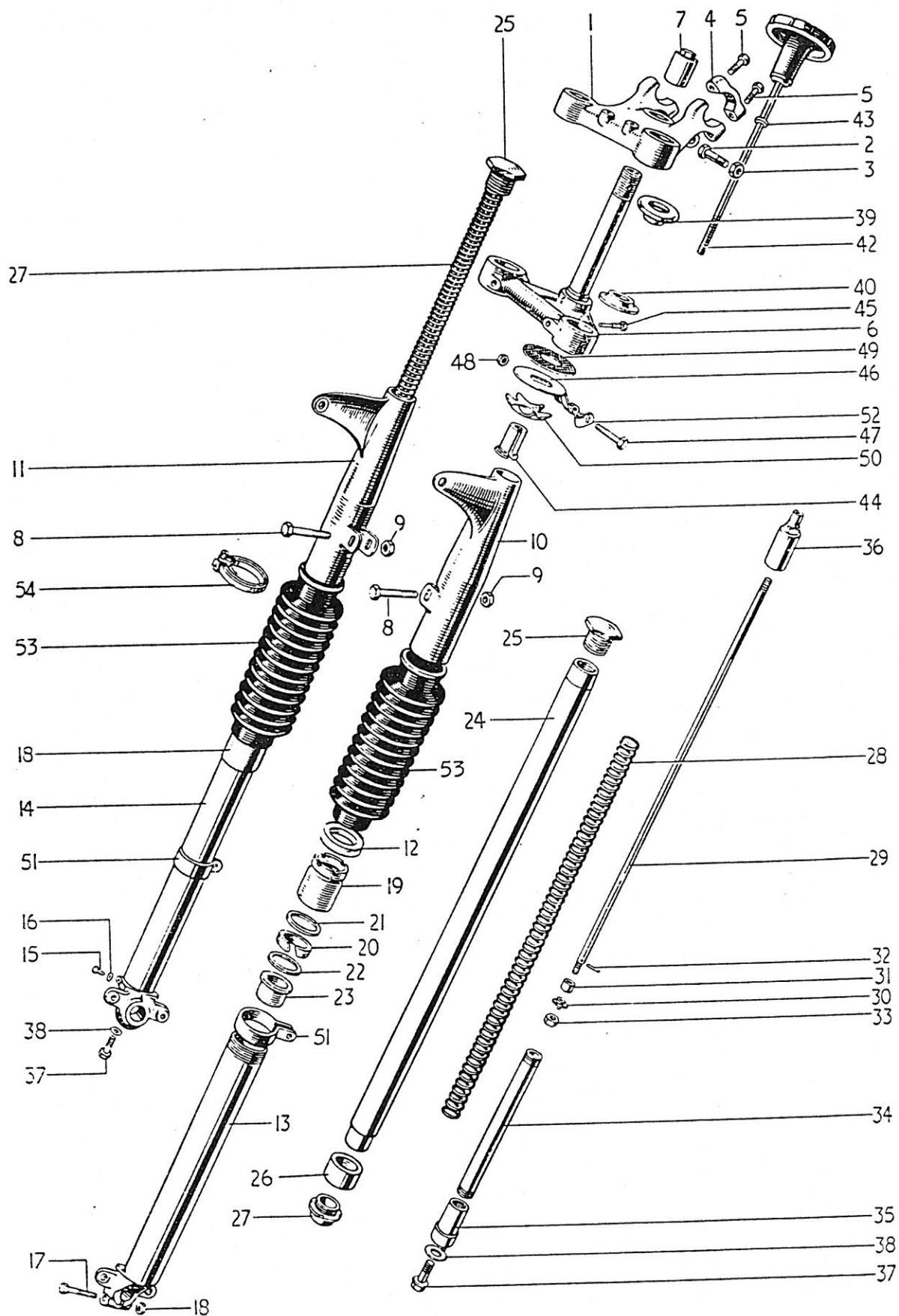
FIG. 16. TELESCOPIC FORK (TROPHY)
