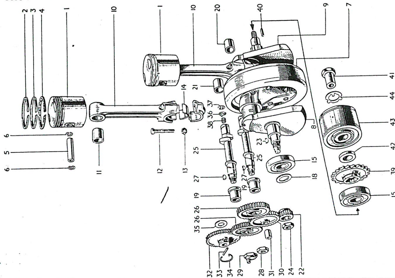
FIG. 3. CRANKSHAFT, CONNECTING RODS, PISTONS, TIMING GEAR, etc.
