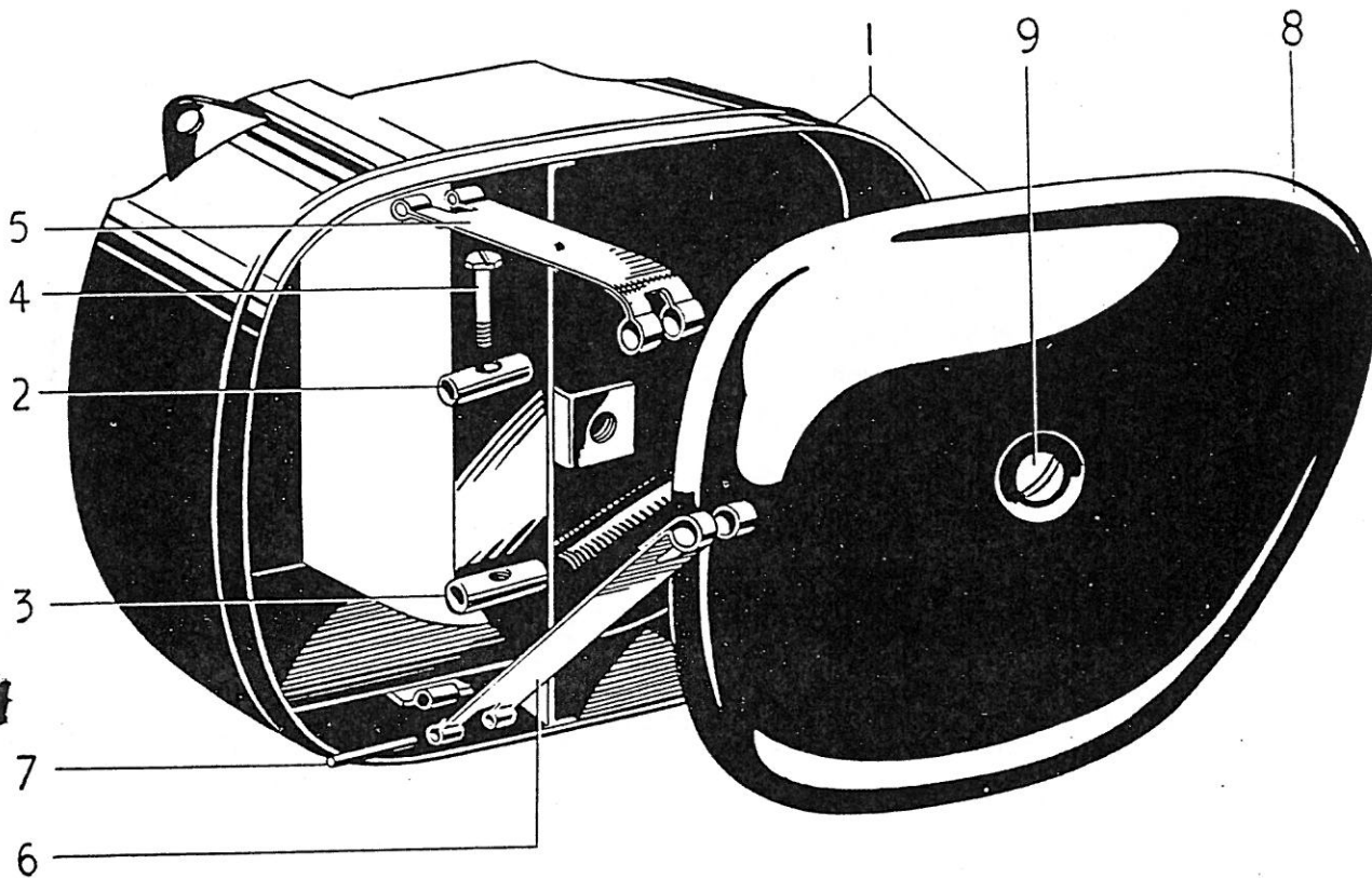
FIG. 26. BATTERY CARRIER AND TOOL BOX
