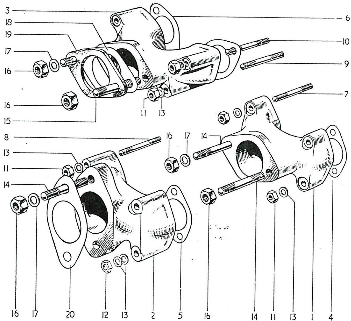
FIG. I. INLET MANIFOLDS
