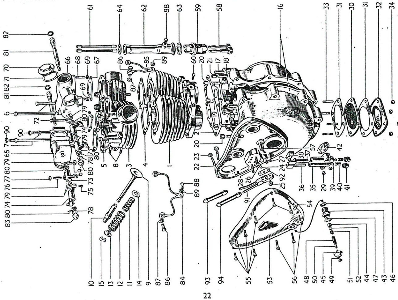
FIG. 4. CRANKCASE, CYLINDER BLOCK, CYLINDER HEAD, etc.
