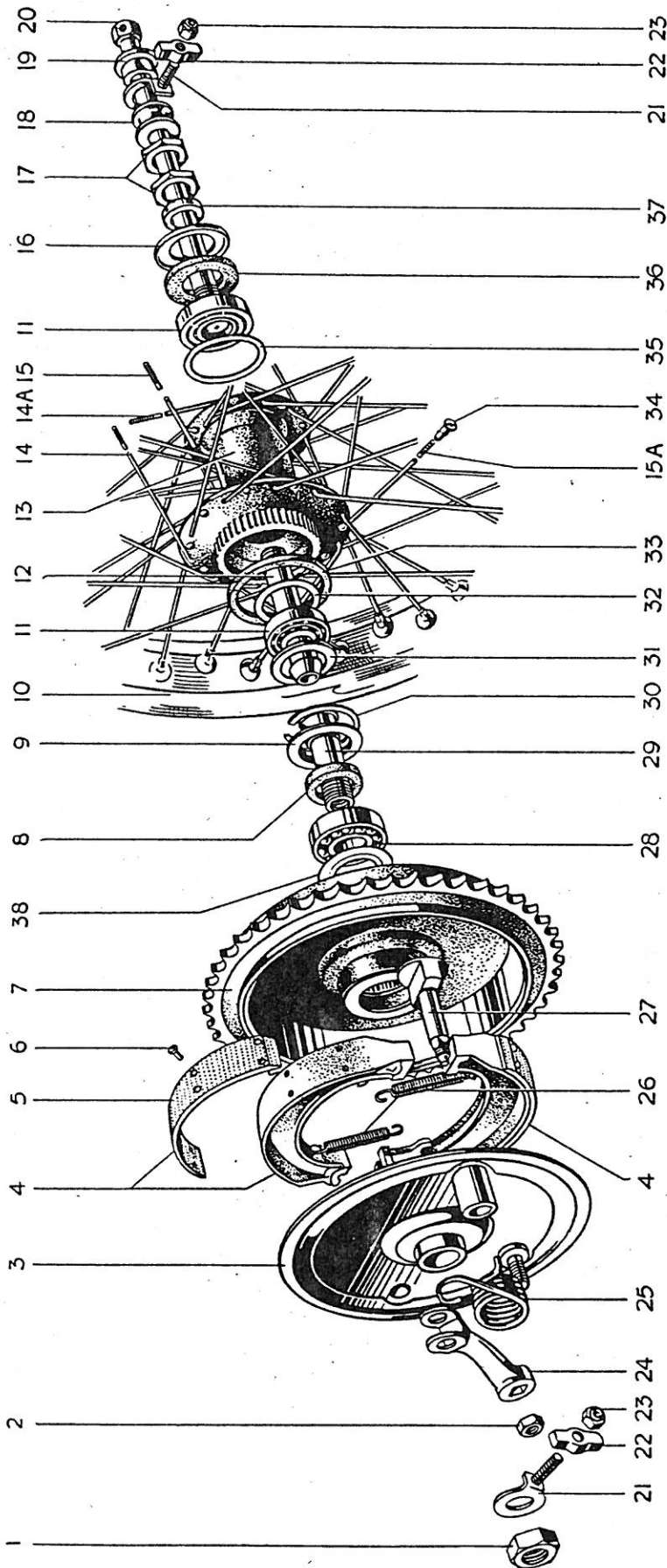
FIG. 21. REAR WHEEL (QUICKLY DETACHABLE)
