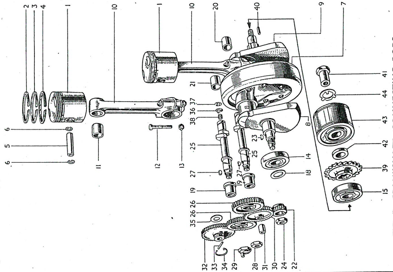
FIG. 5. CRANKSHAFT, CONNECTING RODS, PISTON TIMING GEAR, etc.
