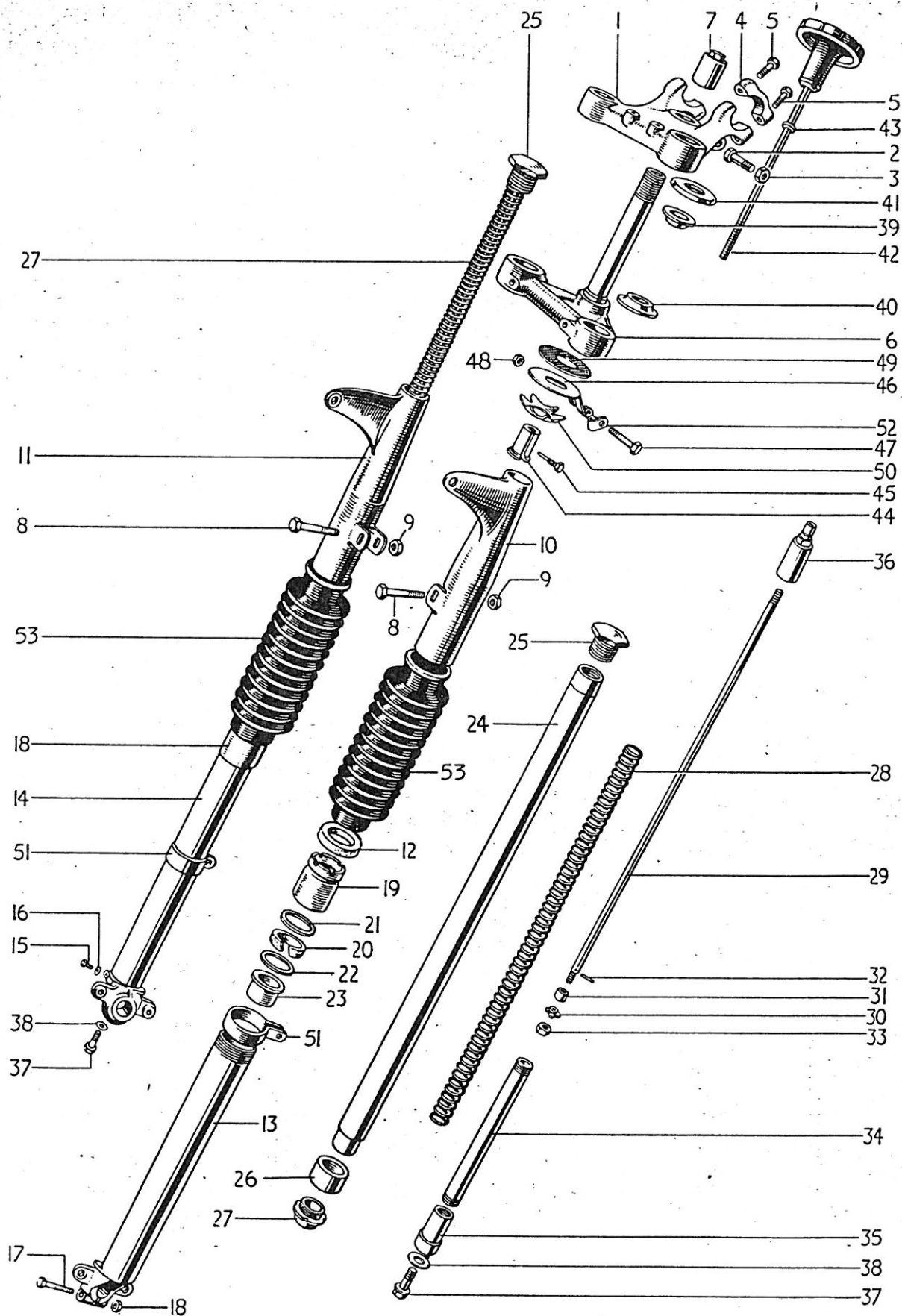
FIG. 17. TELESCOPIC FORK (TROPHY)
