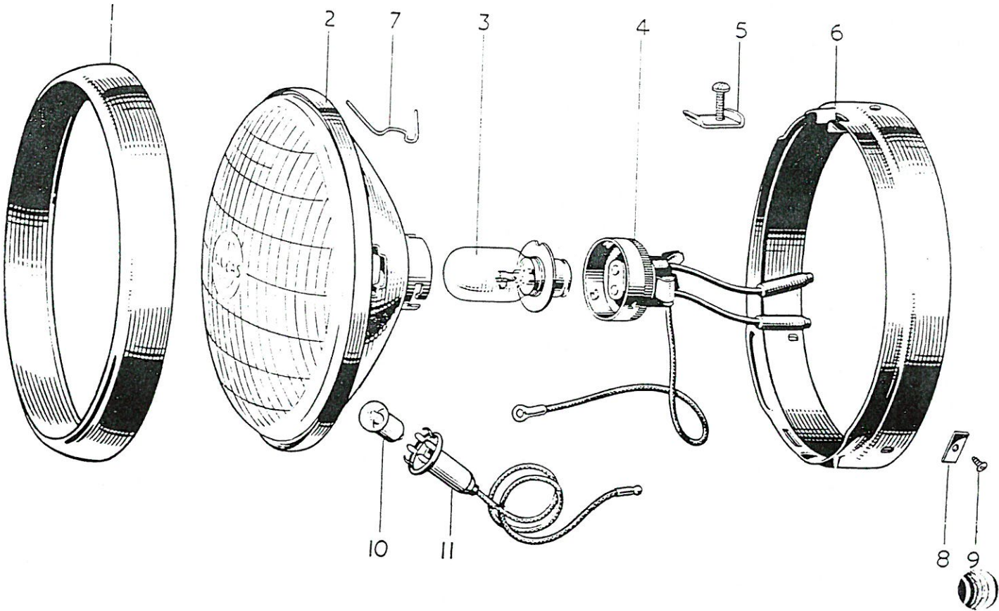
FIG. 20 LUCAS HEADLAMP TYPE MCF700P
