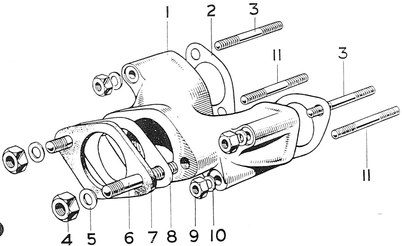
FIG. 1 INLET MANIFOLD
