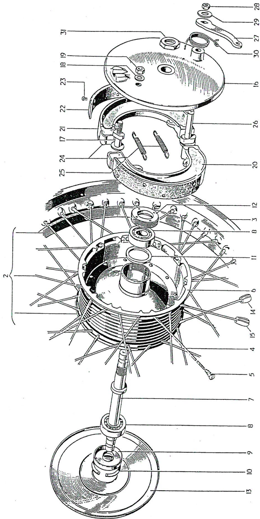
Fig. 17. FRONT WHEEL
