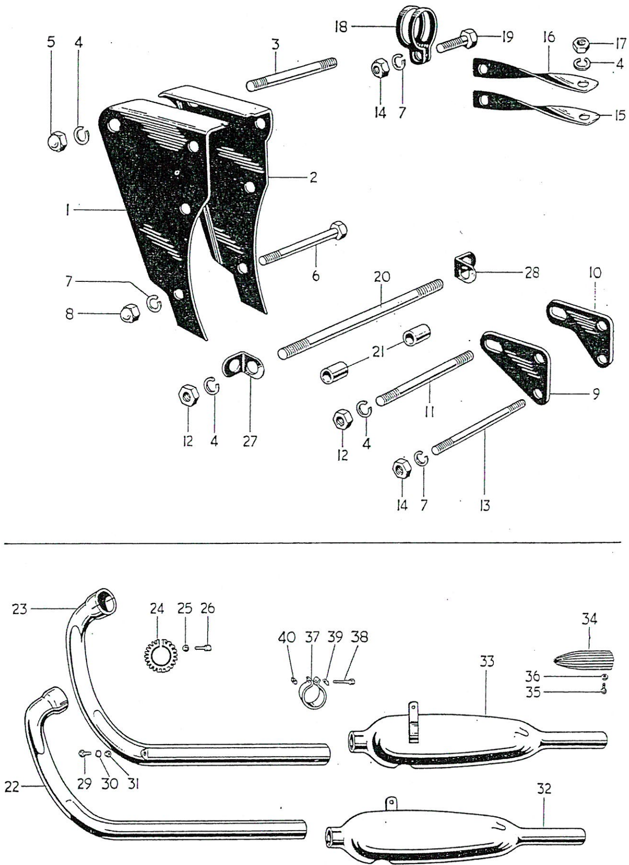
Fig. 10 ENGINE FITTINGS AND EXHAUST SYSTEM.
