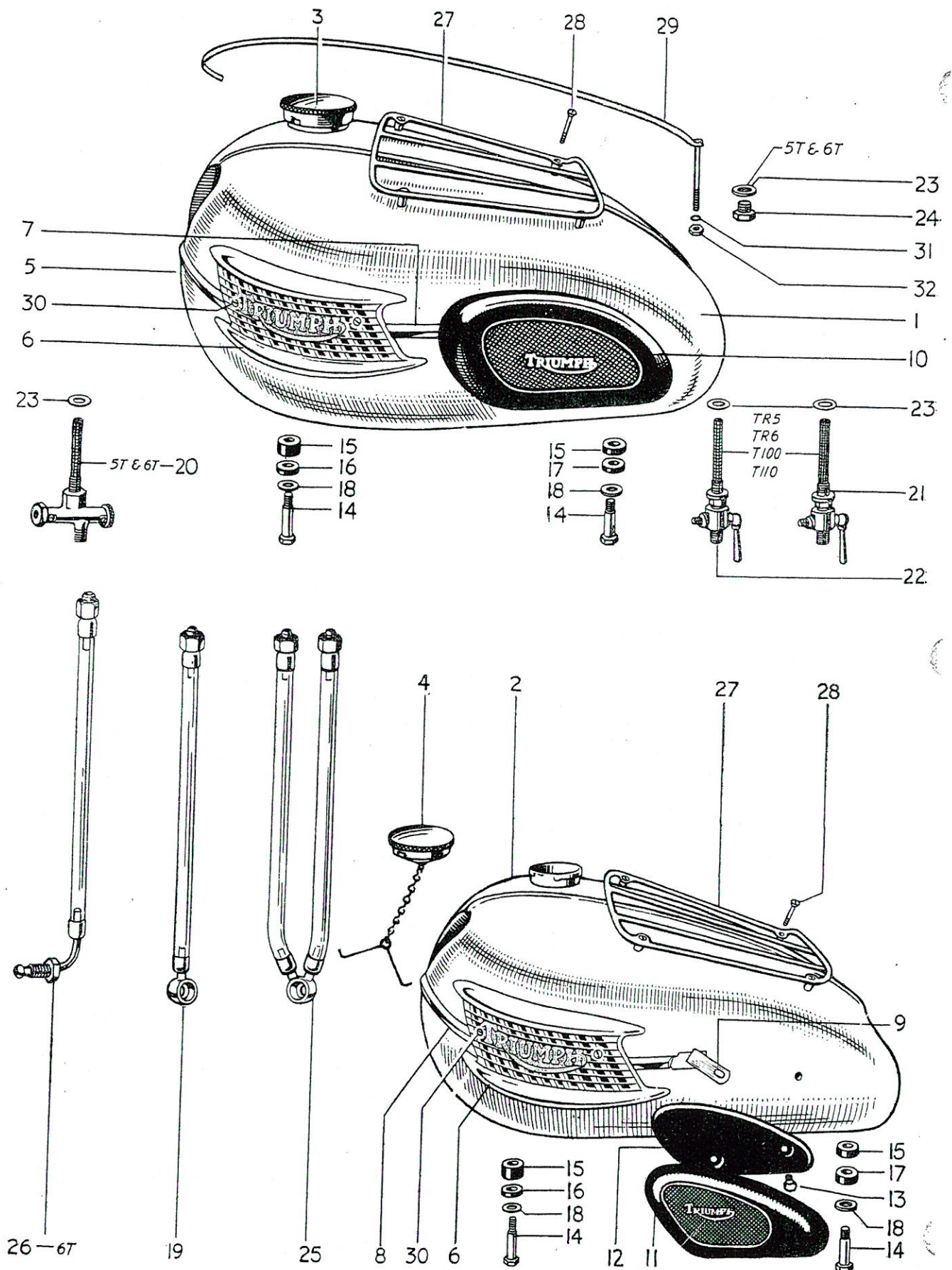
FIG. 22. PETROL TANKS AND FITTINGS
