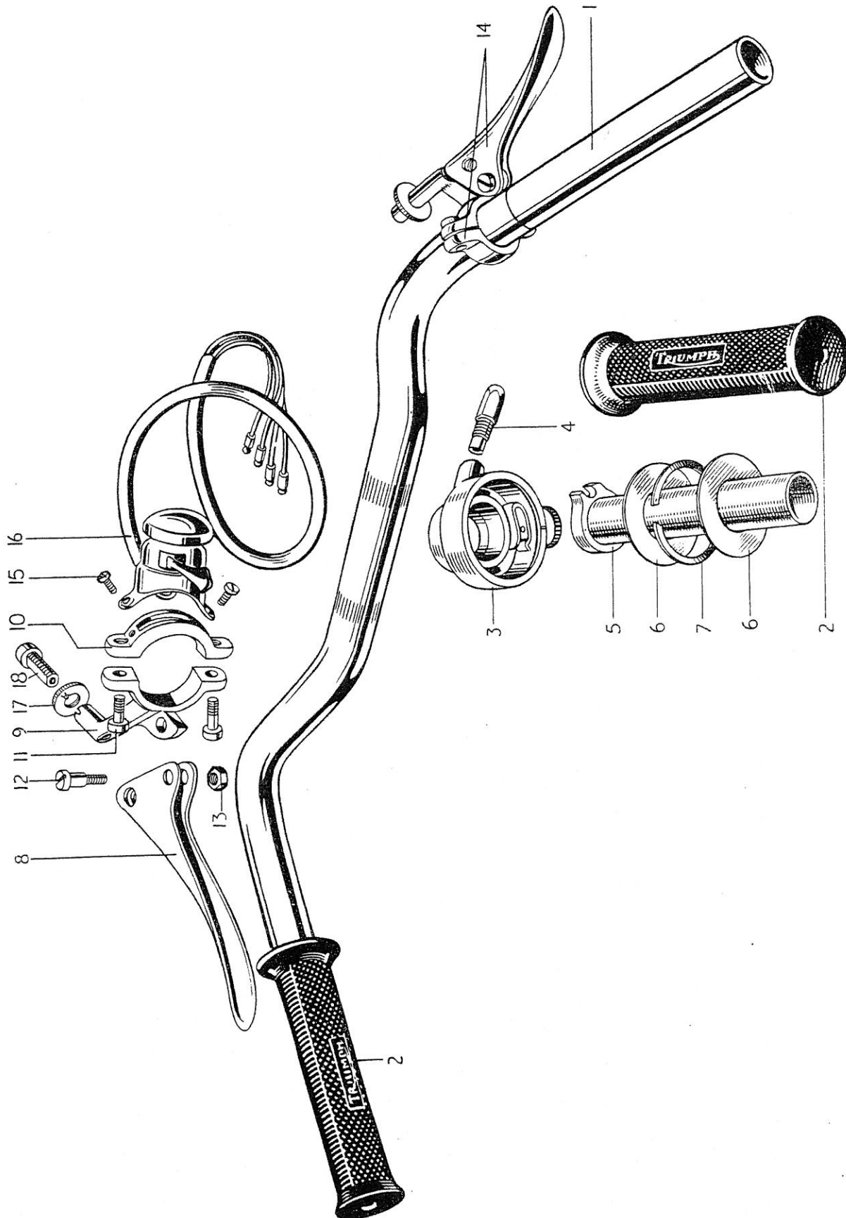
FIG. 25. HANDLEBAR AND CONTROLS
