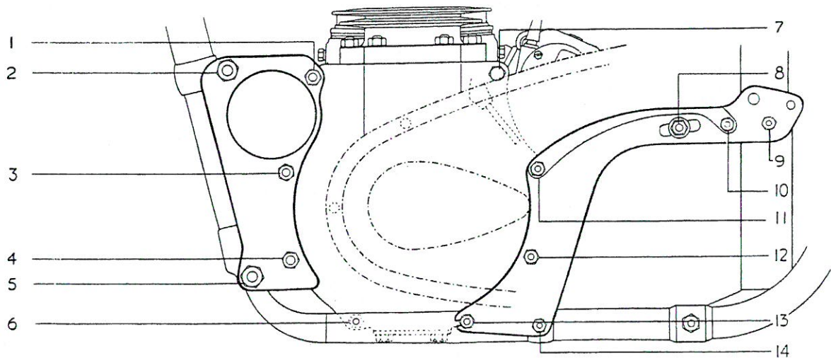
FIG. 14. ENGINE PLATE—STUDS, BOLTS, NUTS AND WASHERS
