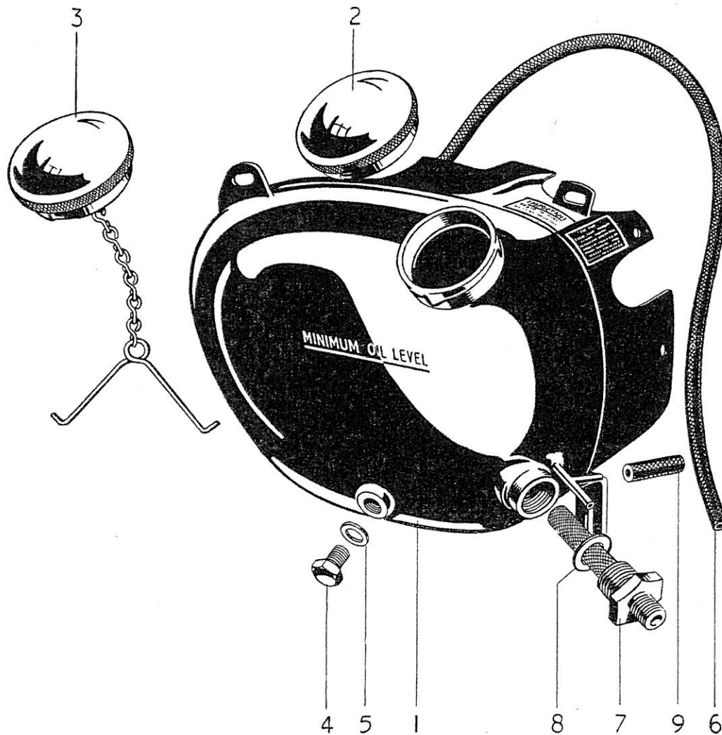
FIG. 23. OIL TANK
