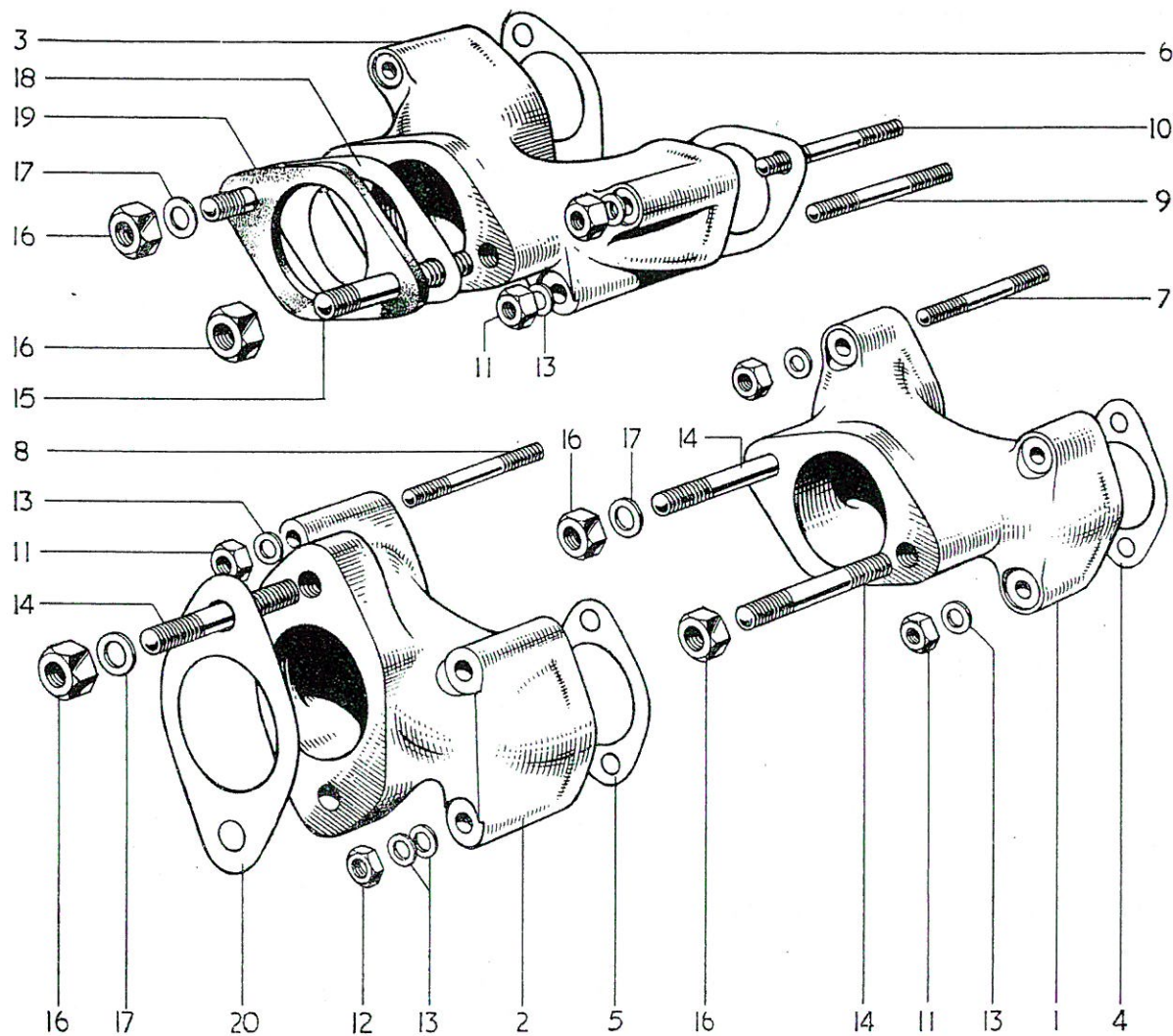
FIG. 1. INLET MANIFOLDS
