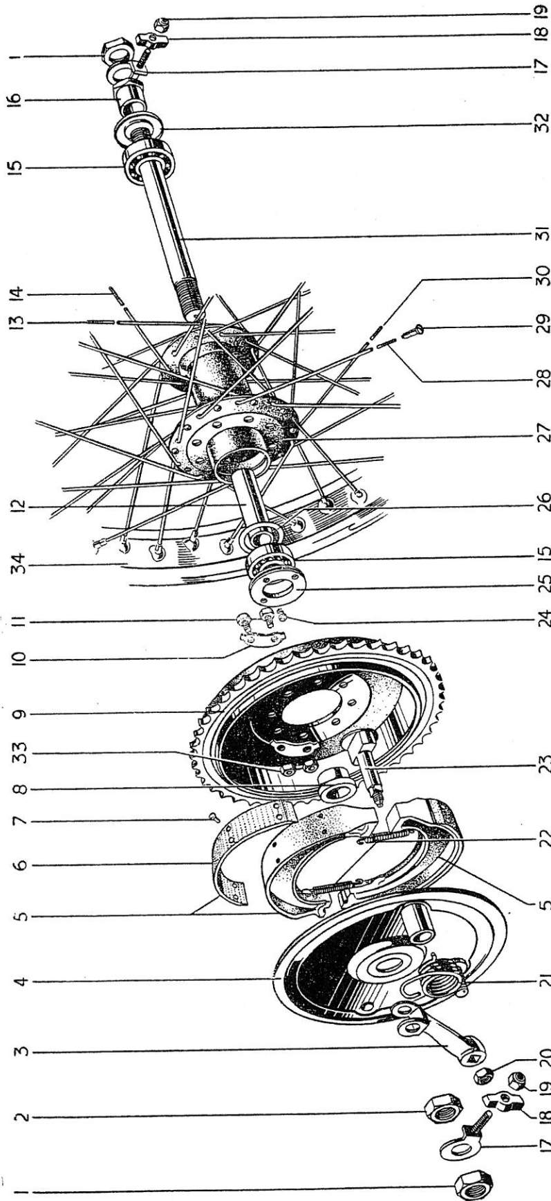
FIG. 19. REAR WHEEL
