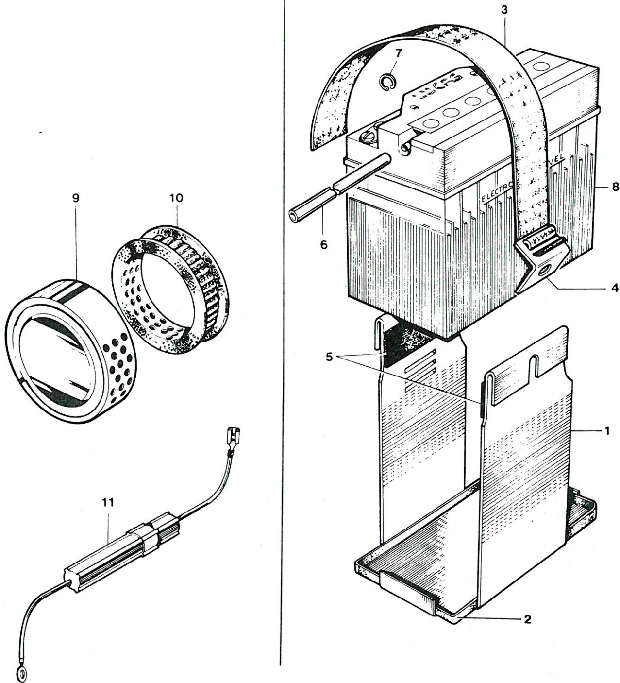
Fig. 23. BATTERY CARRIER AND AIR FILTERS
