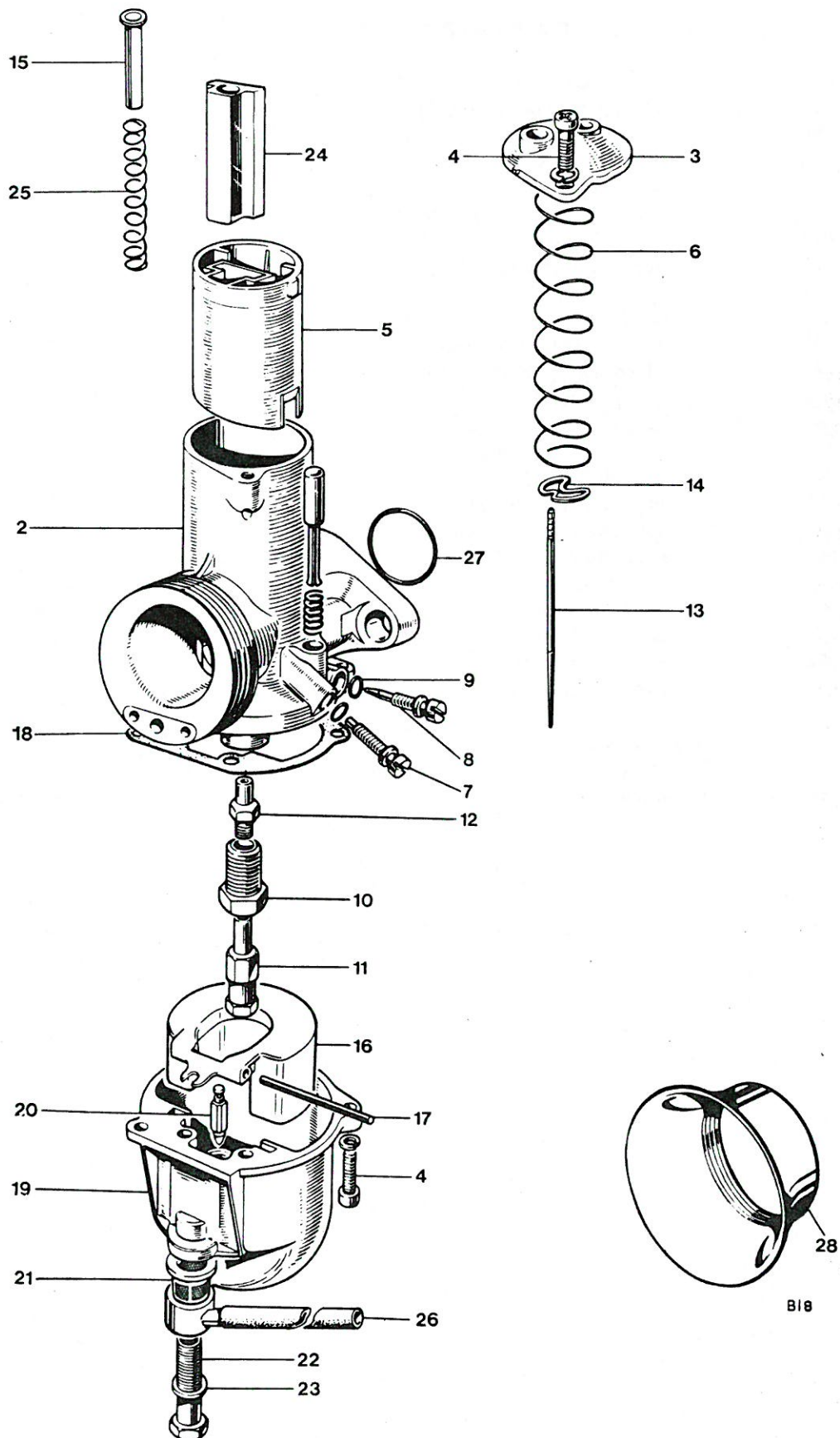
Fig. 30. AMAL CARBURETOR, T120R
