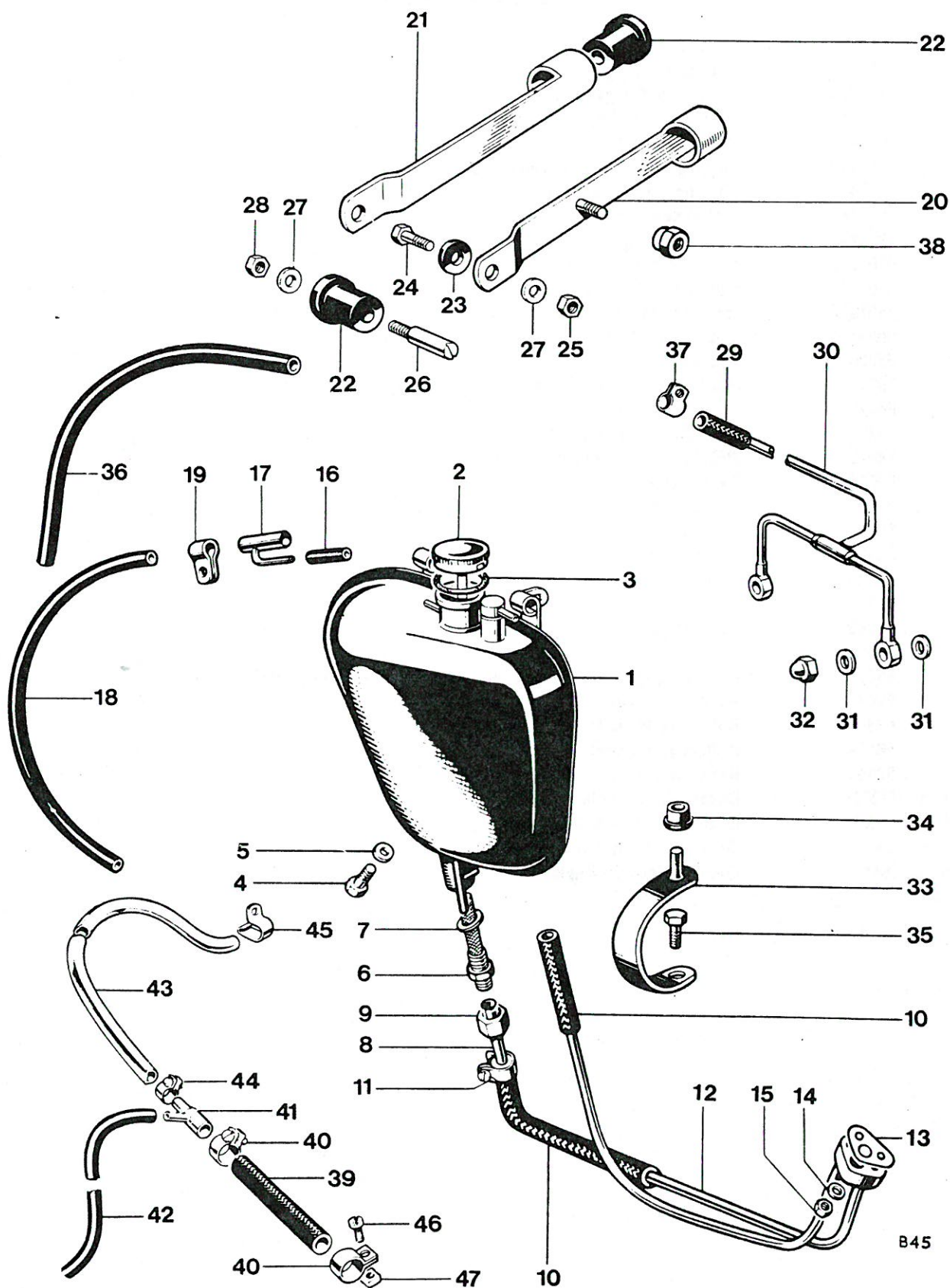
Fig. 22. OIL TANK
