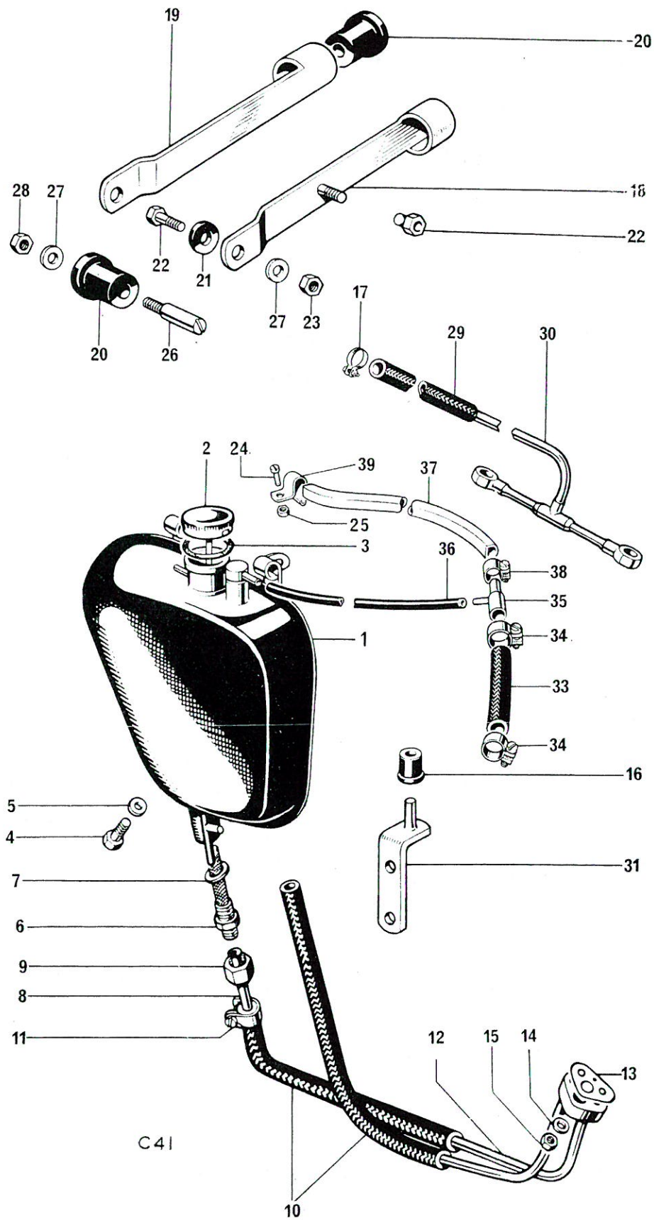
Fig. 26. OIL TANK
