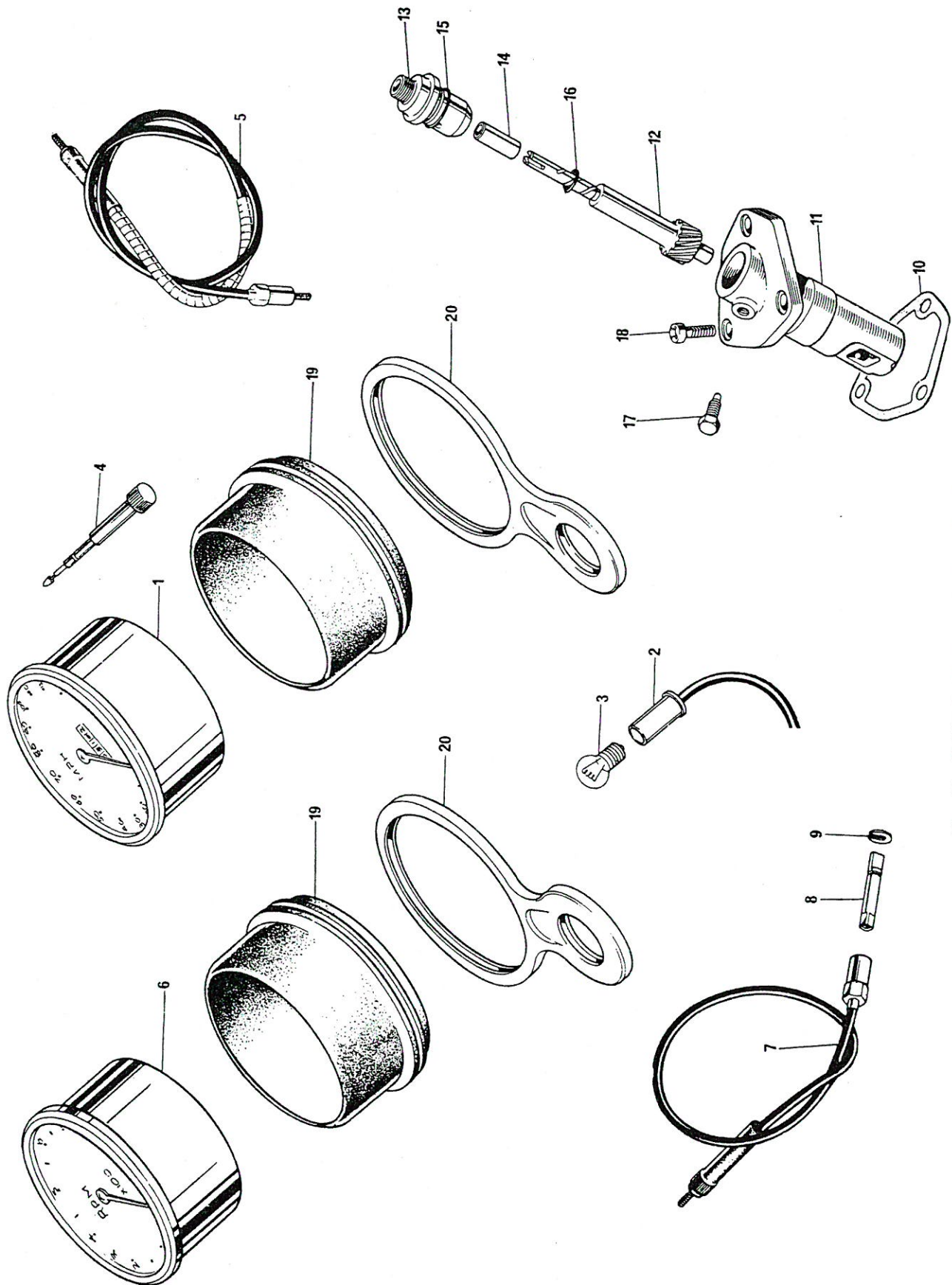
Fig. 33. SPEEDOMETER AND TACHOMETER
