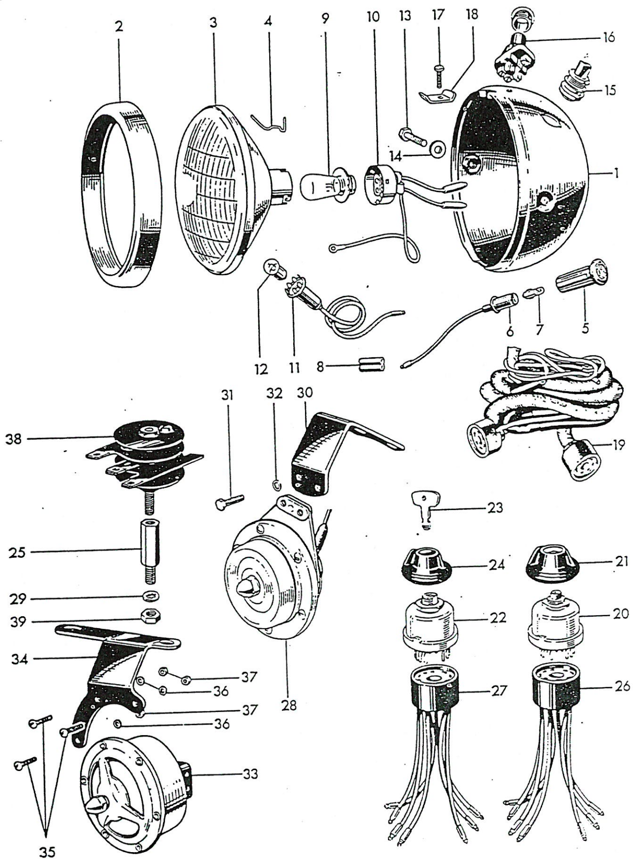
Fig. 19. ELECTRICAL EQUIPMENT
