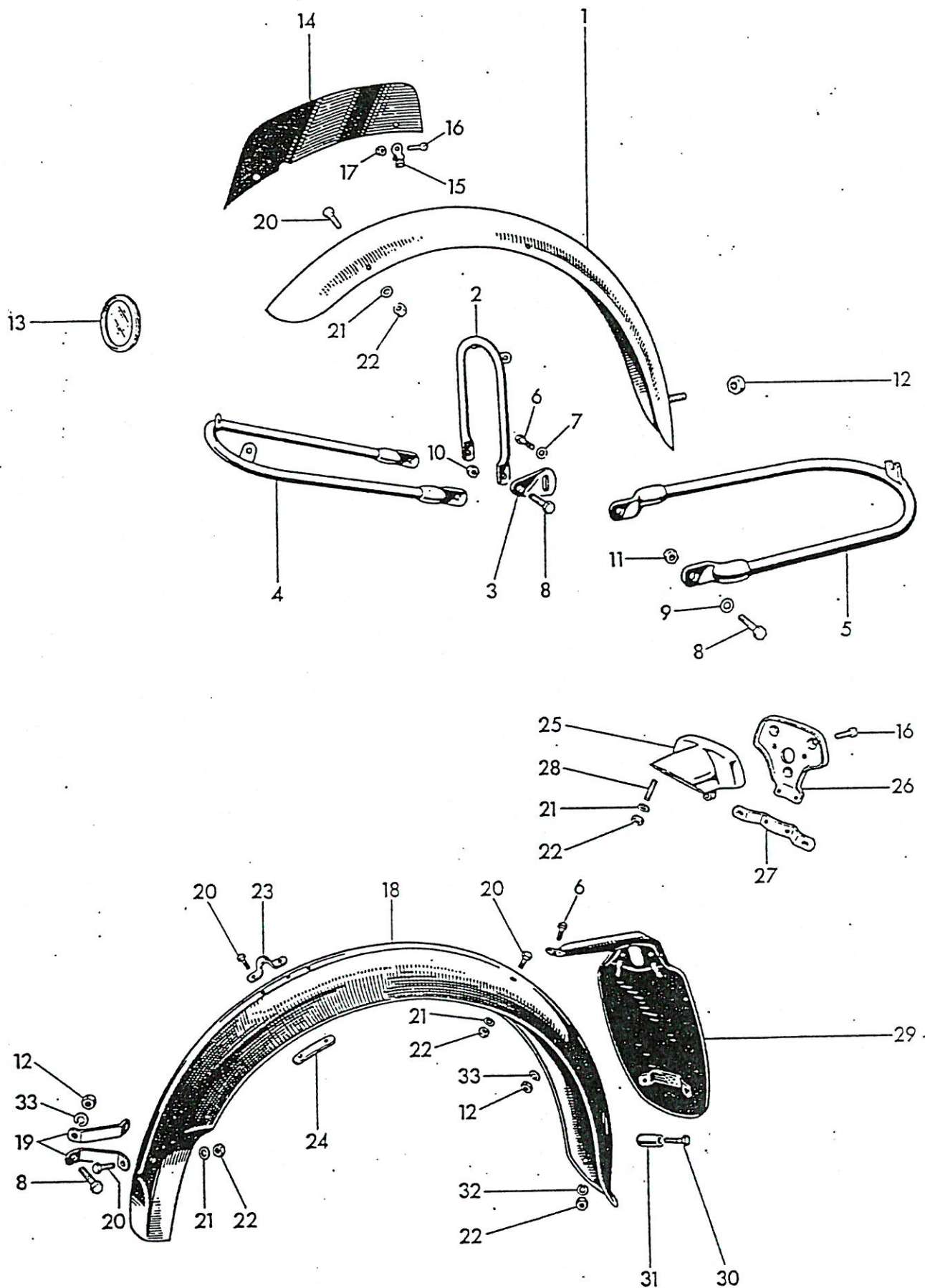
Fig. 12. MUDGUARDS AND NUMBER PLATES
