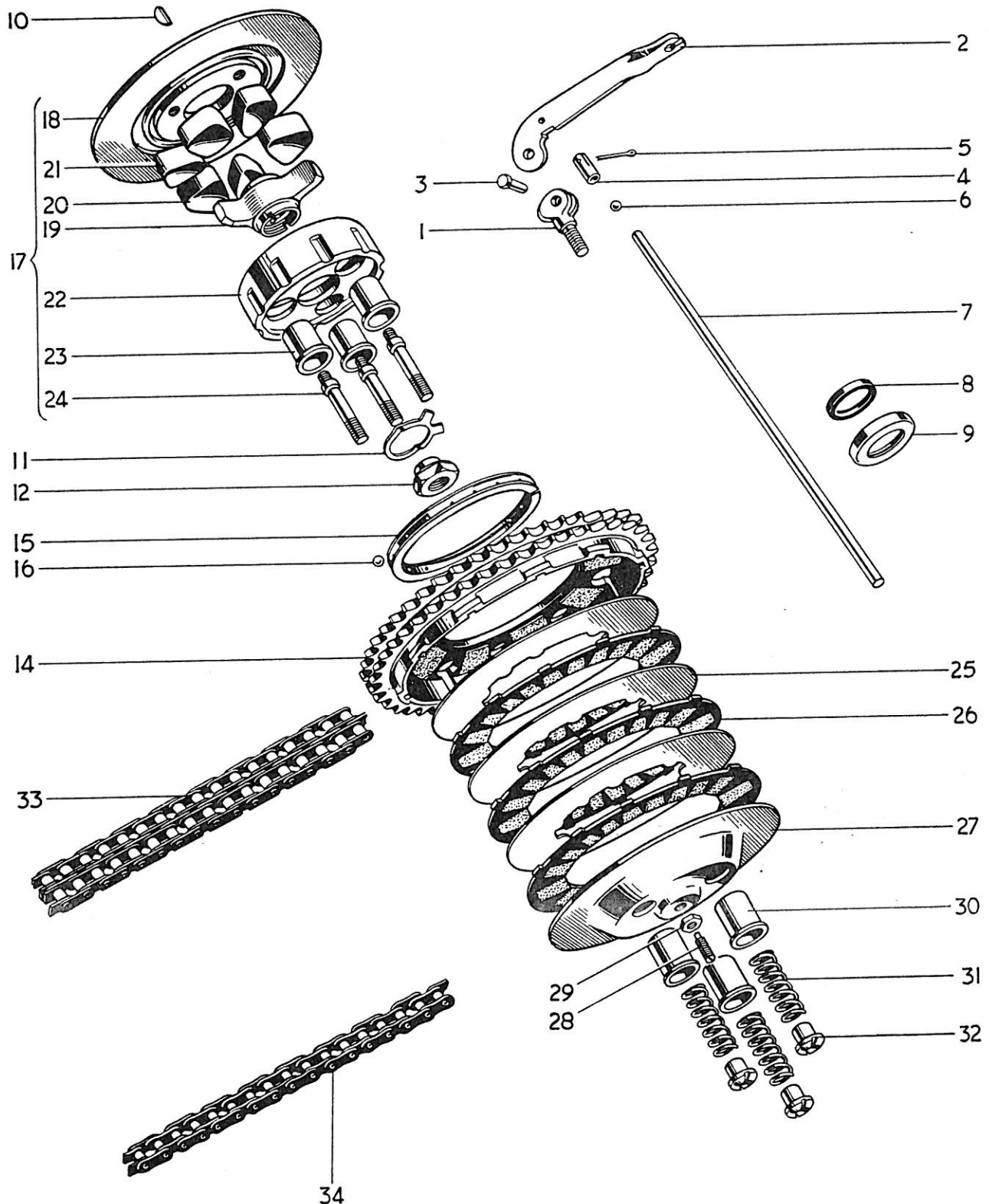
Fig. 7. CLUTCH AND CHAINS
