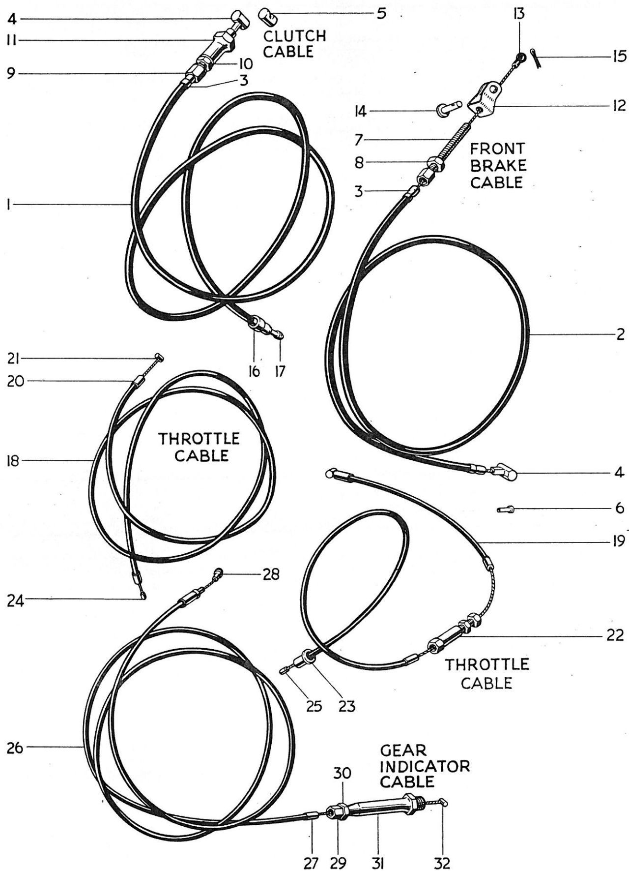
Fig. 22. CONTROL CABLES.
