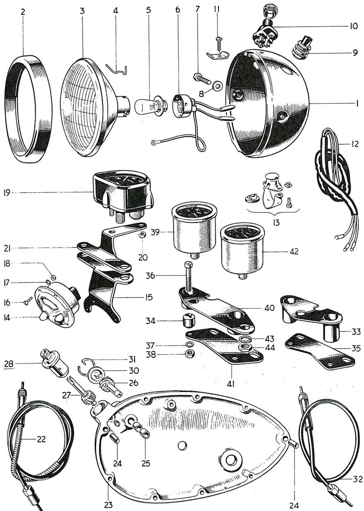
Fig. 13. T20SL HEADLAMP, TACHOMETER, Etc.
