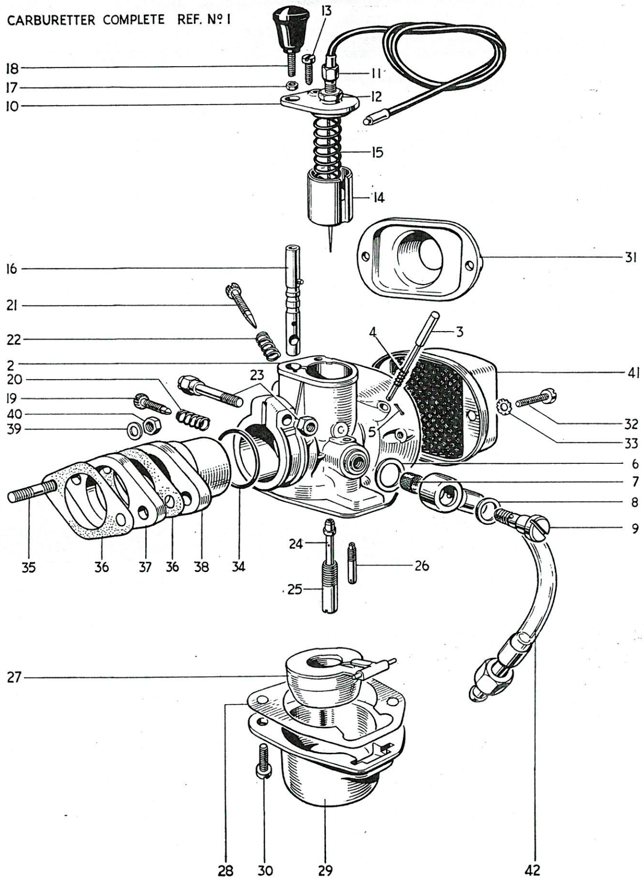
Fig. 24. ZENITH CARBURETTER.
