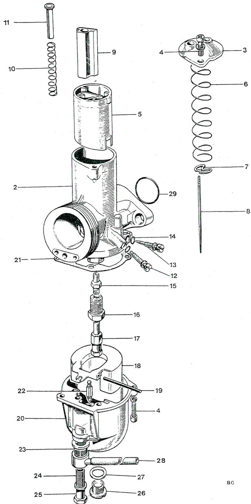
Fig. 8. AMAL CARBURETOR, TR6R, TR6C
