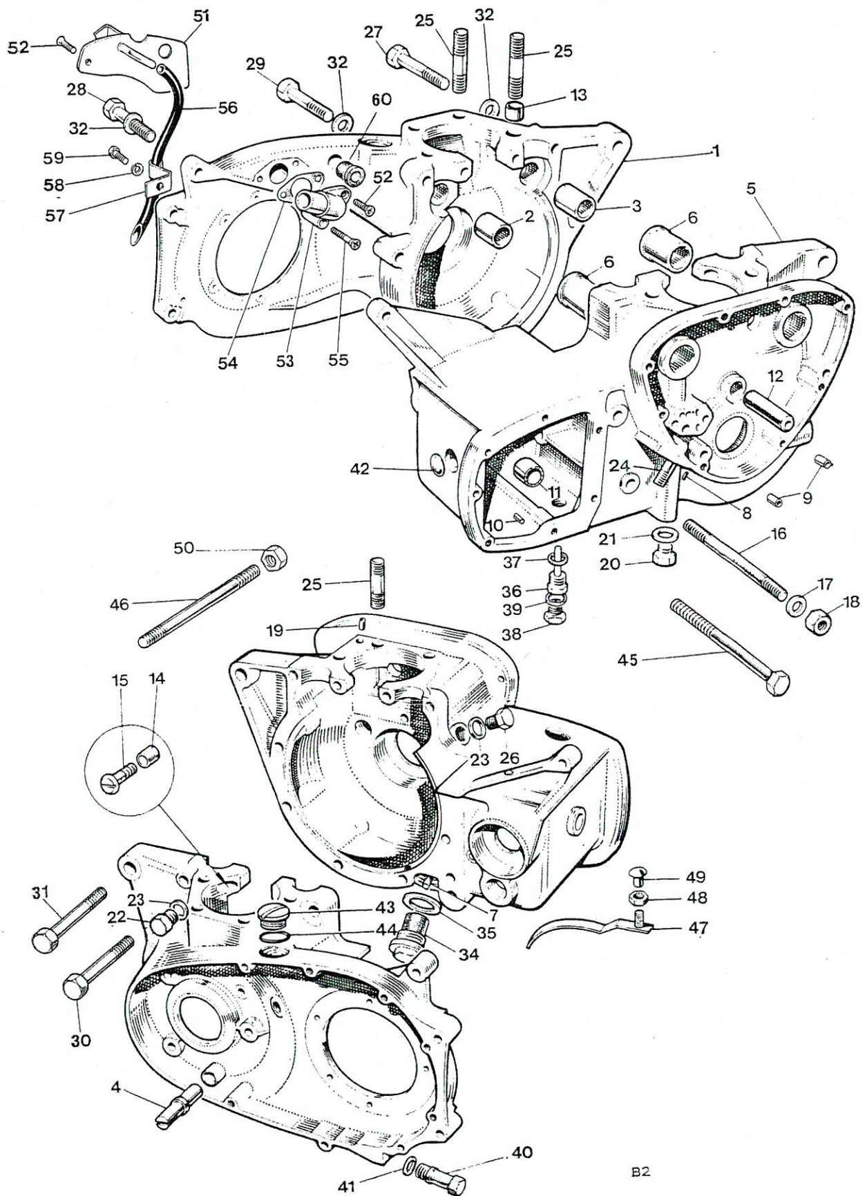
Fig. 2 CRANKCASE
