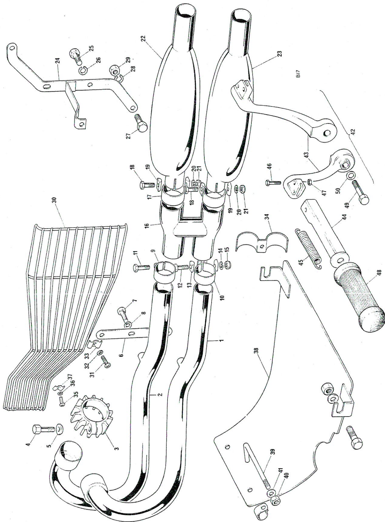
Fig. 21. EXHAUST PIPES AND MUFFLERS, TR6C
