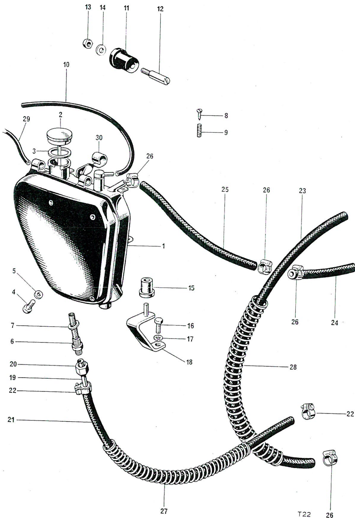
Fig. 24. OIL TANK
