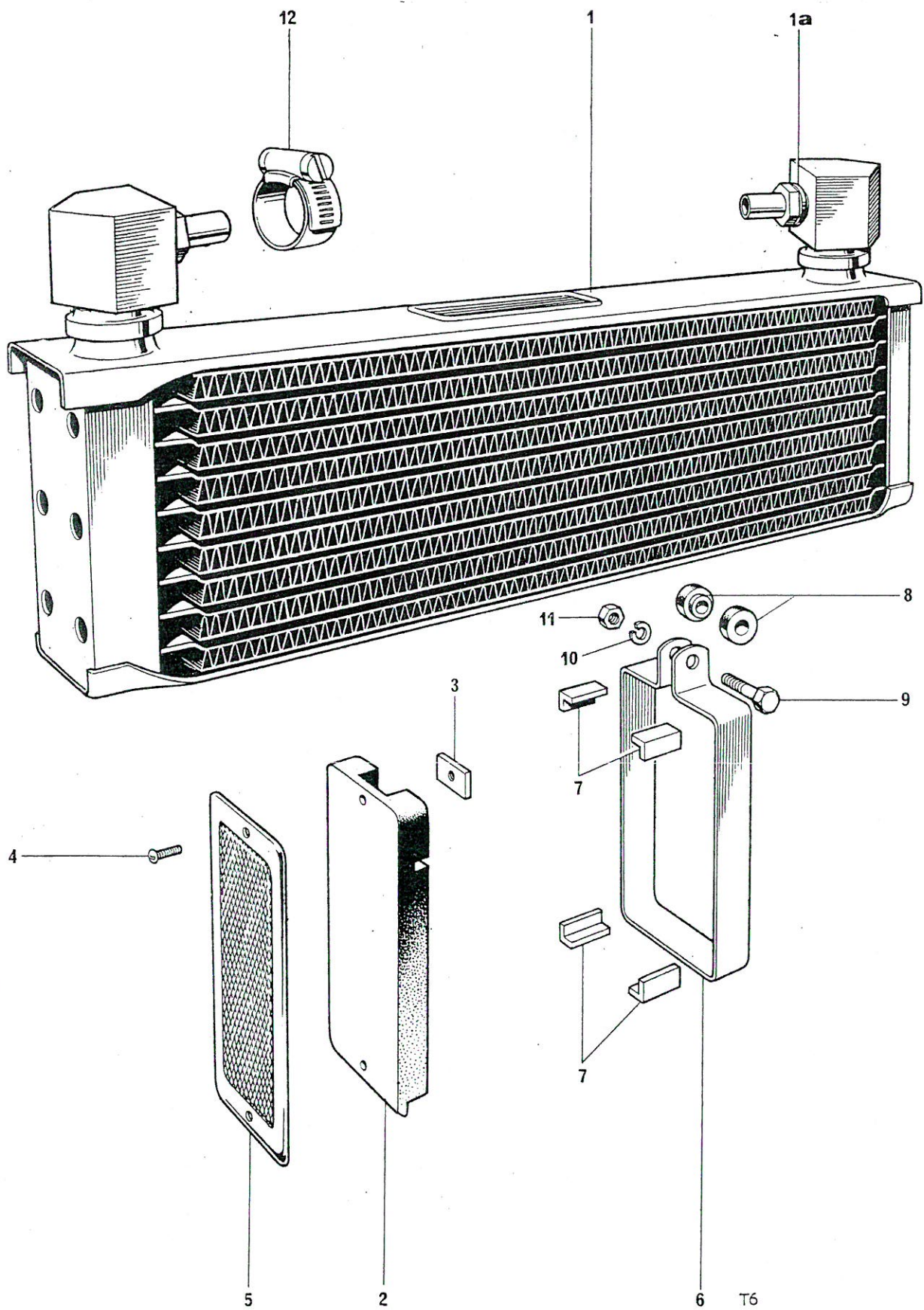
Fig. 22. OIL COOLER
