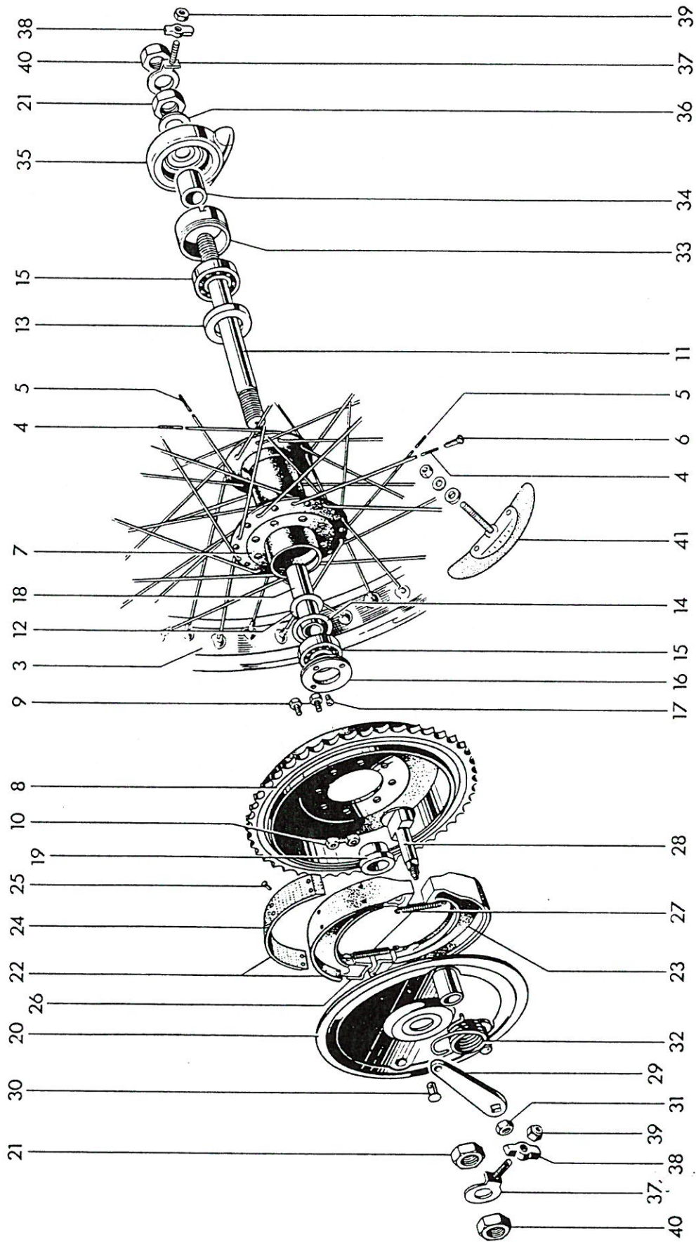
Fig. 18. REAR WHEEL
