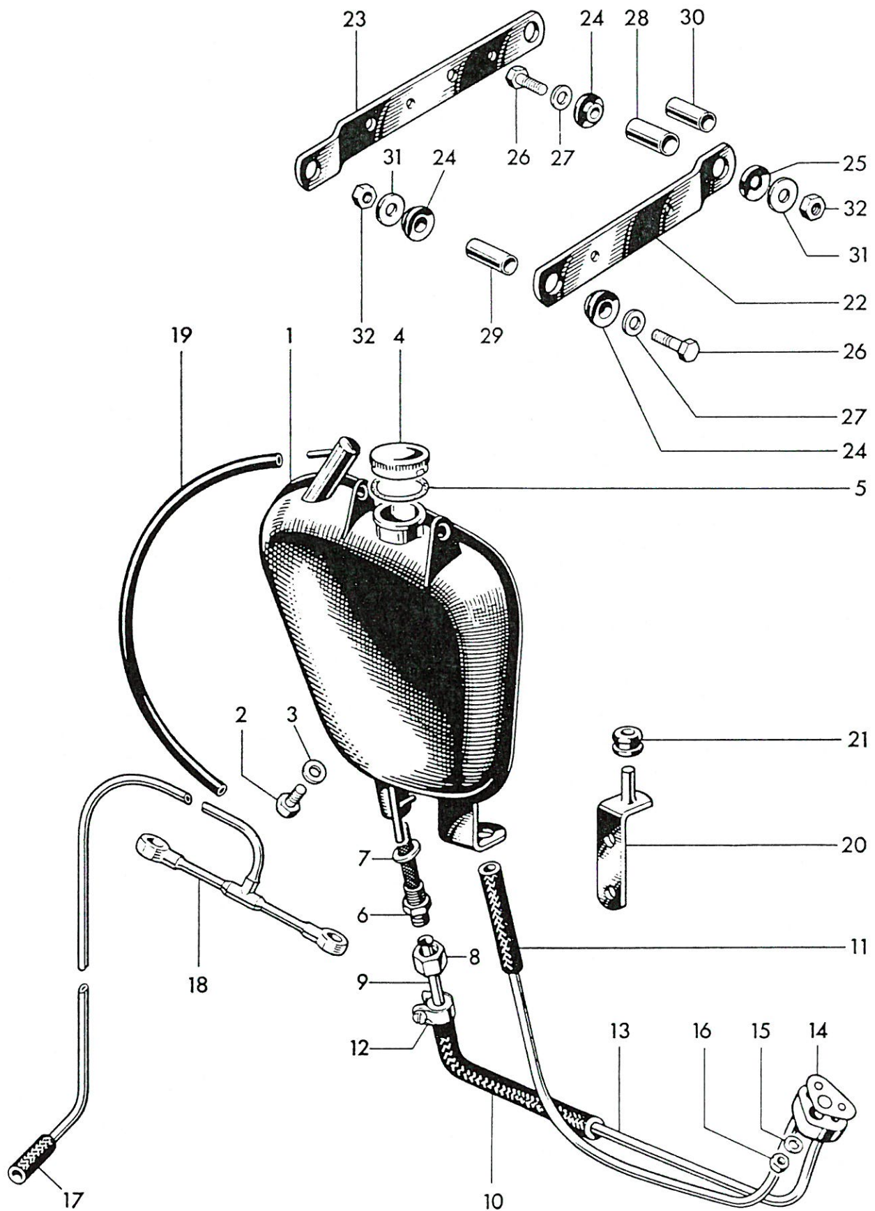
Fig. 23. OIL TANK
