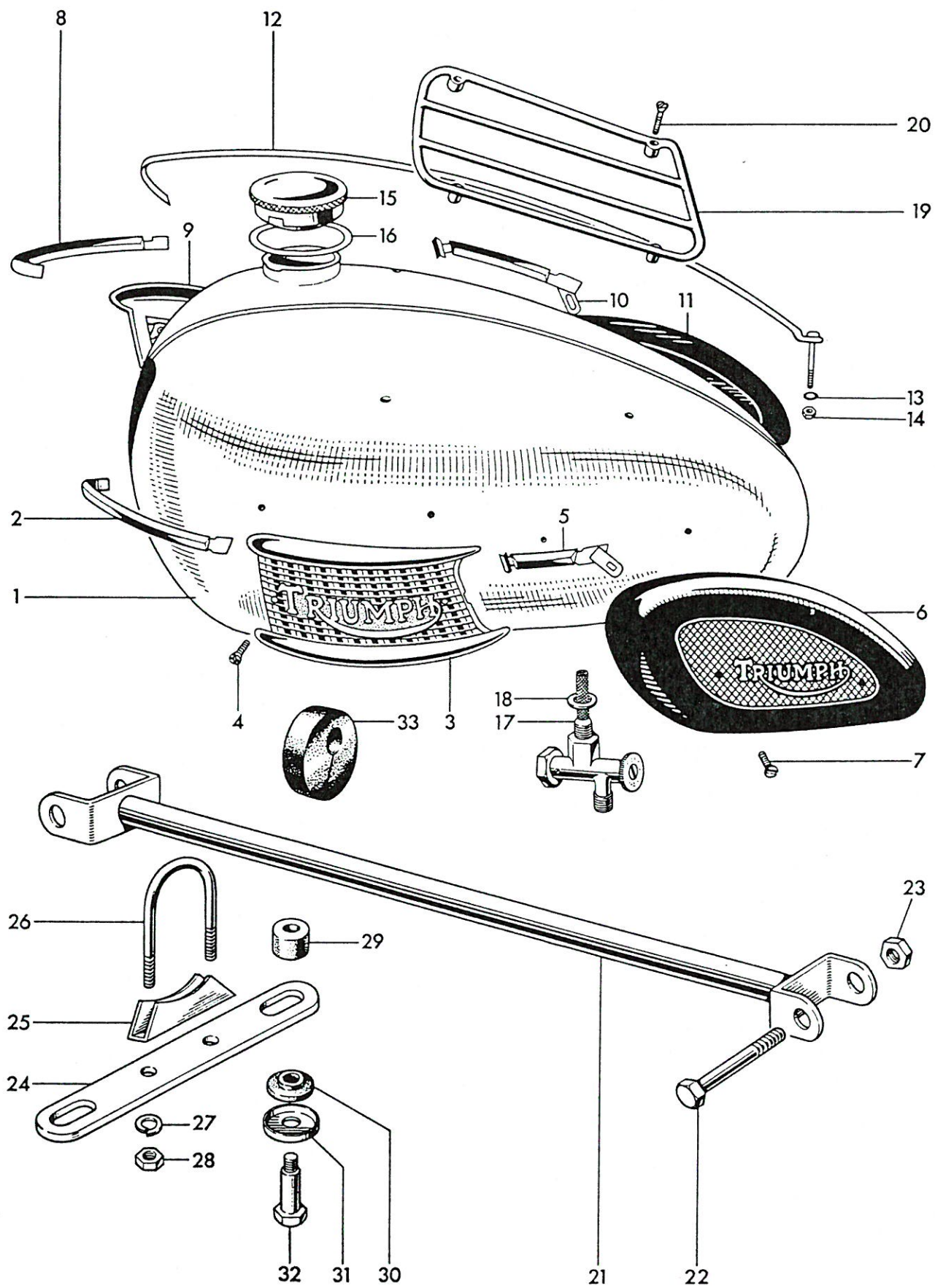
Fig. 22. PETROL TANK
