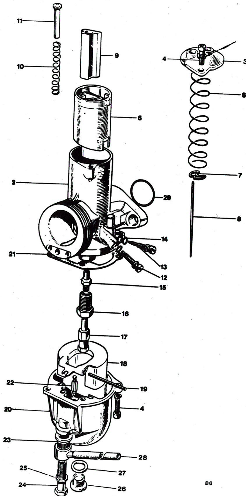
Fig. 8. AMAL CARBURETOR, TR7RV
