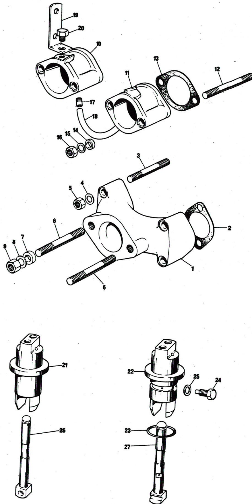
Fig. 4. MANIFOLD AND TAPPETS
