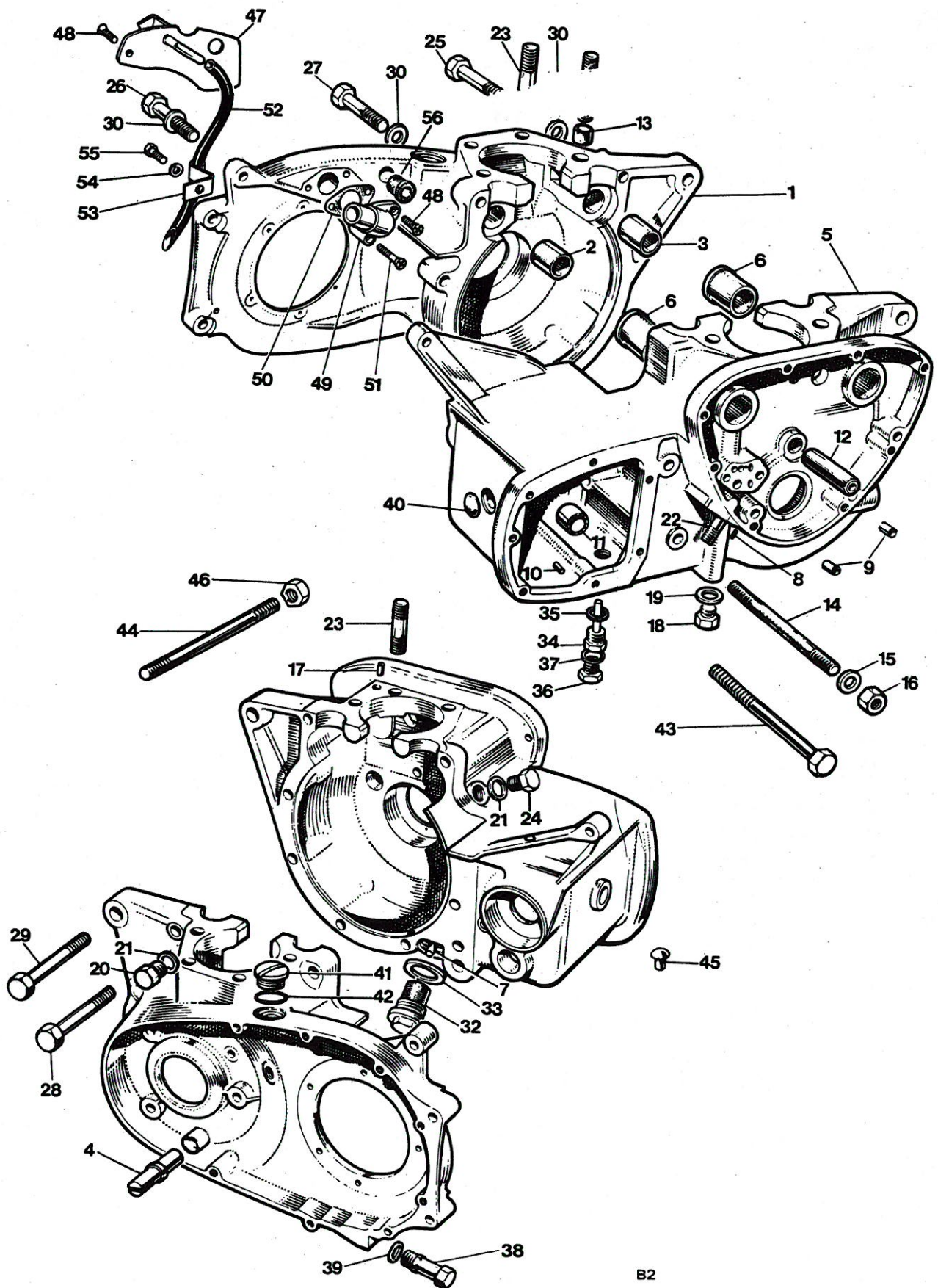
Fig. 2 CRANKCASE
