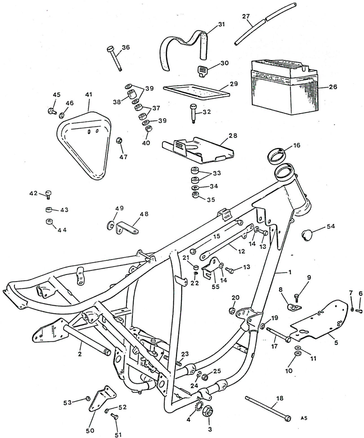
Fig. 5. FRAME COMPLETE
