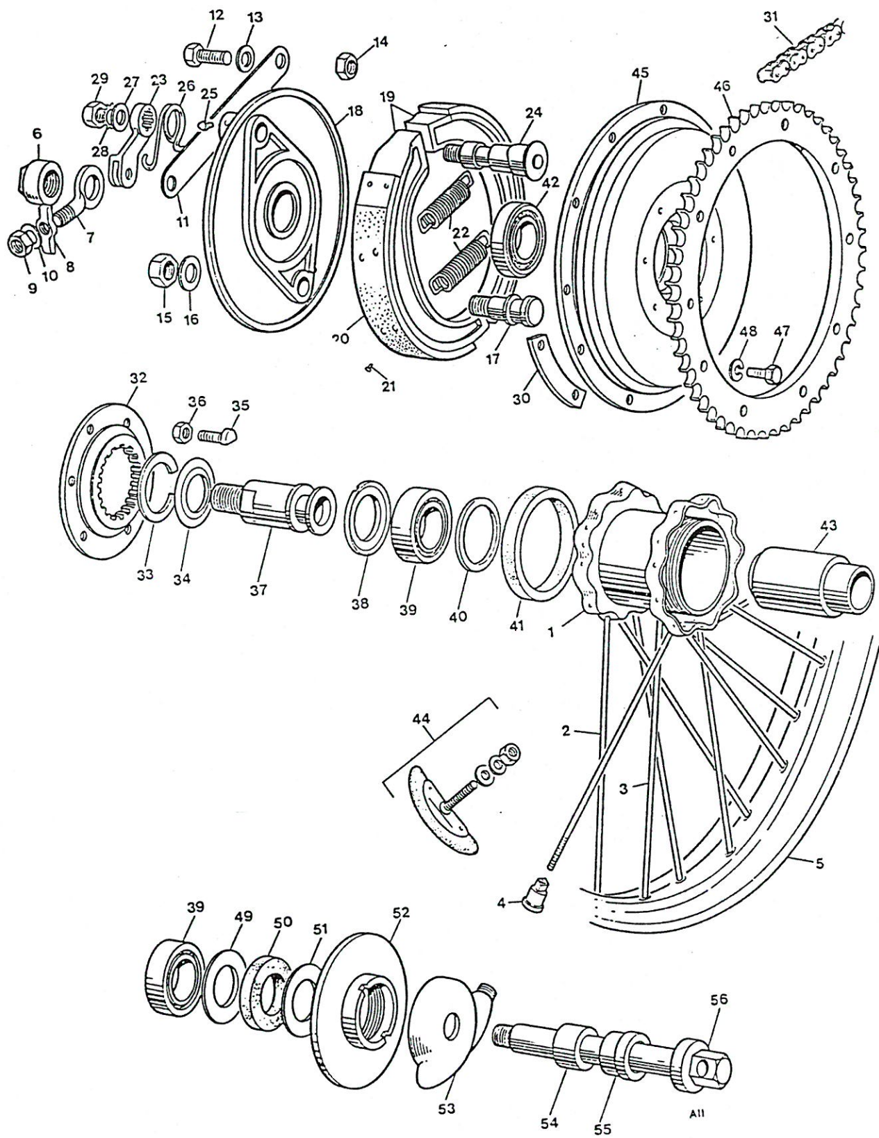
Fig. 11. REAR WHEEL
