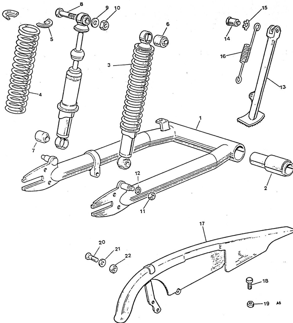
Fig. 6. SWINGING ARM AND SUSPENSION UNITS
