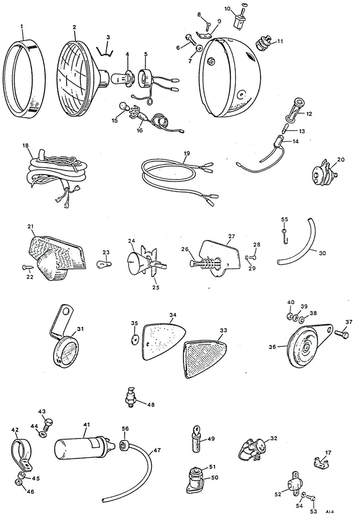
Fig. 16. ELECTRICAL EQUIPMENT
