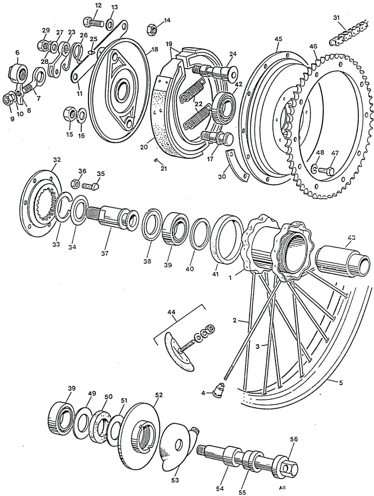
Fig. 11. REAR WHEEL
