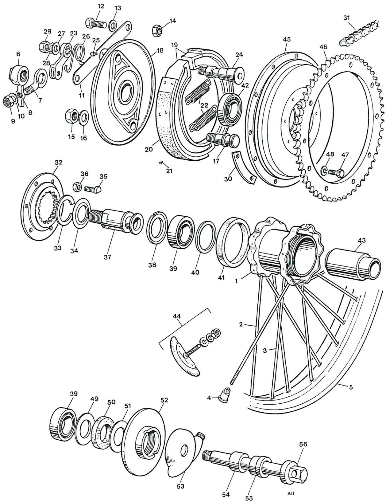
Fig. 11. REAR WHEEL
