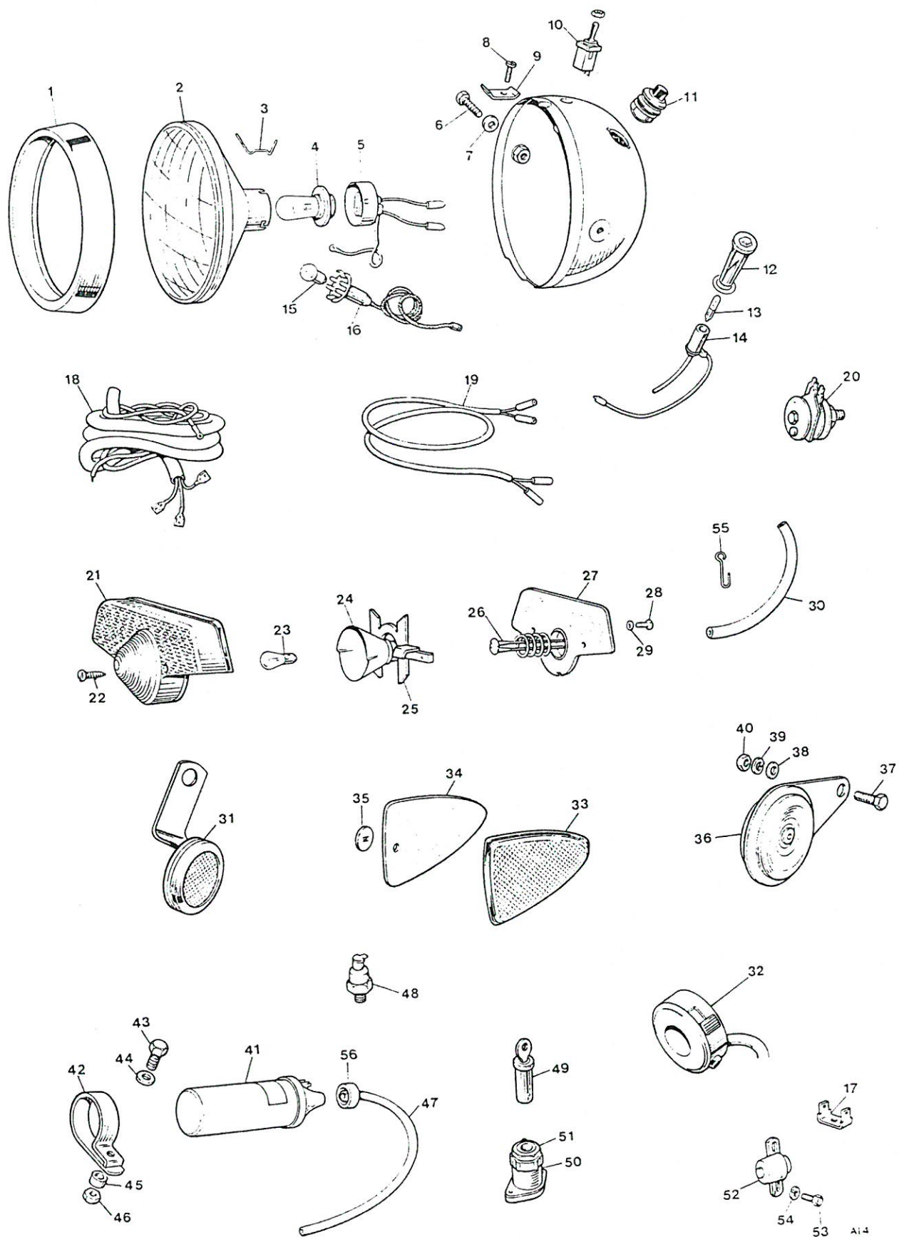
Fig. 16. ELECTRICAL EQUIPMENT
