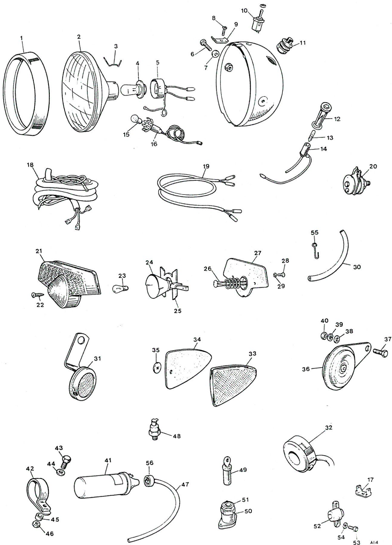
Fig. 16. ELECTRICAL EQUIPMENT
