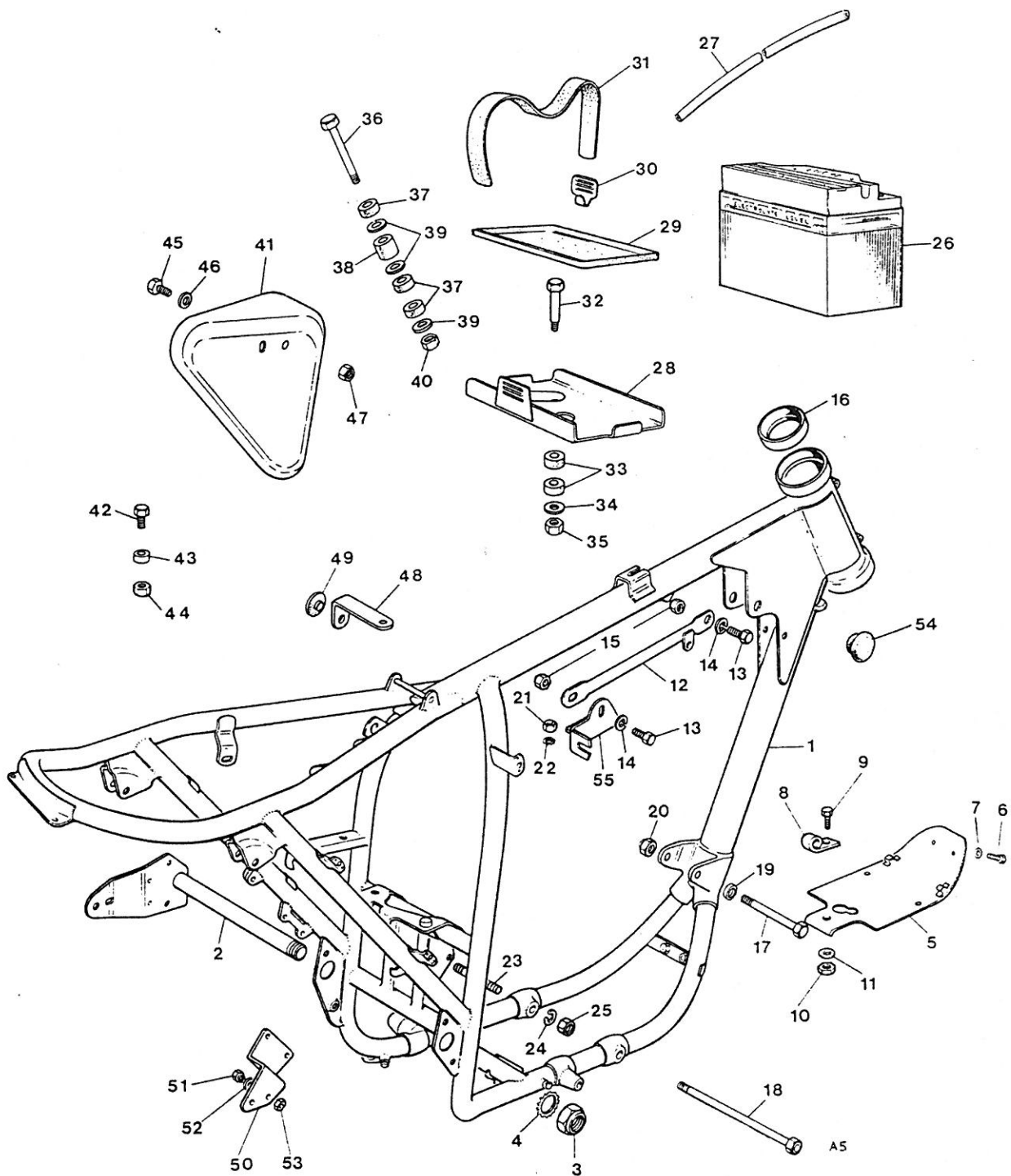
Fig. 5. FRAME COMPLETE
