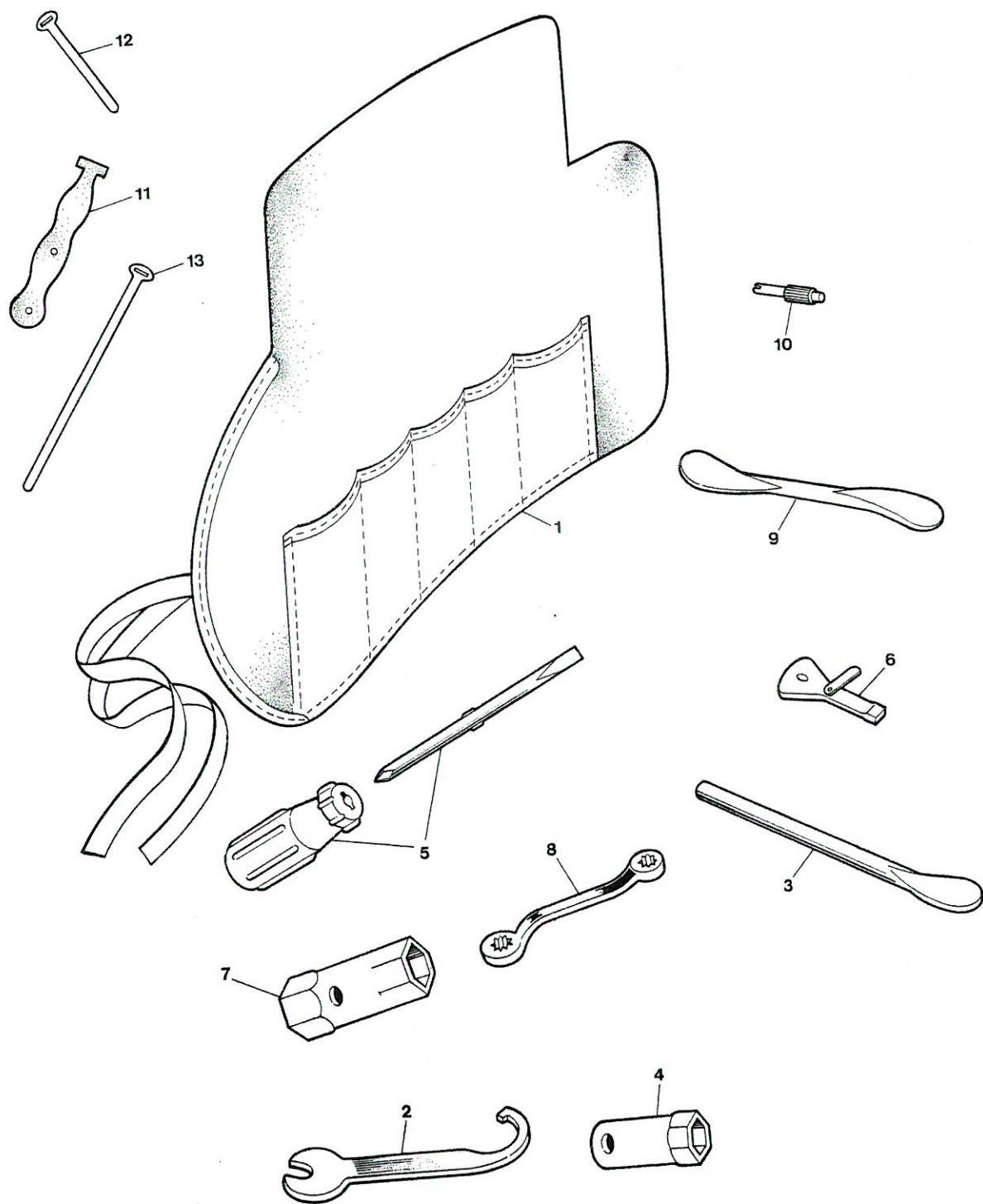
Fig.15 TOOL KIT
