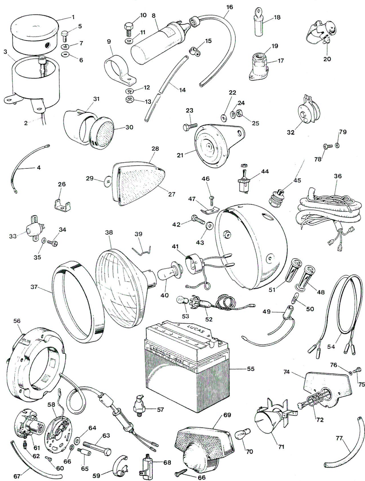
Fig.14 ELECTRICAL EQUIPMENT
