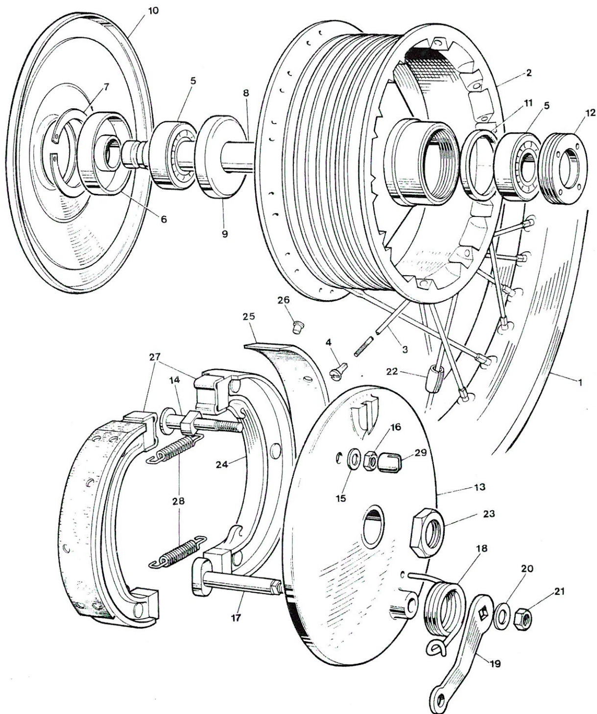
Fig.10 FRONT WHEEL
