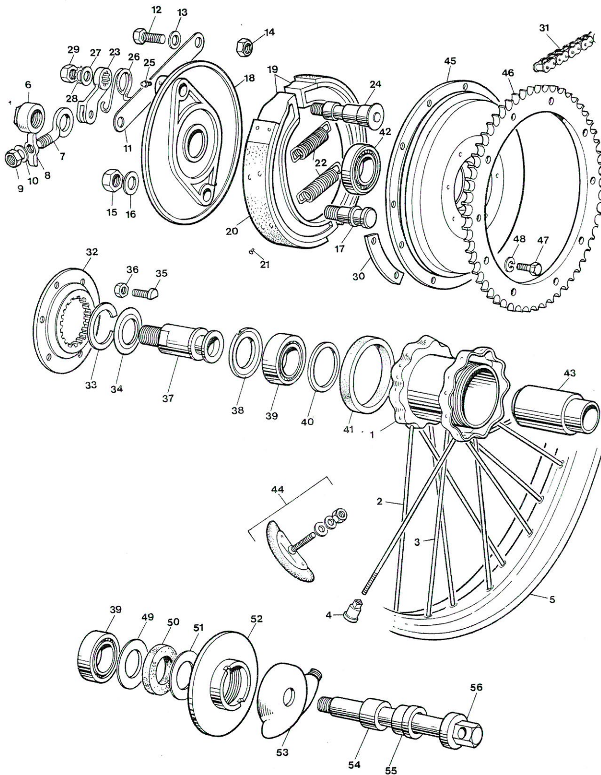
Fig.11 REAR WHEEL
