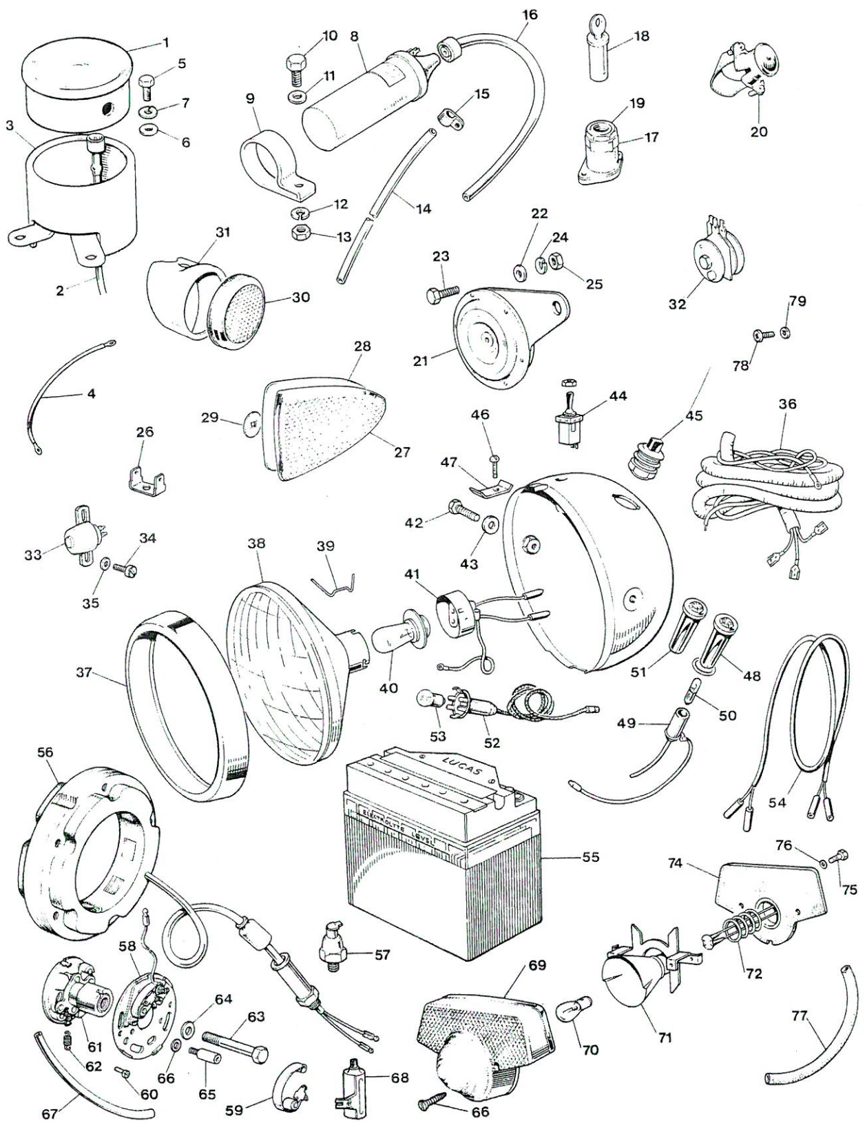
Fig.14 ELECTRICAL EQUIPMENT
