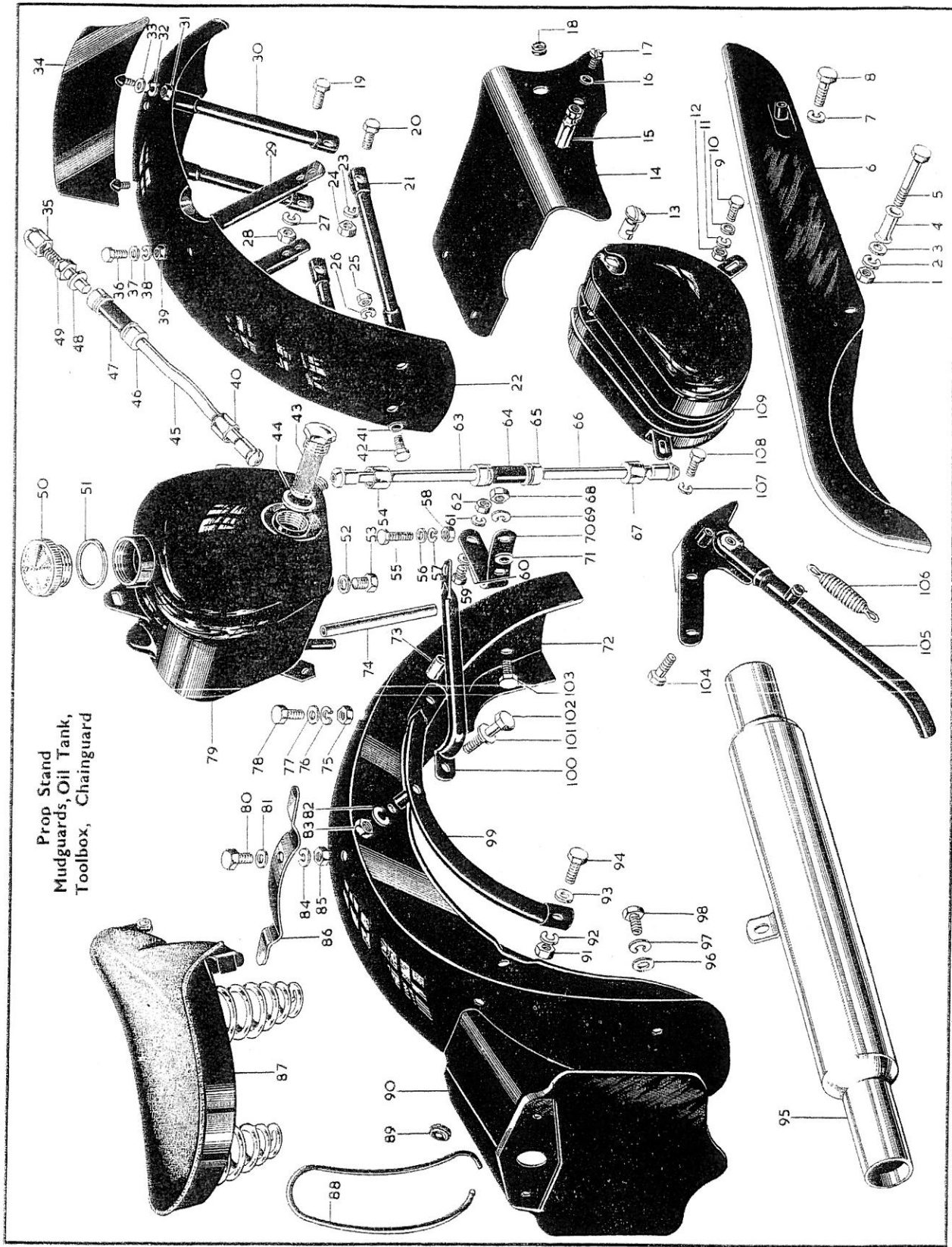
Plate 27 Prop Stand, Mudguards, Oil Tank, Toolbox and Chainguard
