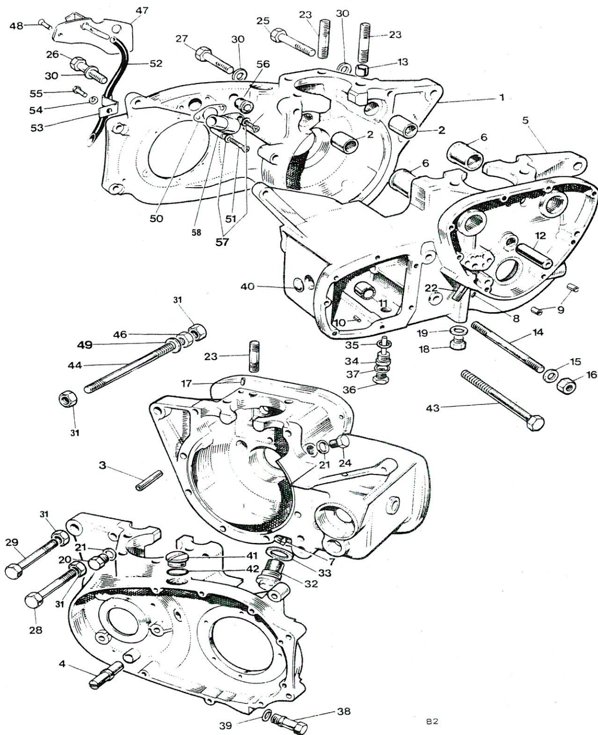
Fig. 2 CRANKCASE
