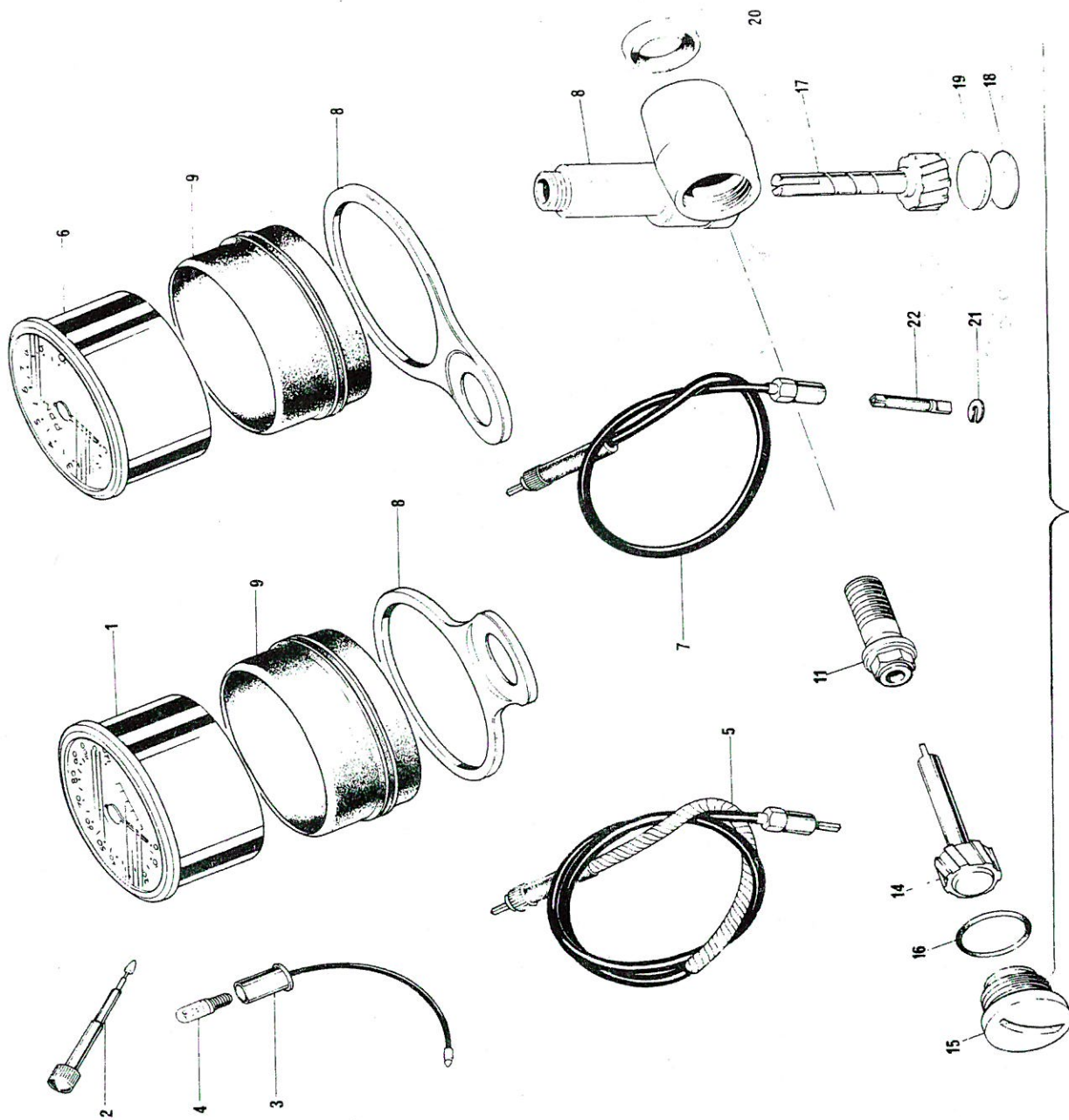
10 TACHOMETER GEARBL. COMPLETE Fig. 32. SPEEDOMETER AND TACHOMETER
