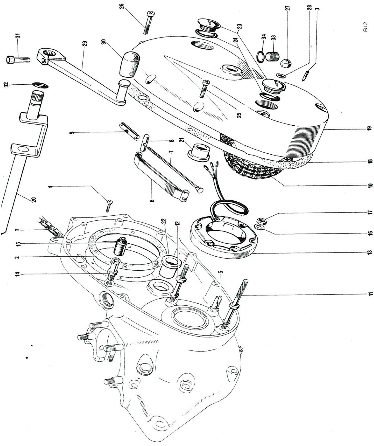
Fig. 15. CHAINCASE AND CHAINS
