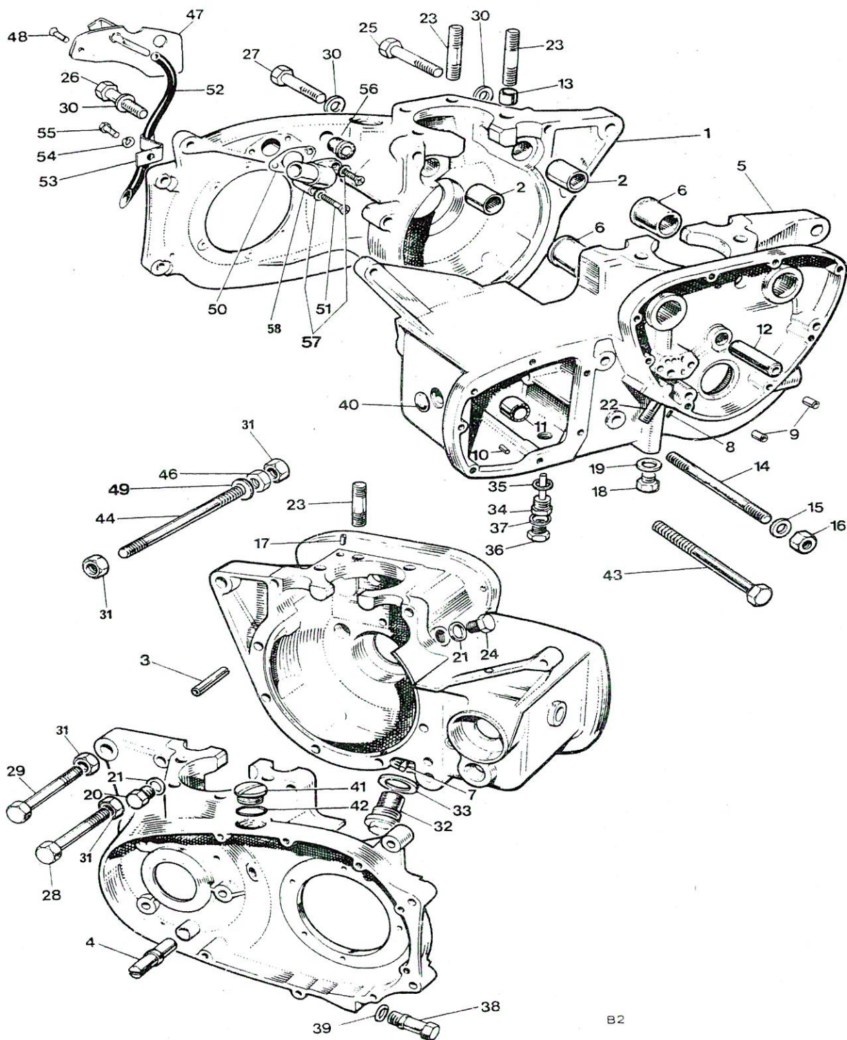
Fig. 2 CRANKCASE
