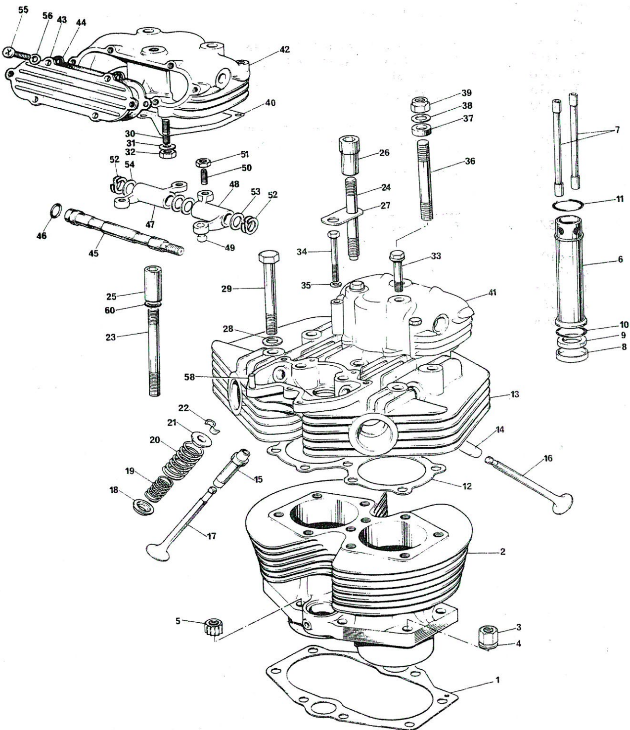
CYLINDER BLOCK & HEAD, T140V
