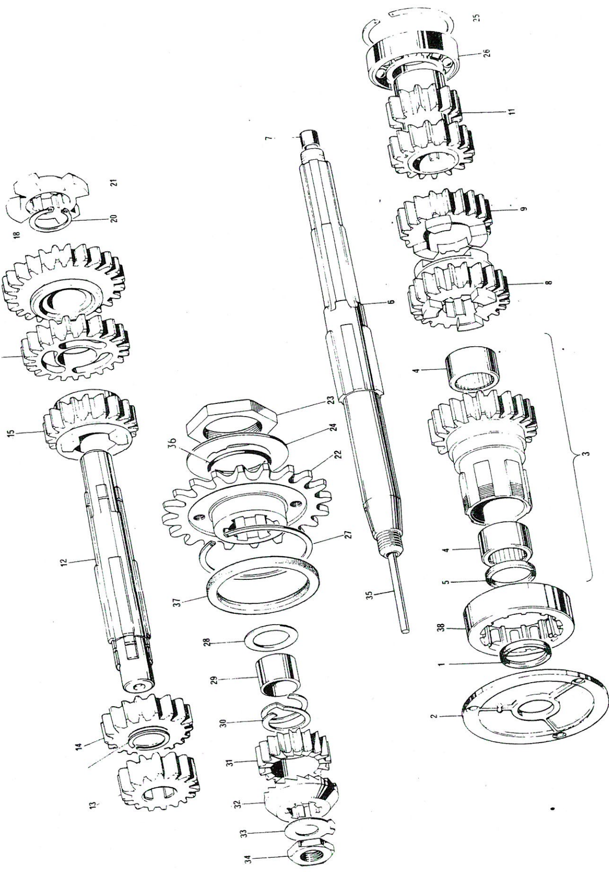
Fig. 12 GEARBOX SHAFTS AND GEARS (5 SPEED)
