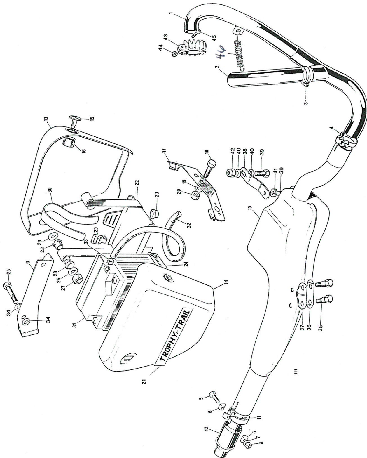
Fig. 13. EXHAUST SYSTEM, SIDE COVERS AND BATTERY
