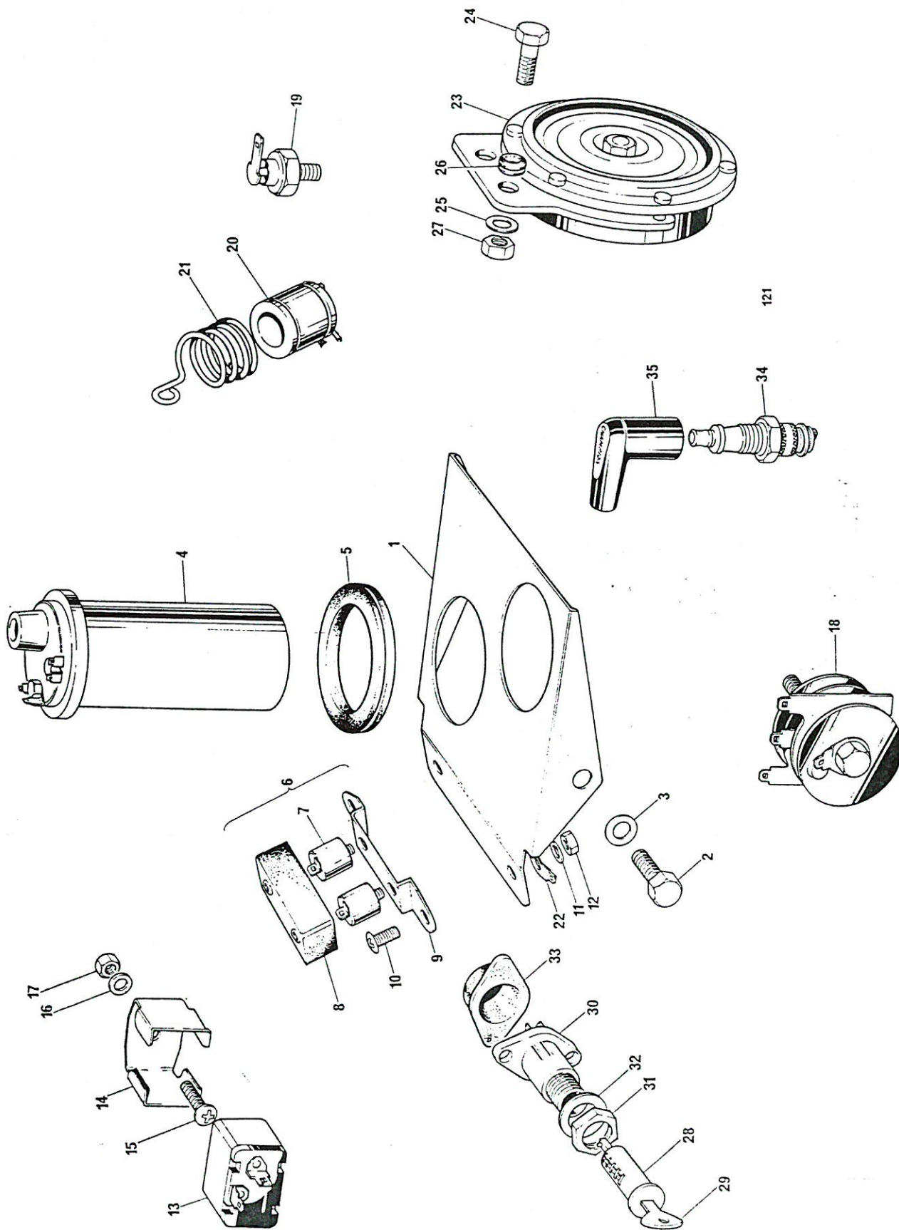
FIG. 23. ELECTRICAL COMPONENTS
