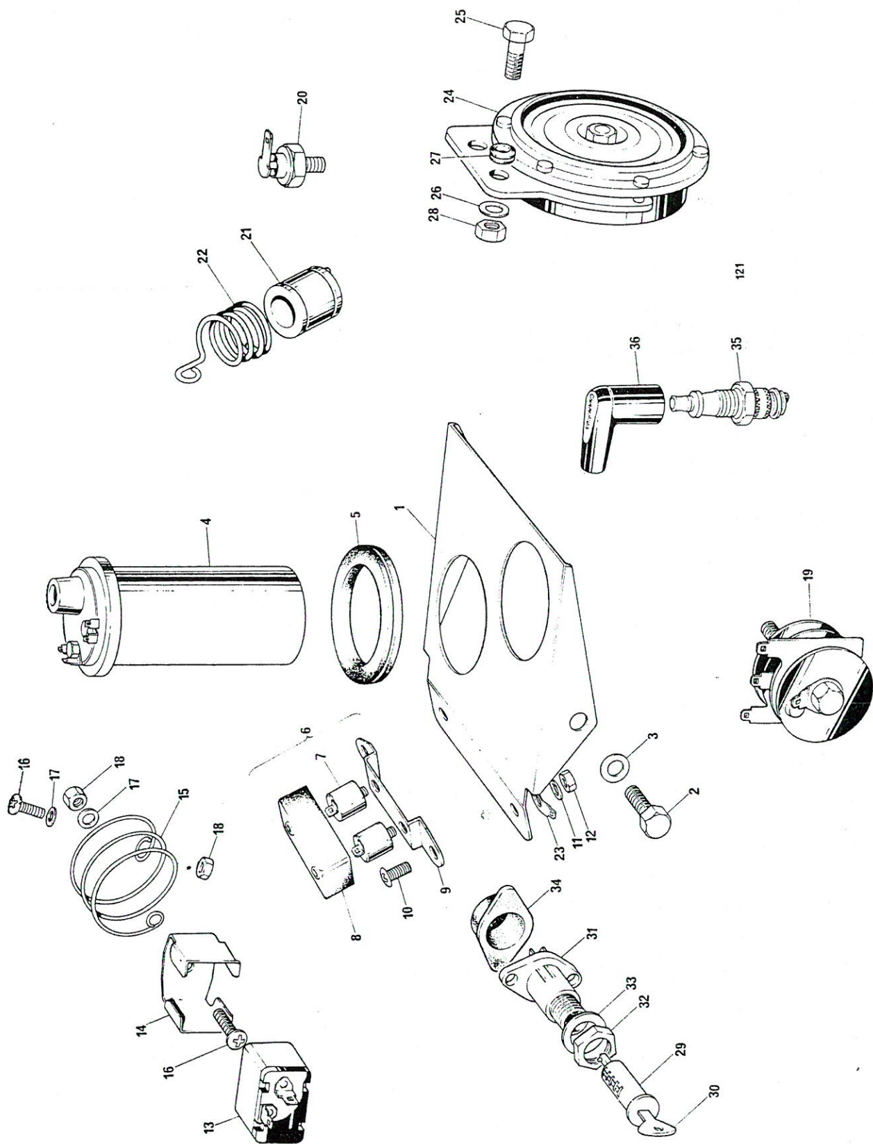
Fig. 22. ELECTRICAL COMPONENTS
