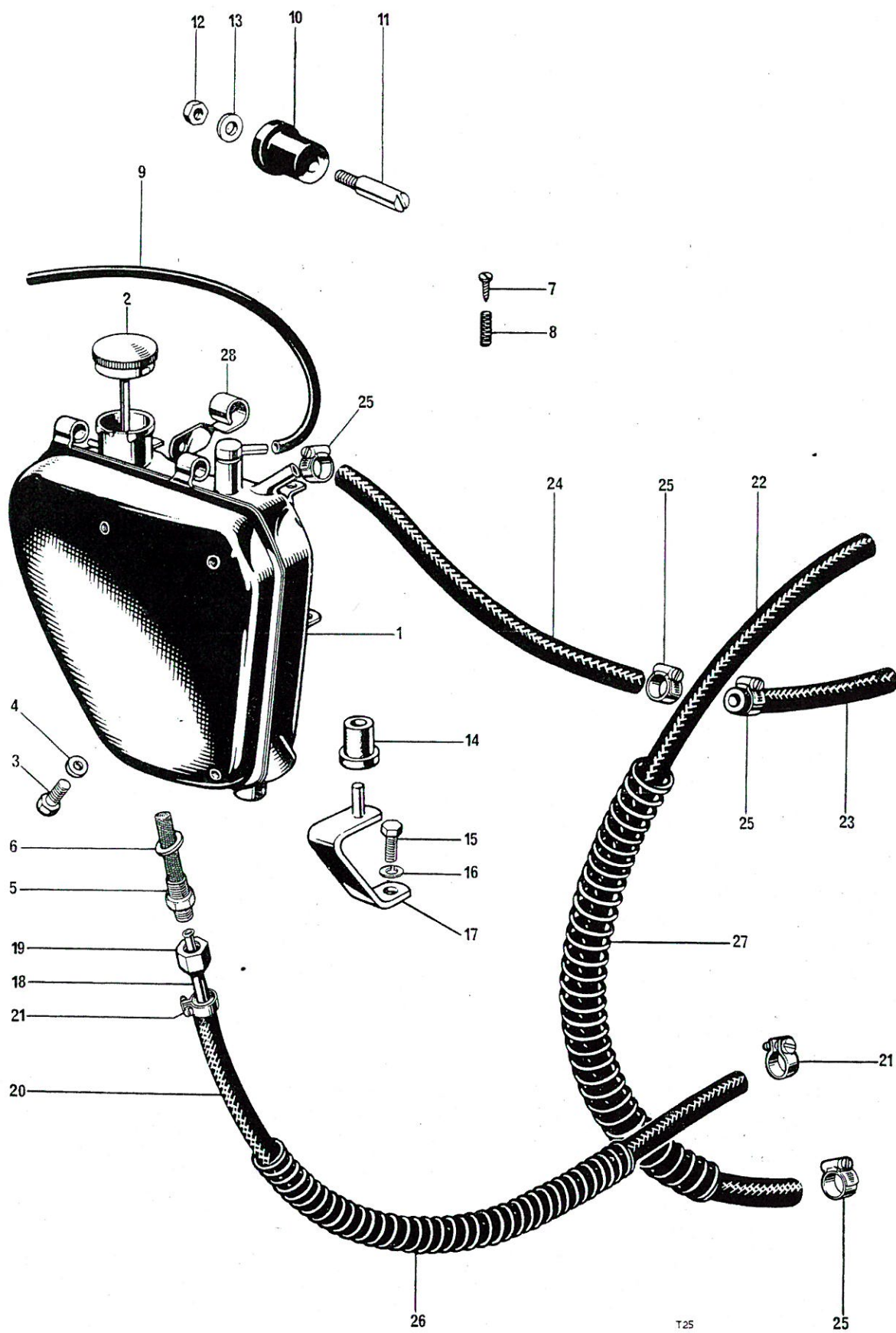
Fig. 25. OIL TANK
