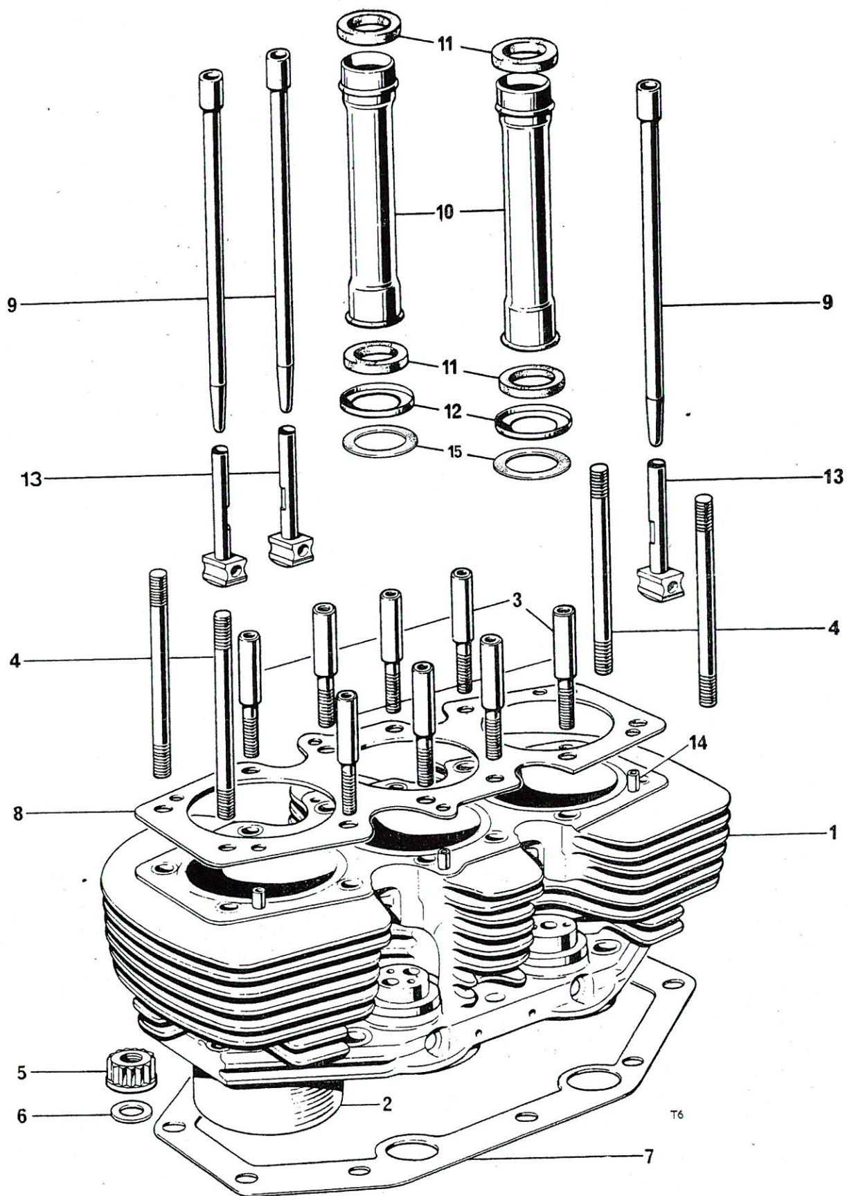
Fig. 6. CYLINDER BARREL, PUSH RODS AND TUBES, TAPPETS
