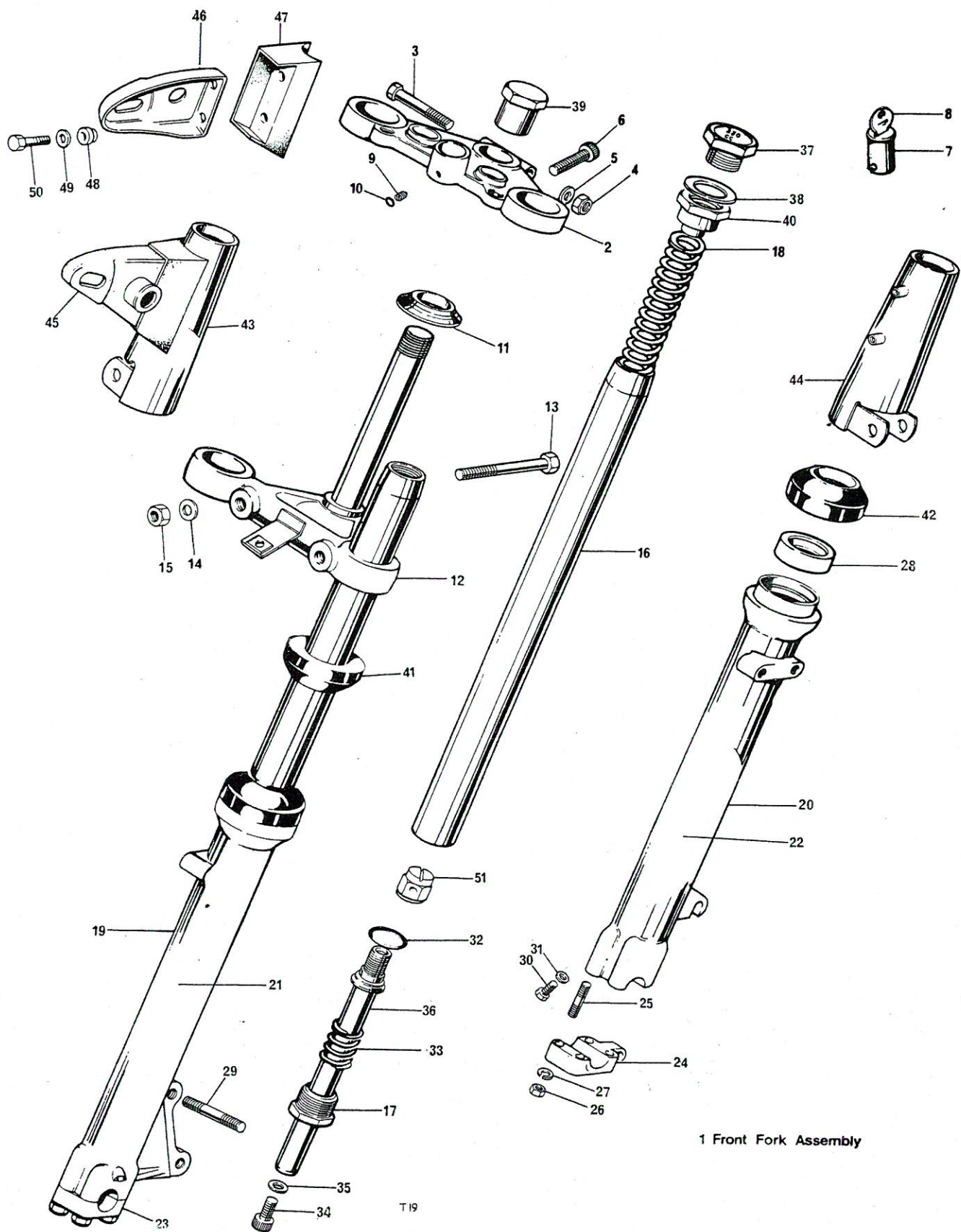
Fig. 19. TELESCOPIC FRONT FORK
