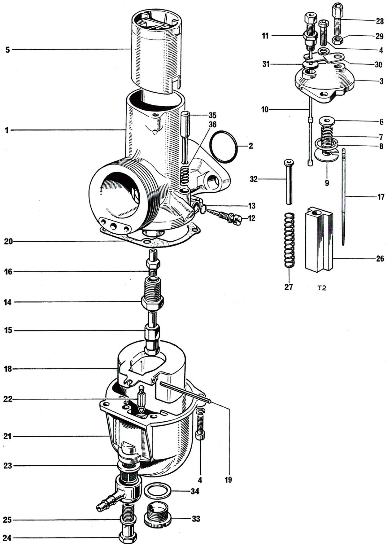
Fig. 5. CARBURETORS
