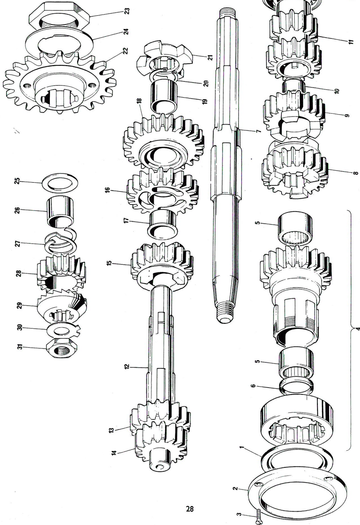
FIG. 11. GEARBOX SHAFTS AND GEARS
