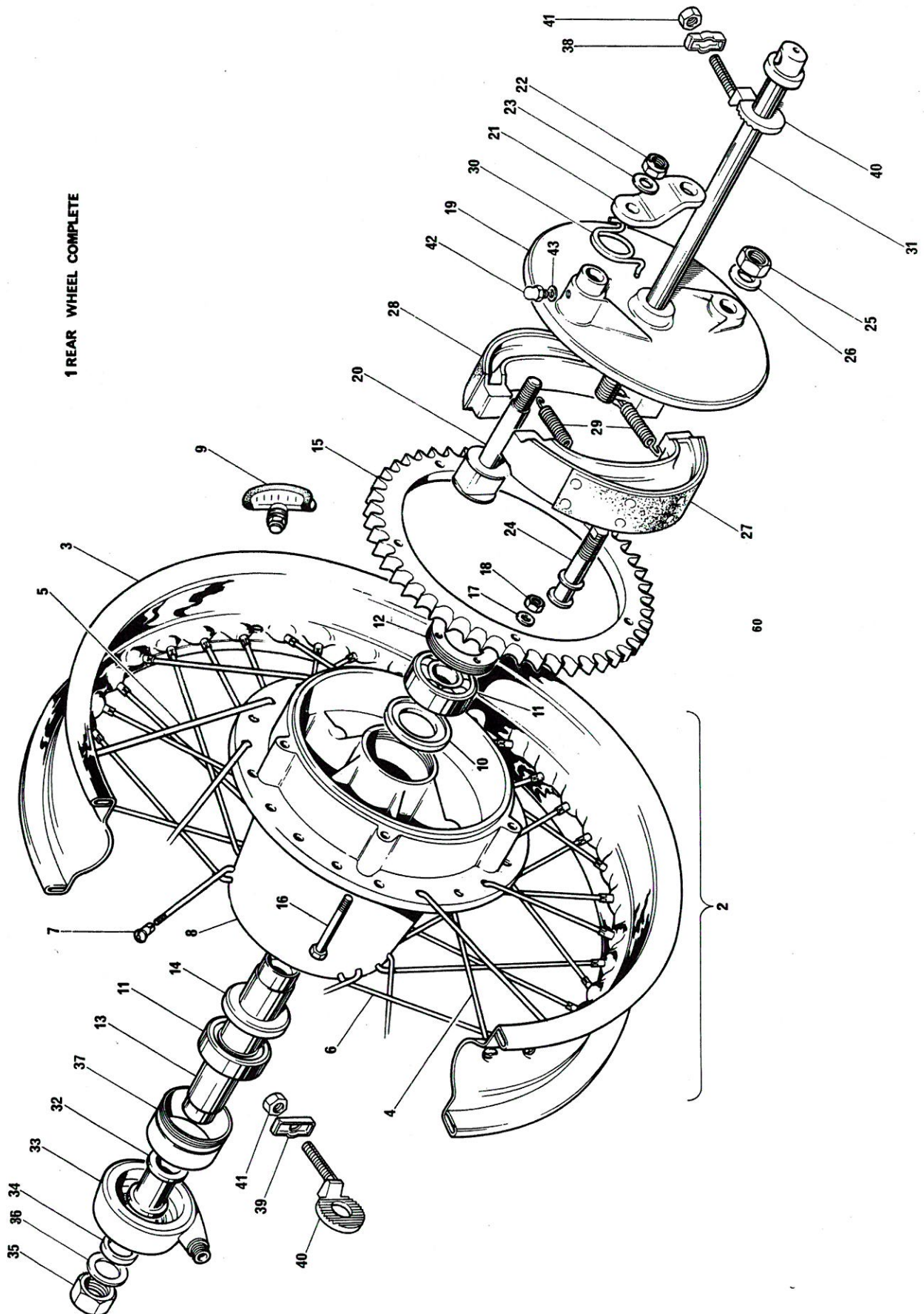
Fig. 22. REAR WHEEL
