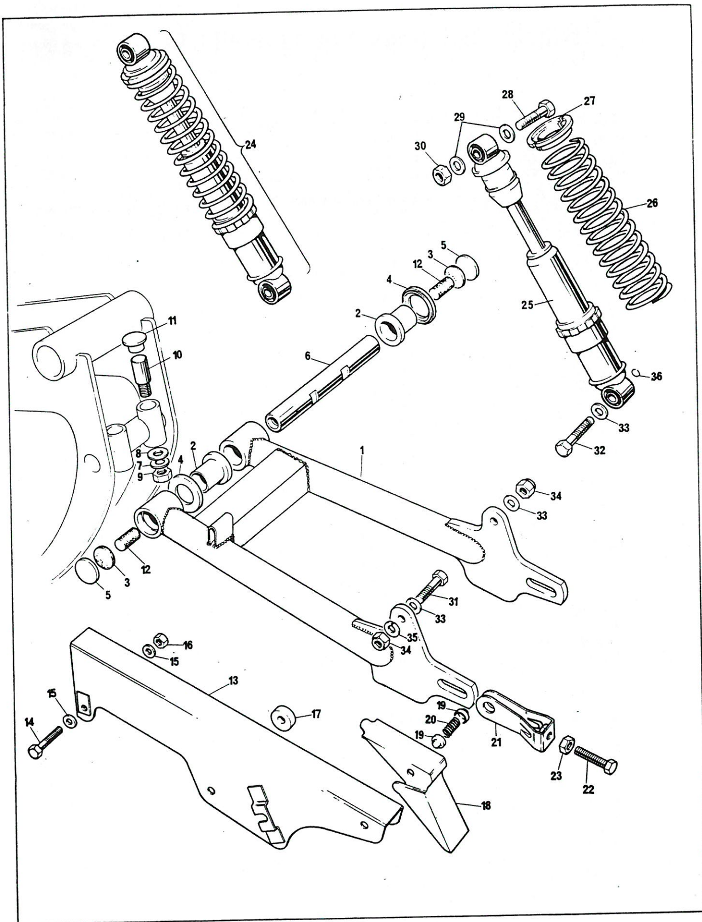
Swinging Arm, Suspension Units, Chainguard
