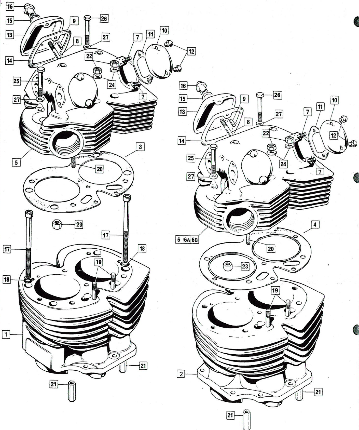
Engine: Cylinder, Cylinder Head 750 and 850
