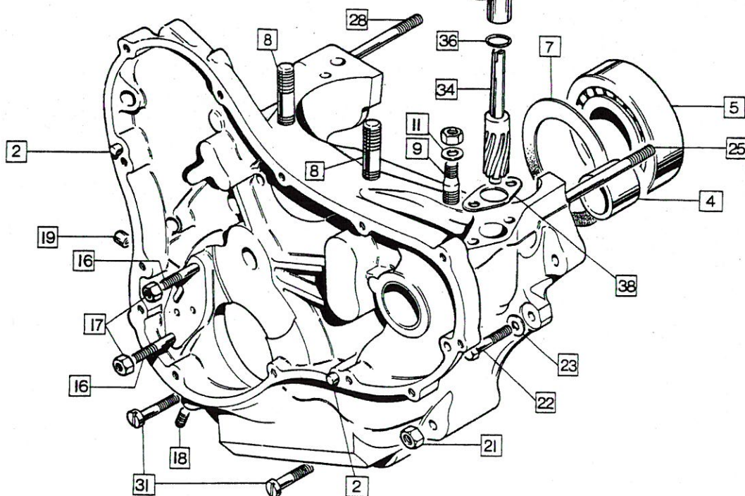
750 Engine: Crankcases, Crankcase Breather, Tachometer Drive
