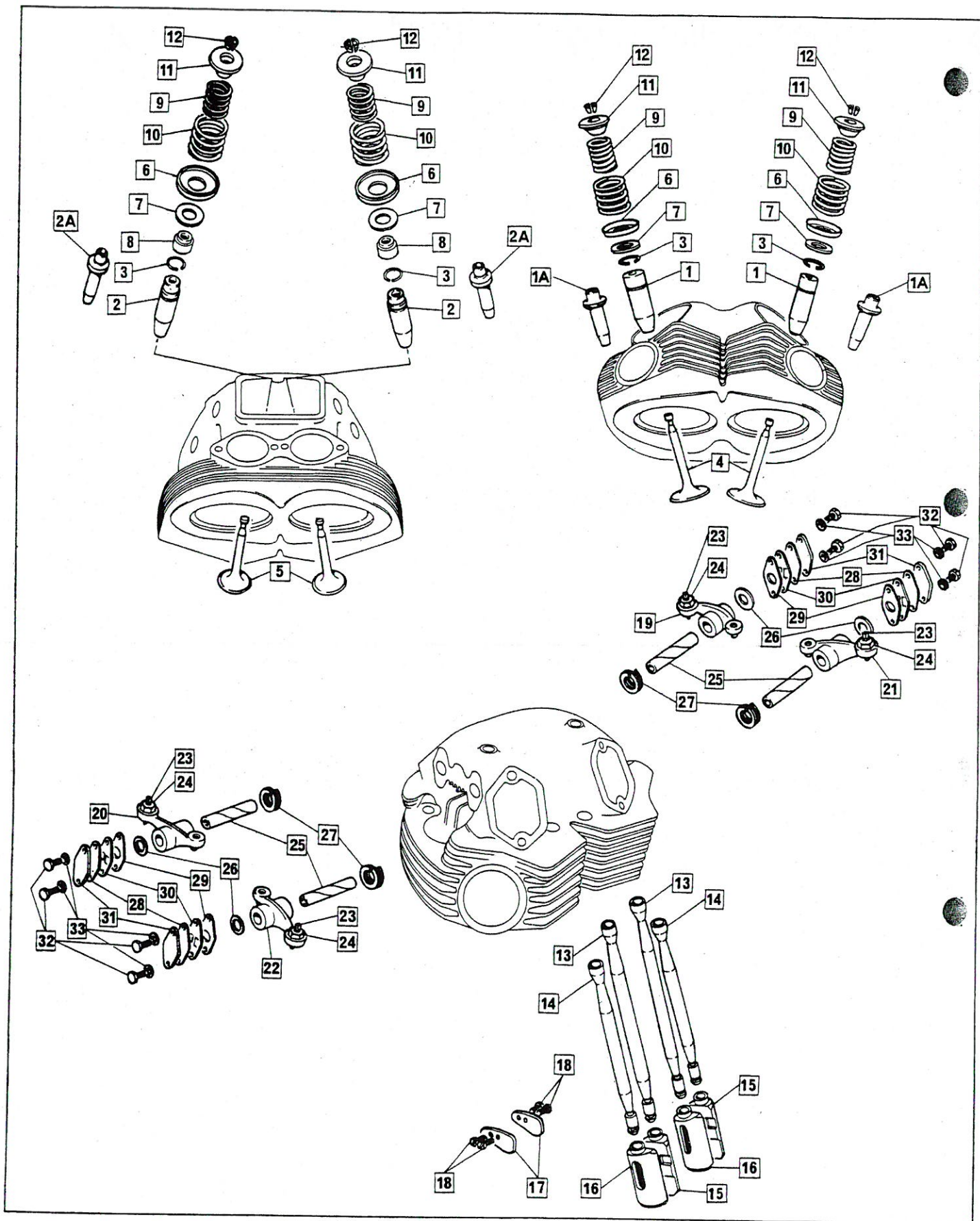
Valve Gear
