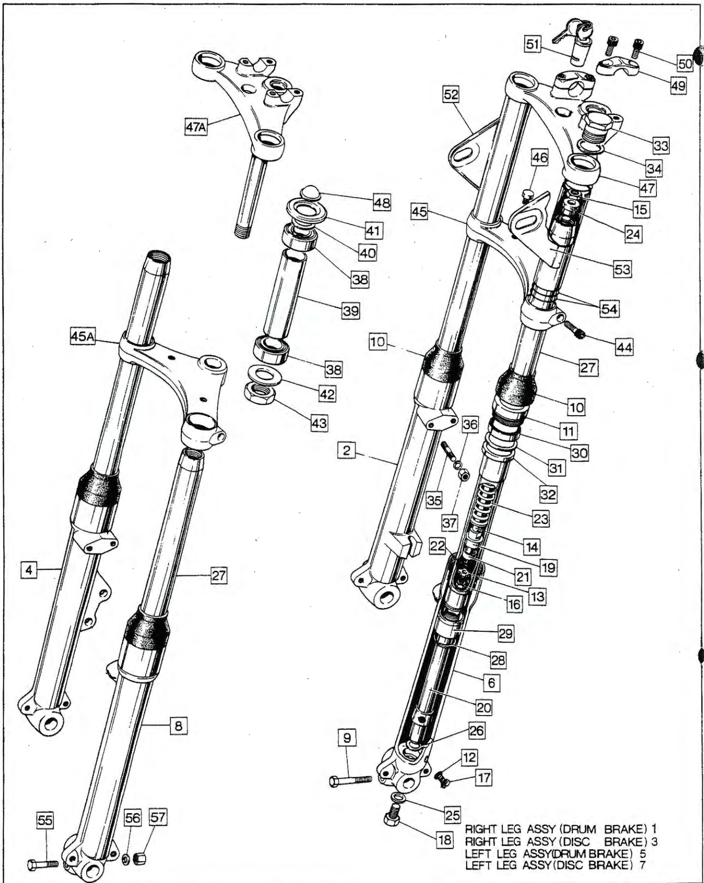
Front Forks, Steering Lock, Steering Head Bearings
