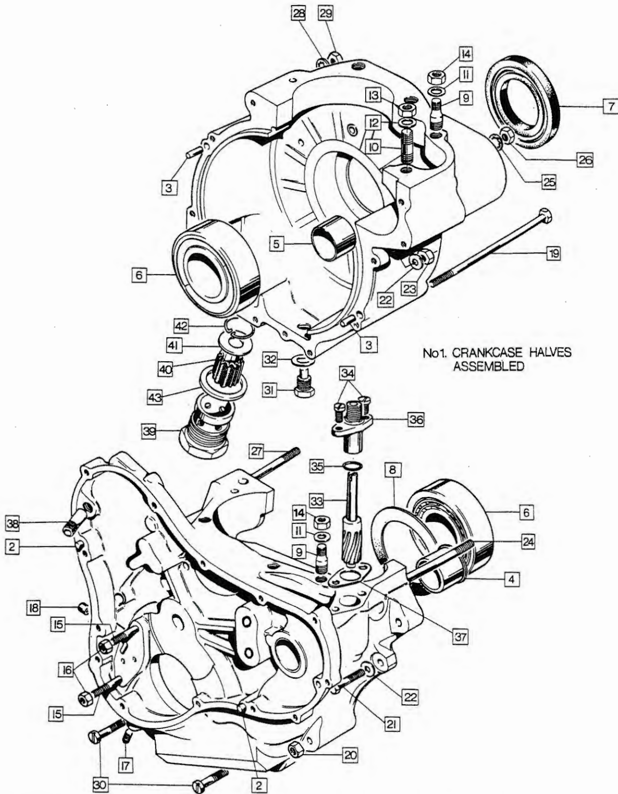
850 Engine: Crankcases, Filter, Breather, Tachometer Drive
