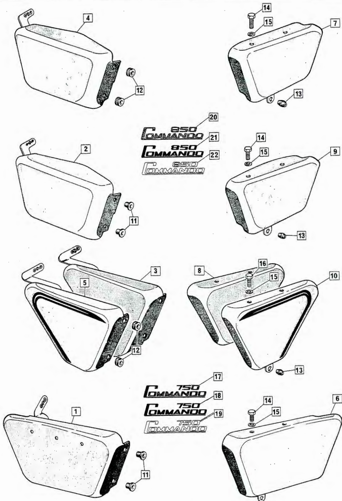
Side Covers, Accessory Covers
