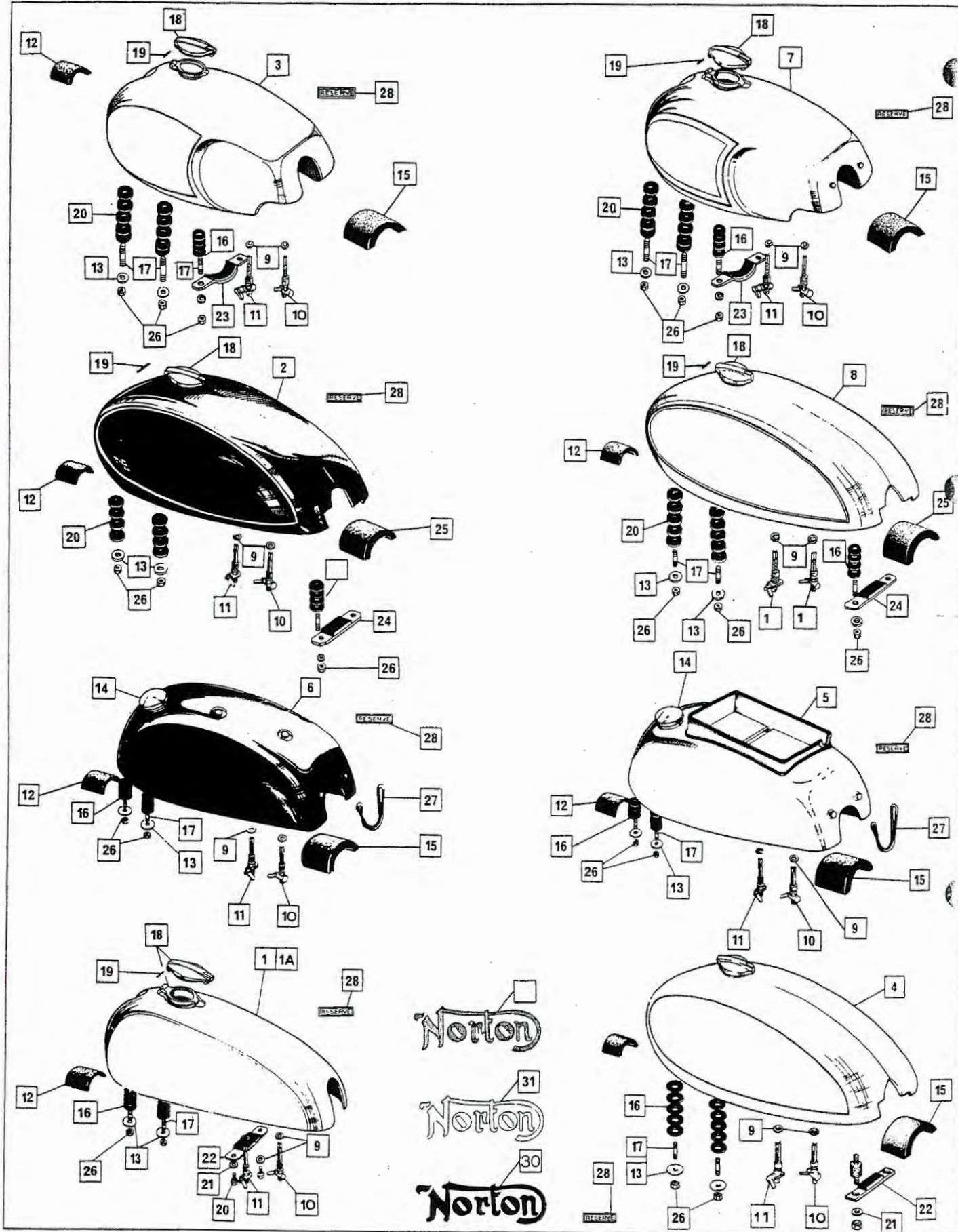
Fuel Tanks
