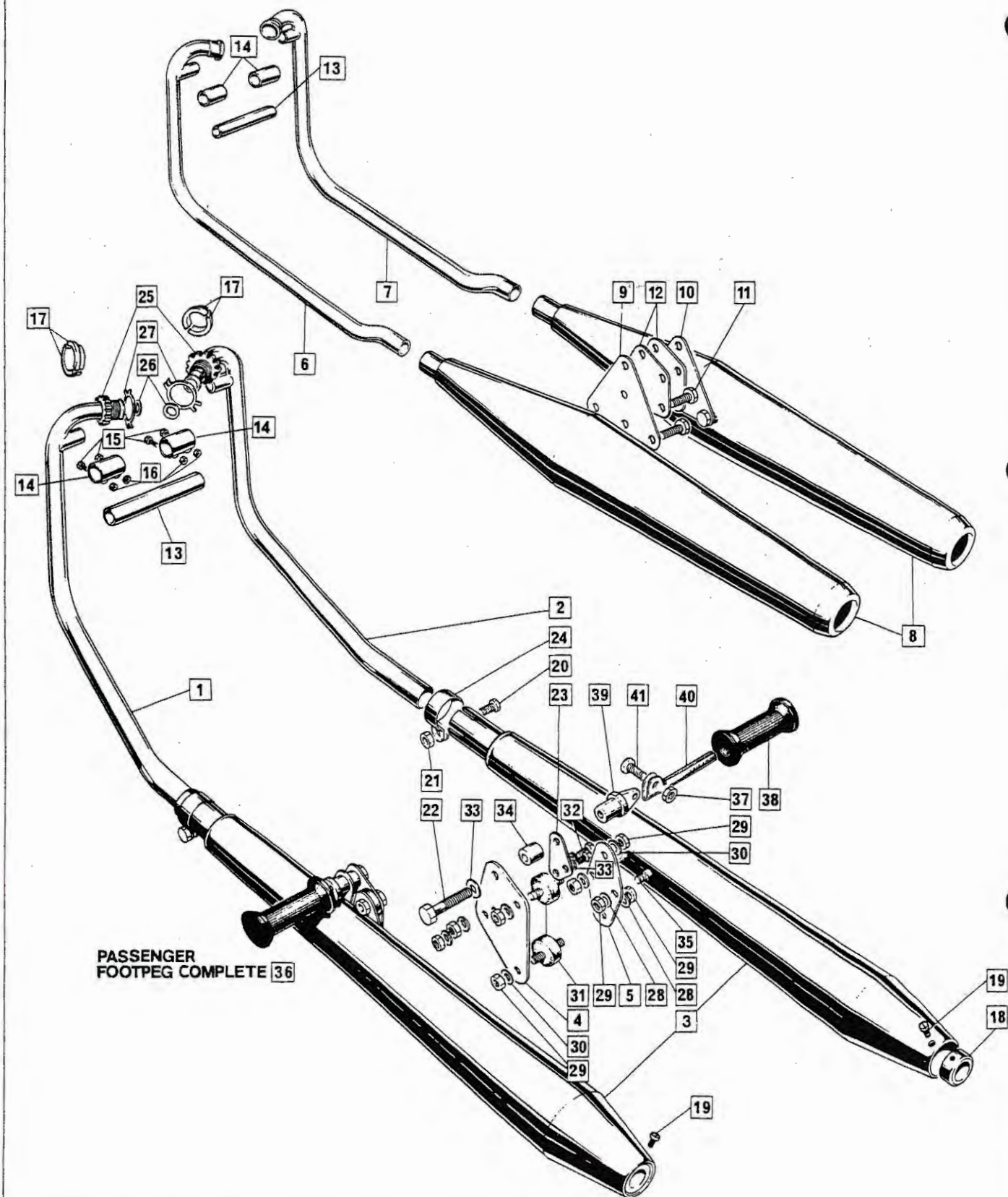
850 Exhausts, Mufflers, Mutes, Passenger Footpegs
