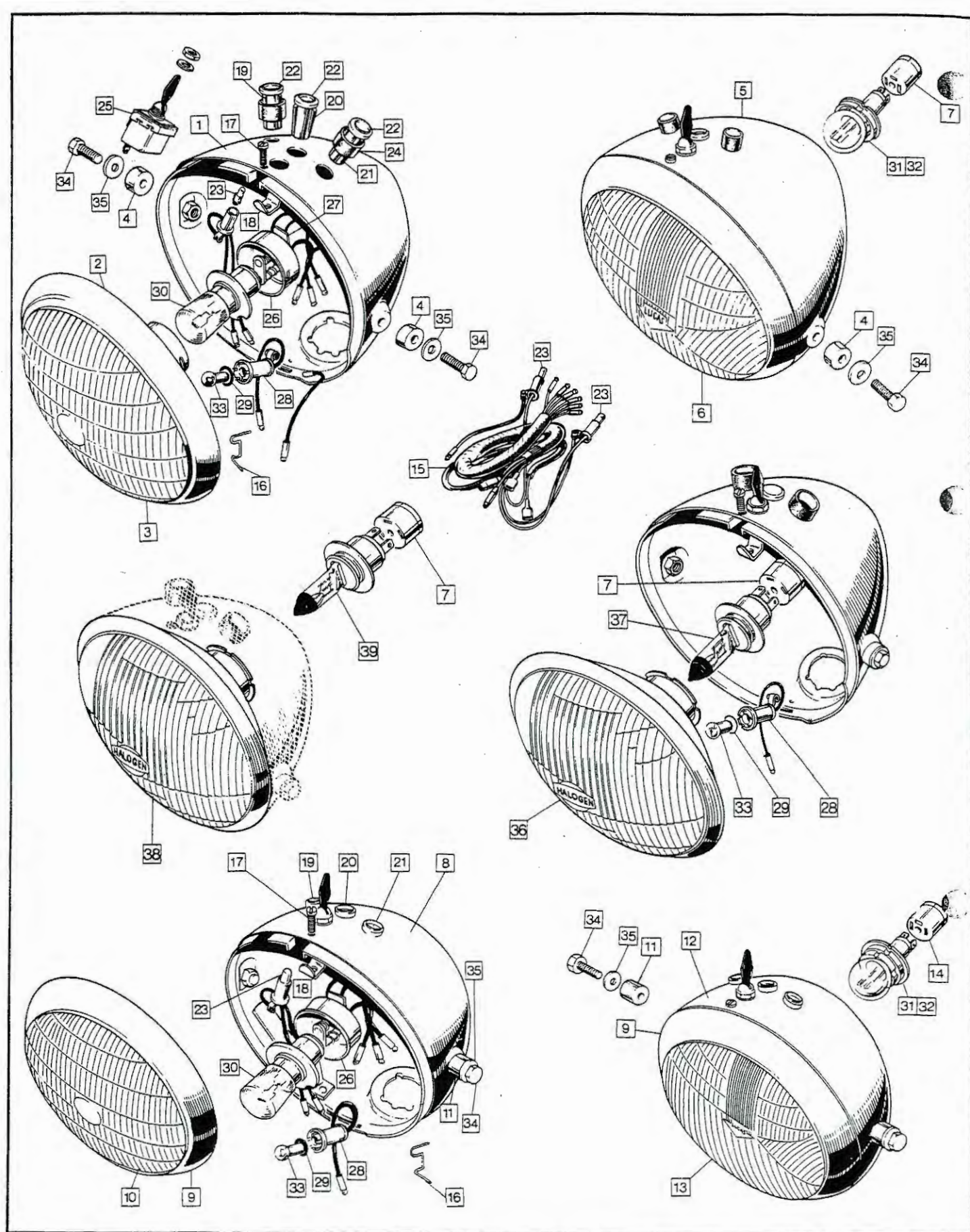
Head Lights
