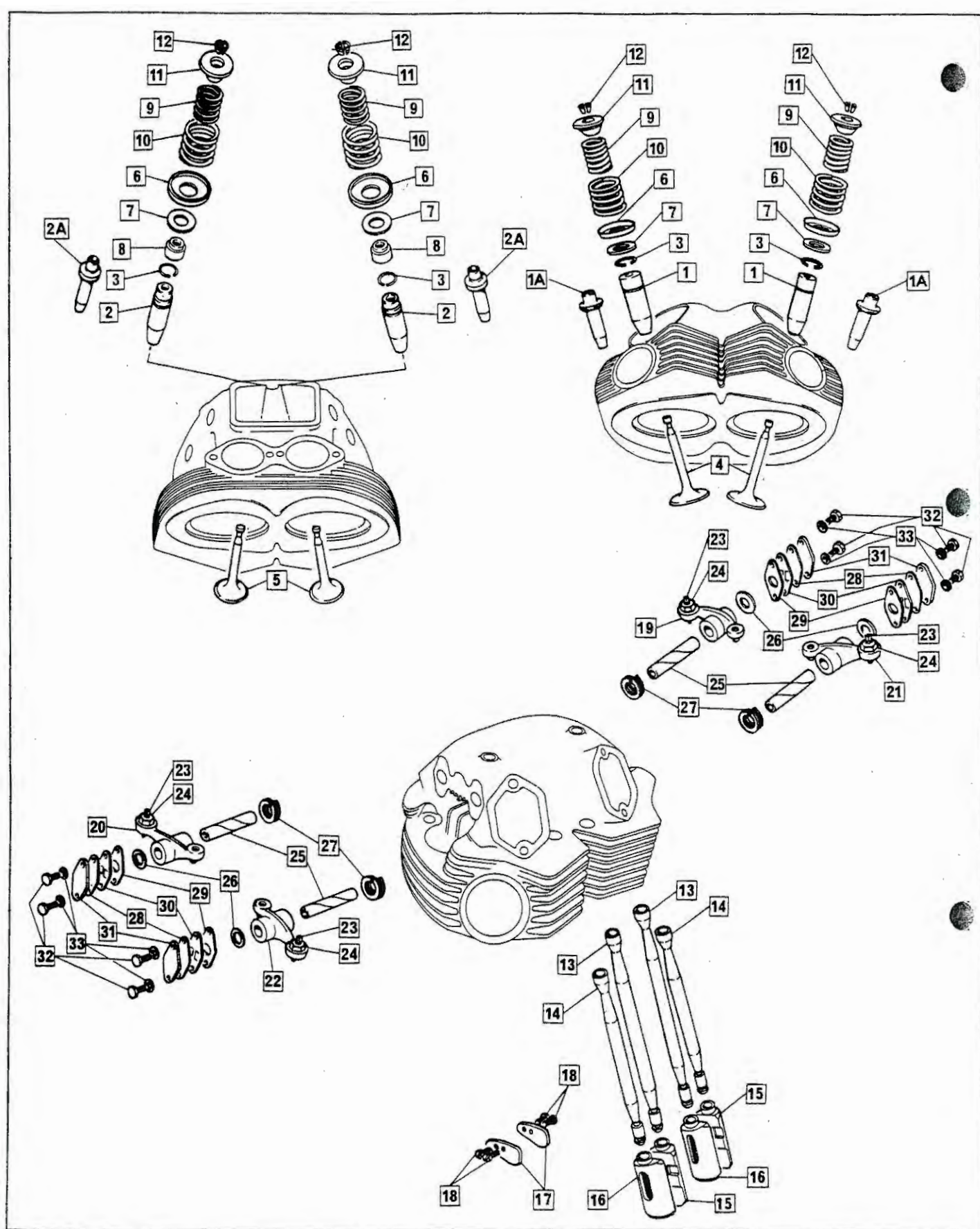
Valve Gear
