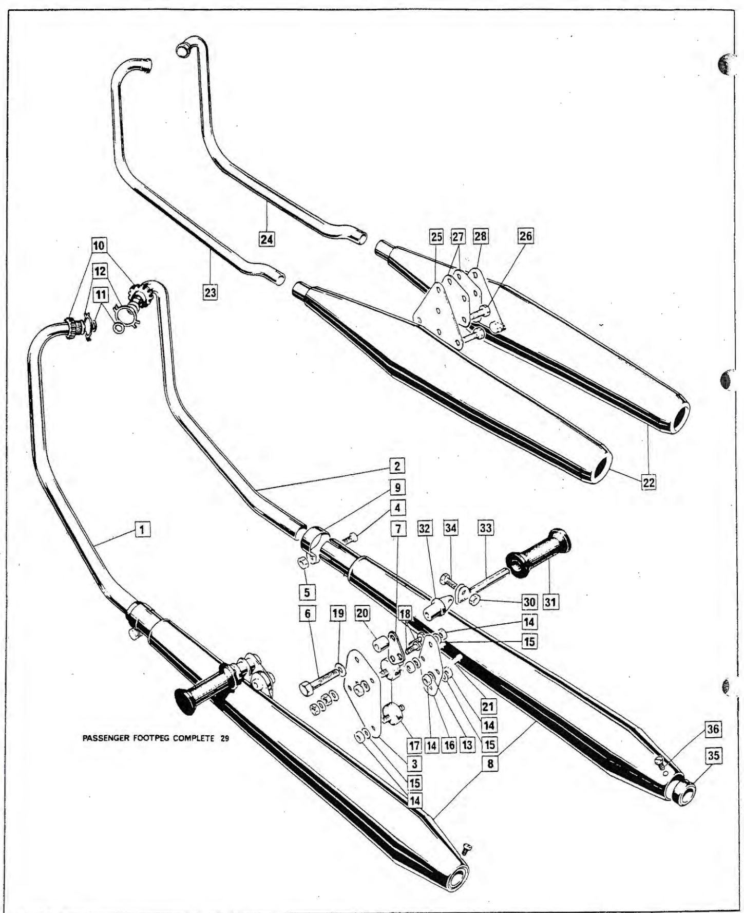
750 Exhausts, Mufflers, Mutes, Passenger Footpegs
