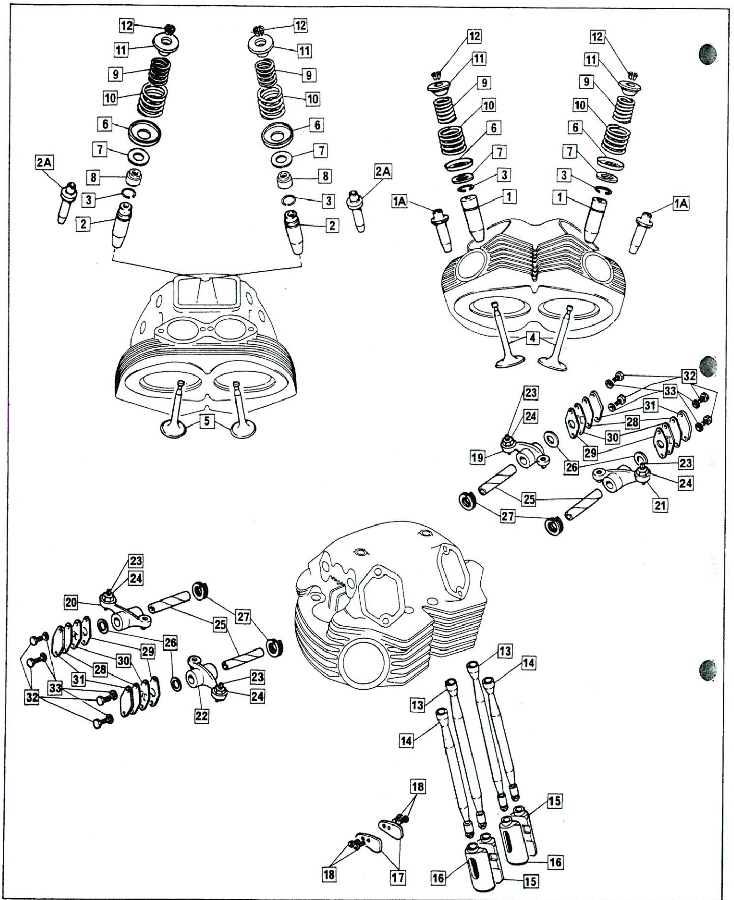
Valve Gear
