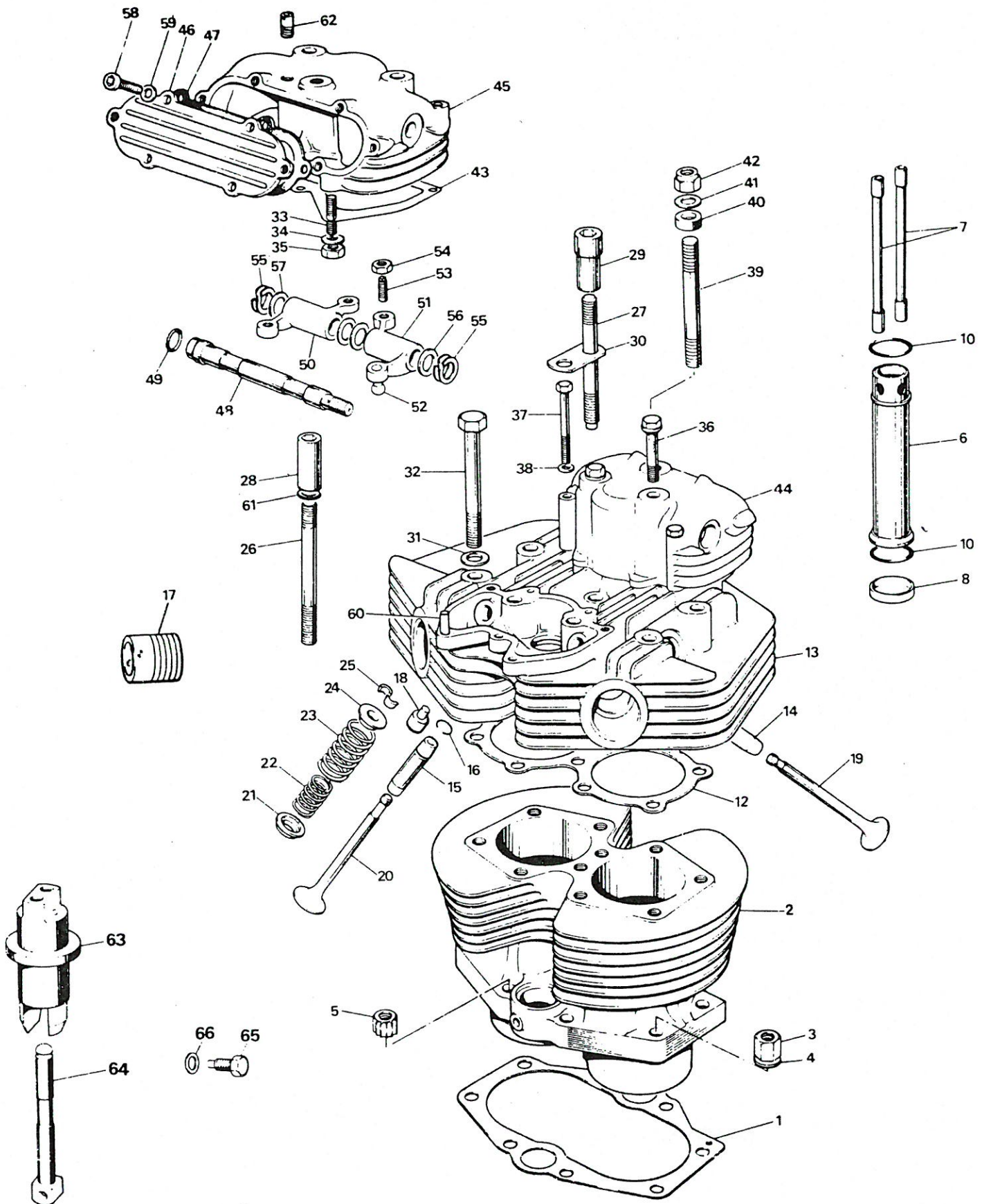
CYLINDER BLOCK AND HEAD
