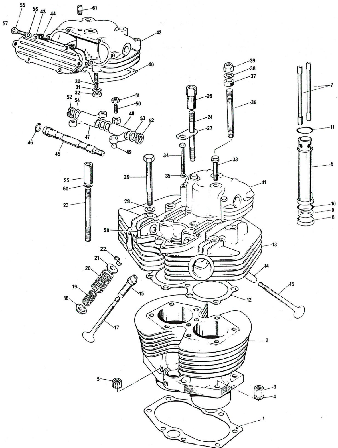
CYLINDER BLOCK & HEAD, T140E
