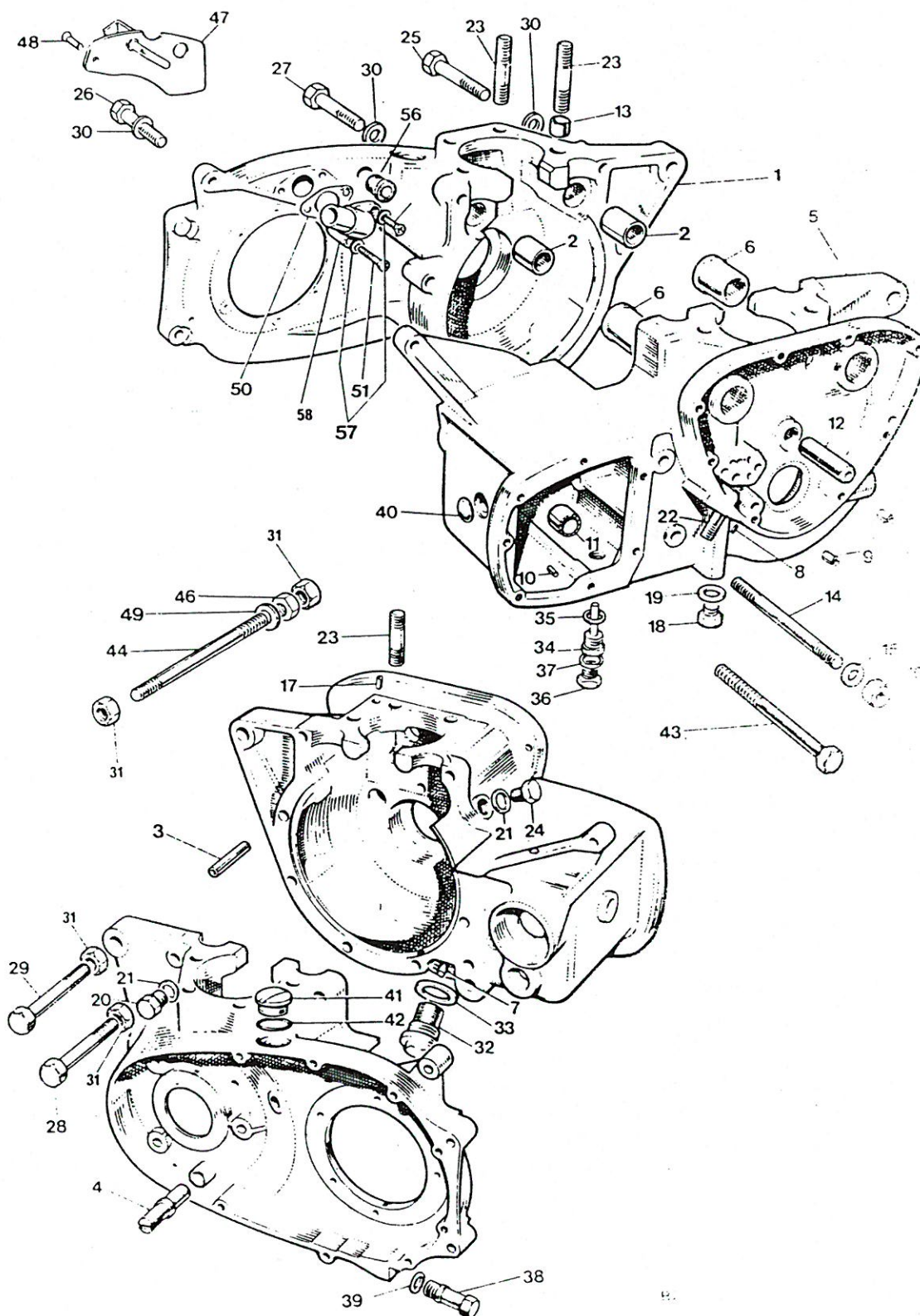
Fig. 2 CRANKCASE
