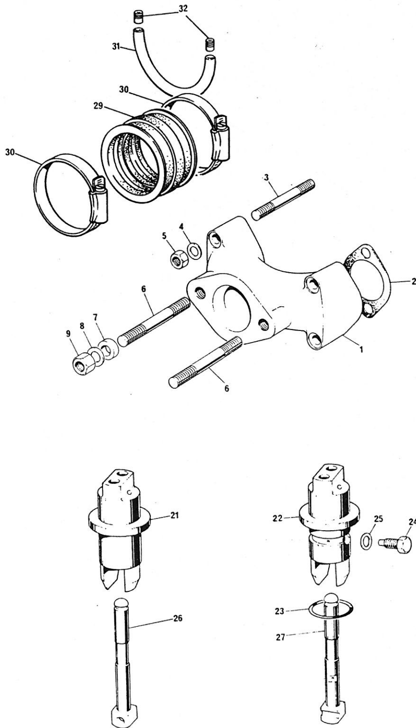
Fig. 4. MANIFOLD AND TAPPETS
