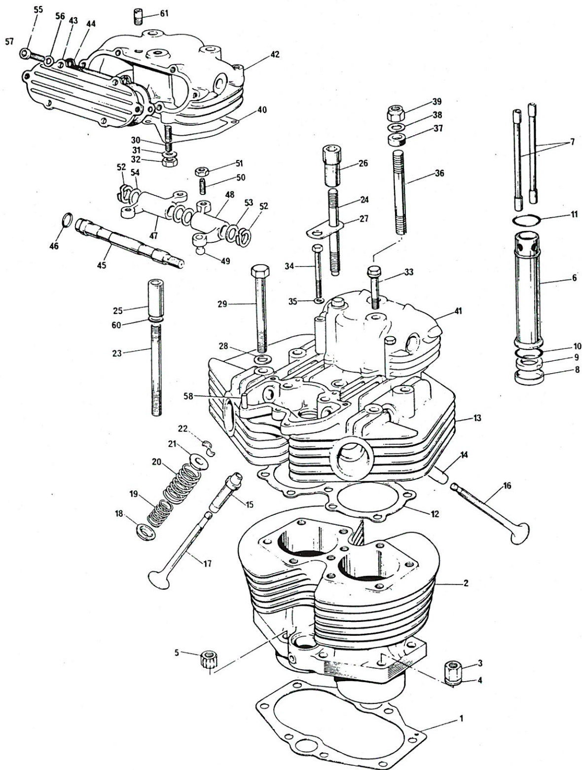
CYLINDER BLOCK & HEAD, TR7
