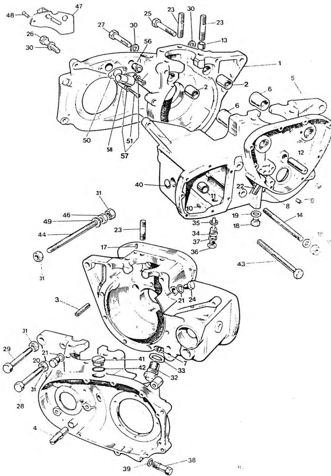
Fig. 2 CRANKCASE
