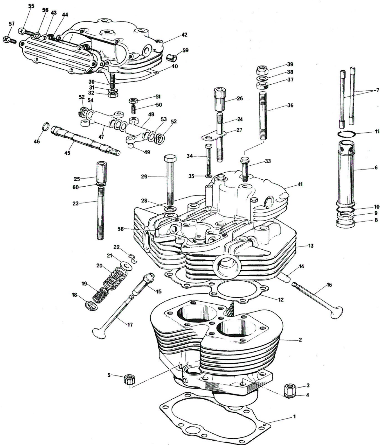
CYLINDER BLOCK AND HEAD, T140V
