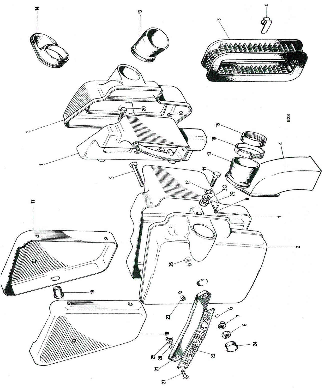
Fig. 26 AIR CLEANERS AND SIDE PANELS
