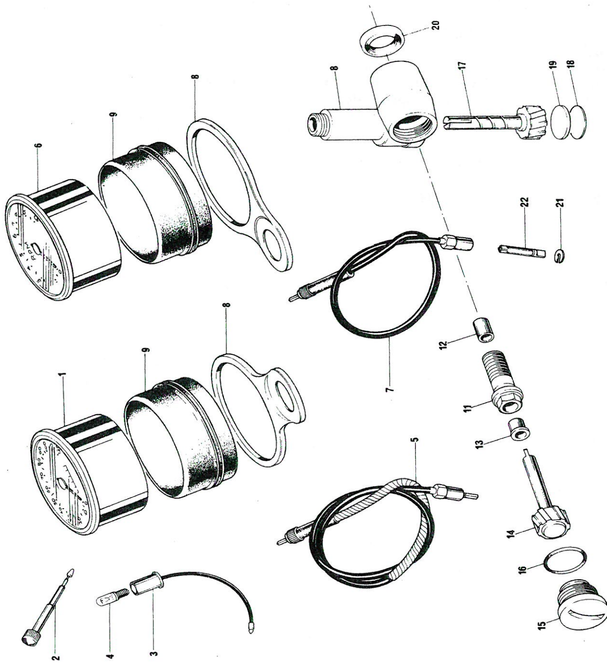
Fig. 32. SPEEDOMETER AND TACHOMETER
