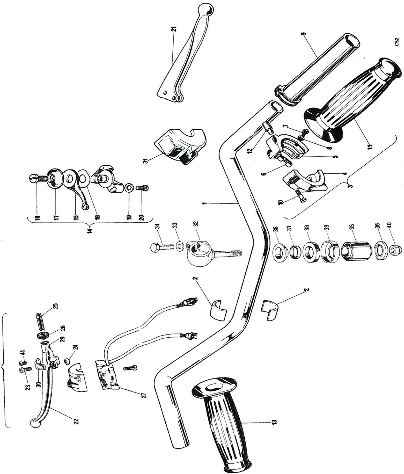
Fig. 29. HAND LEVER AND CONTROL LEVERS
