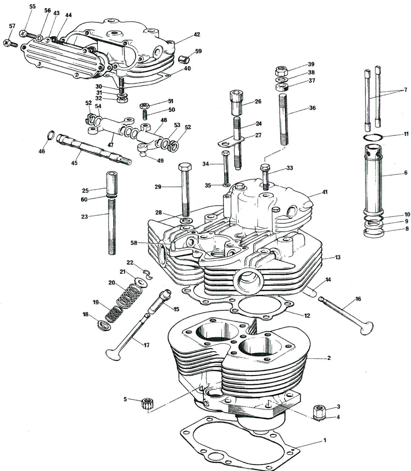
CYLINDER BLOCK AND HEAD, T140V
