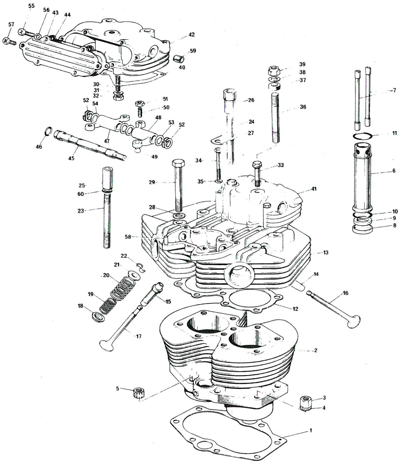
Fig. 5. CYLINDER BLOCK AND HEAD, TR7RV
