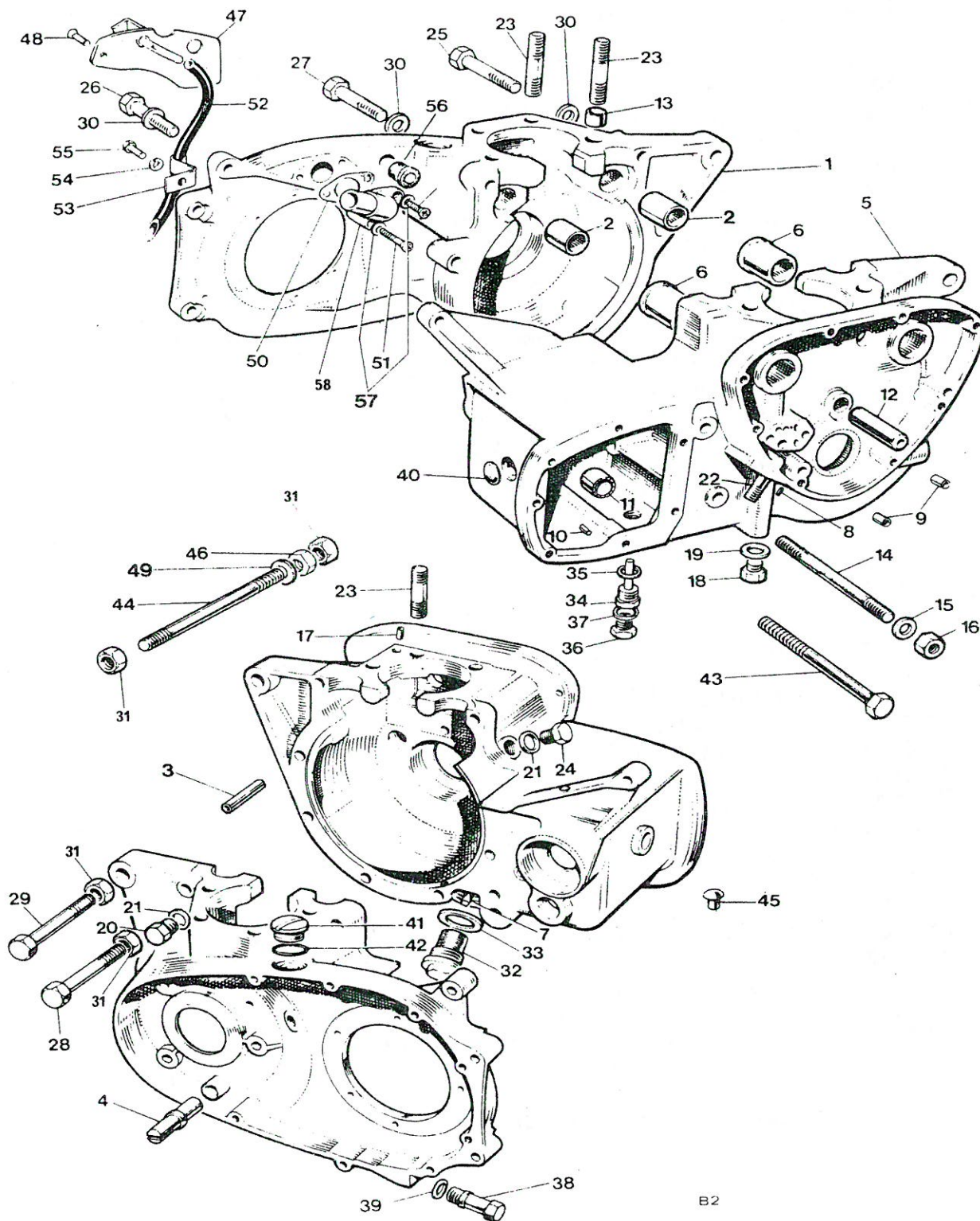
Fig. 2 CRANKCASE
