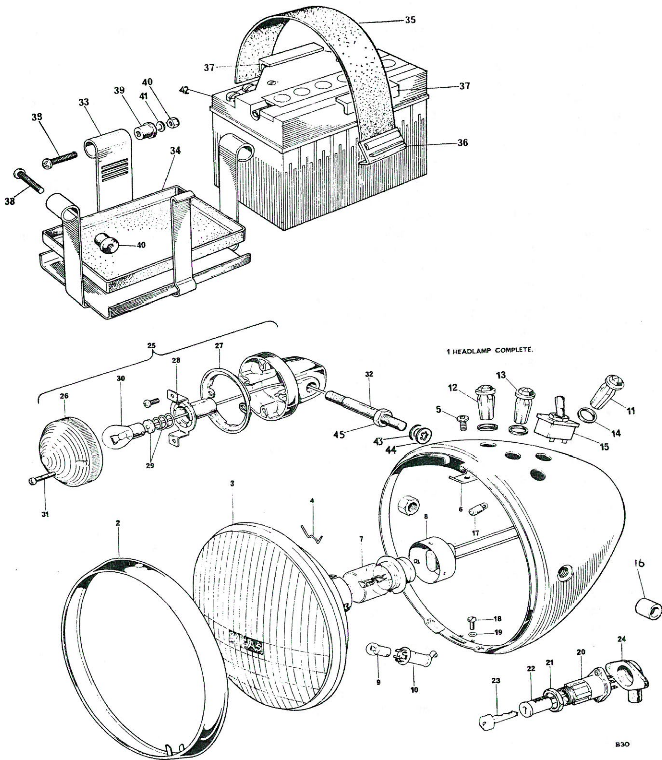
Fig. 34. HEADLAMP AND FLASHER LAMPS
