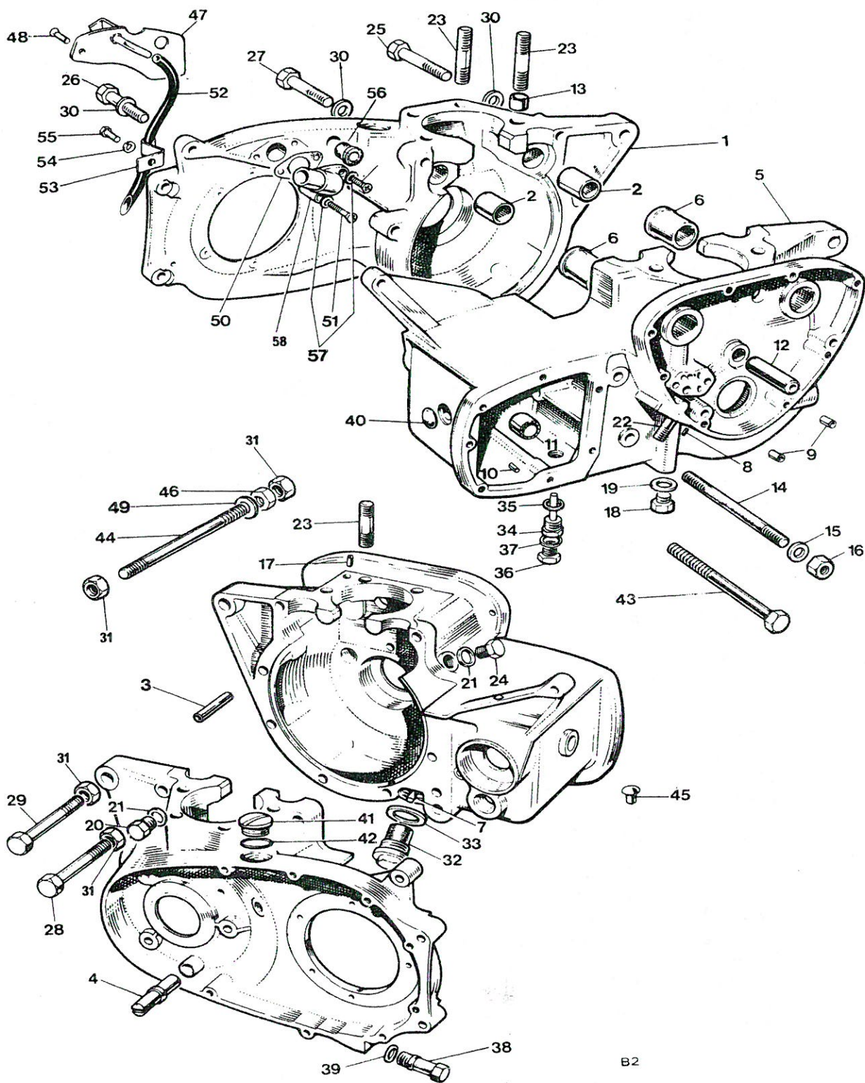
Fig. 2 CRANKCASE
