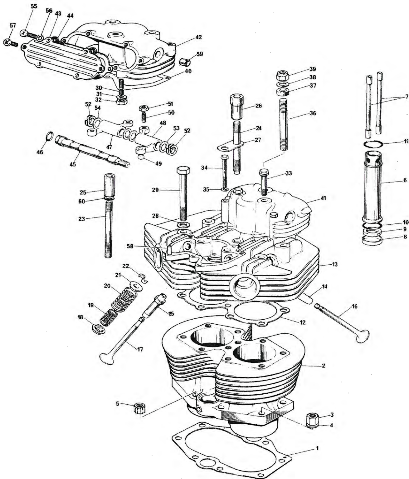
CYLINDER BLOCK AND HEAD, TI40V
