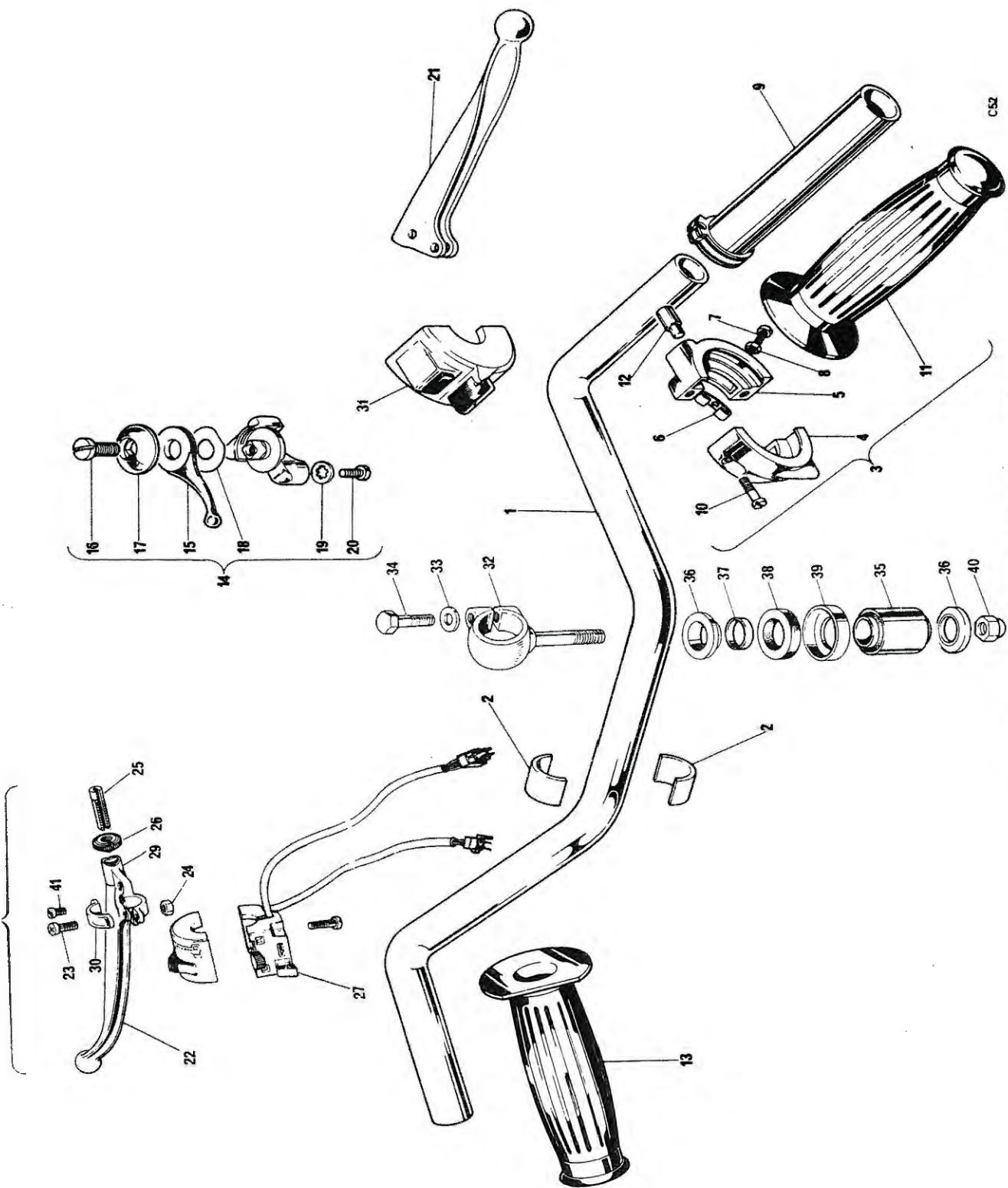
FIG. 29. HANDLEBAR AND CONTROL LEVERS
