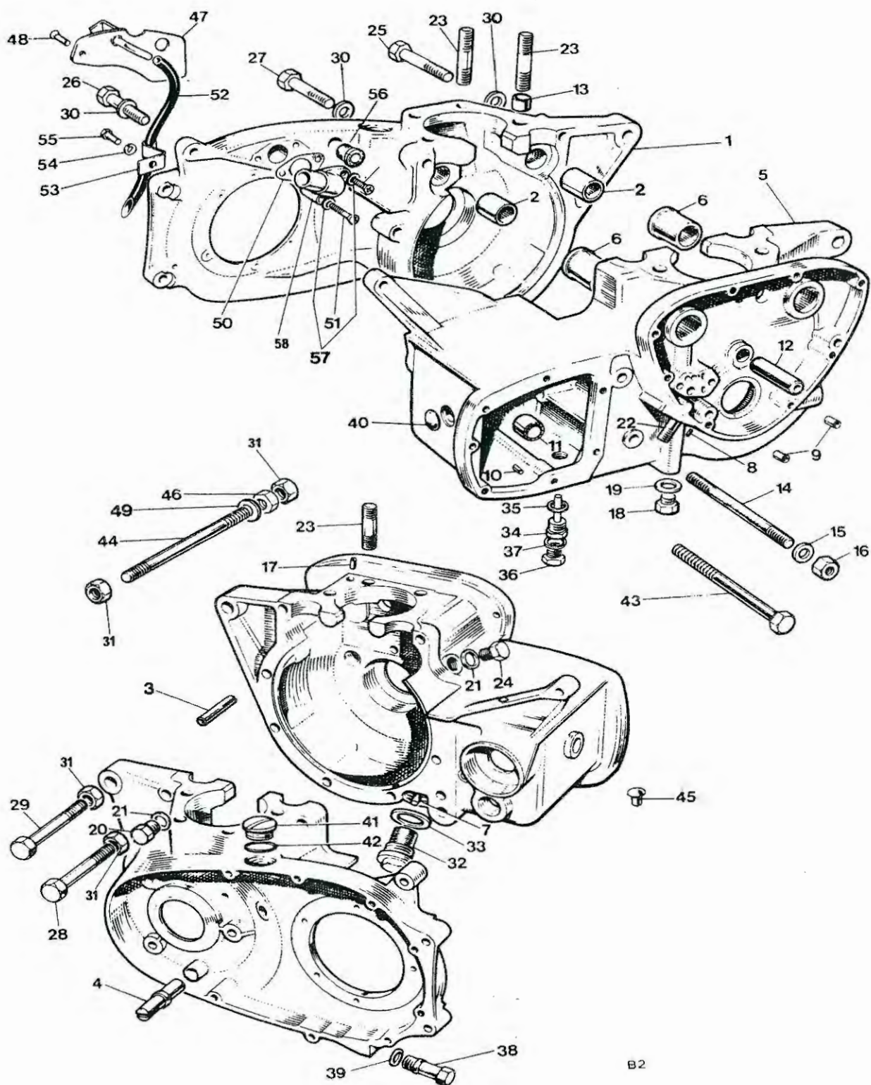
Fig. 2 CRANKCASE
