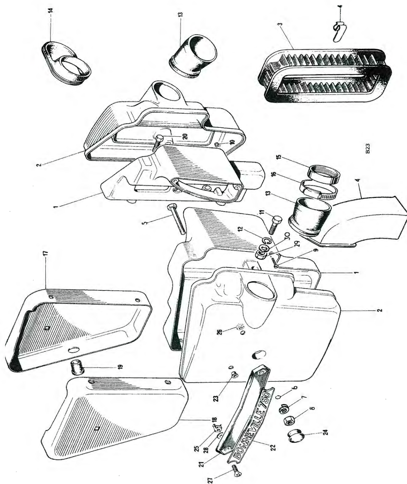
Fig. 26 AIR CLEANERS AND SIDE PANELS
