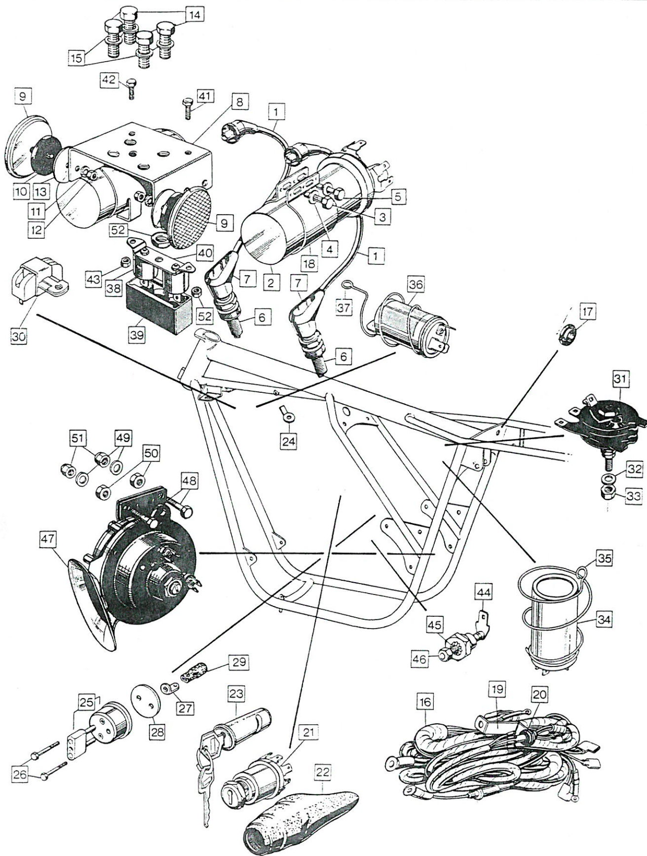
Basic Electrical Components
