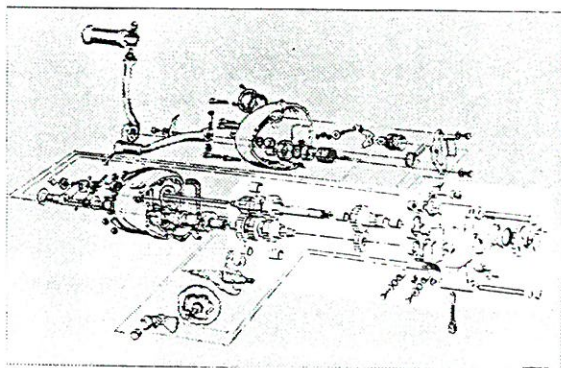
Gearbox: Shell, Gear Cluster, Mounting Bolts, Adjuster and Countershaft Sprockets
