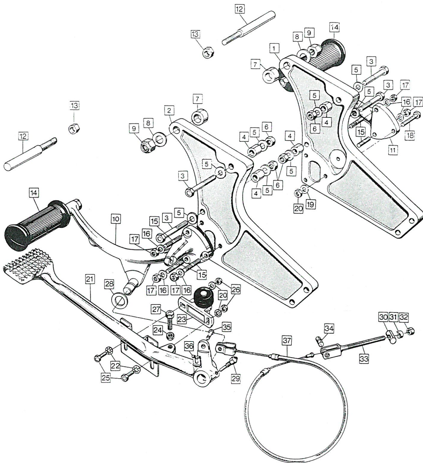
Support Plates, Riders Footpegs, Rear Brake Pedal and Linkage
