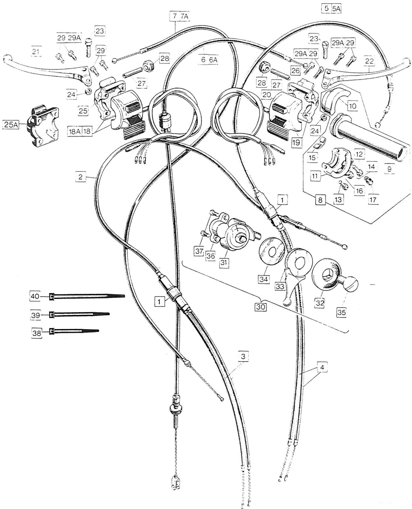
Controls and Control Cables
