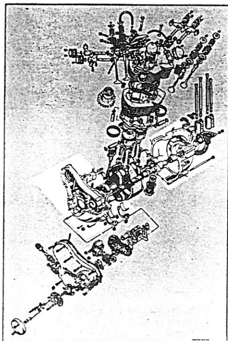
Engine: Crankcases, Crankcase Breather, Tachometer Drive
