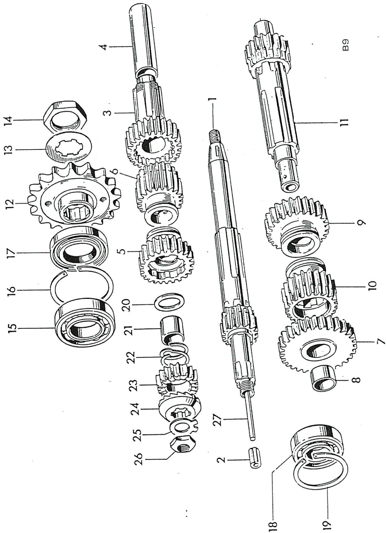
Fig. 10 GEARBOX SHAFTS AND GEARS
