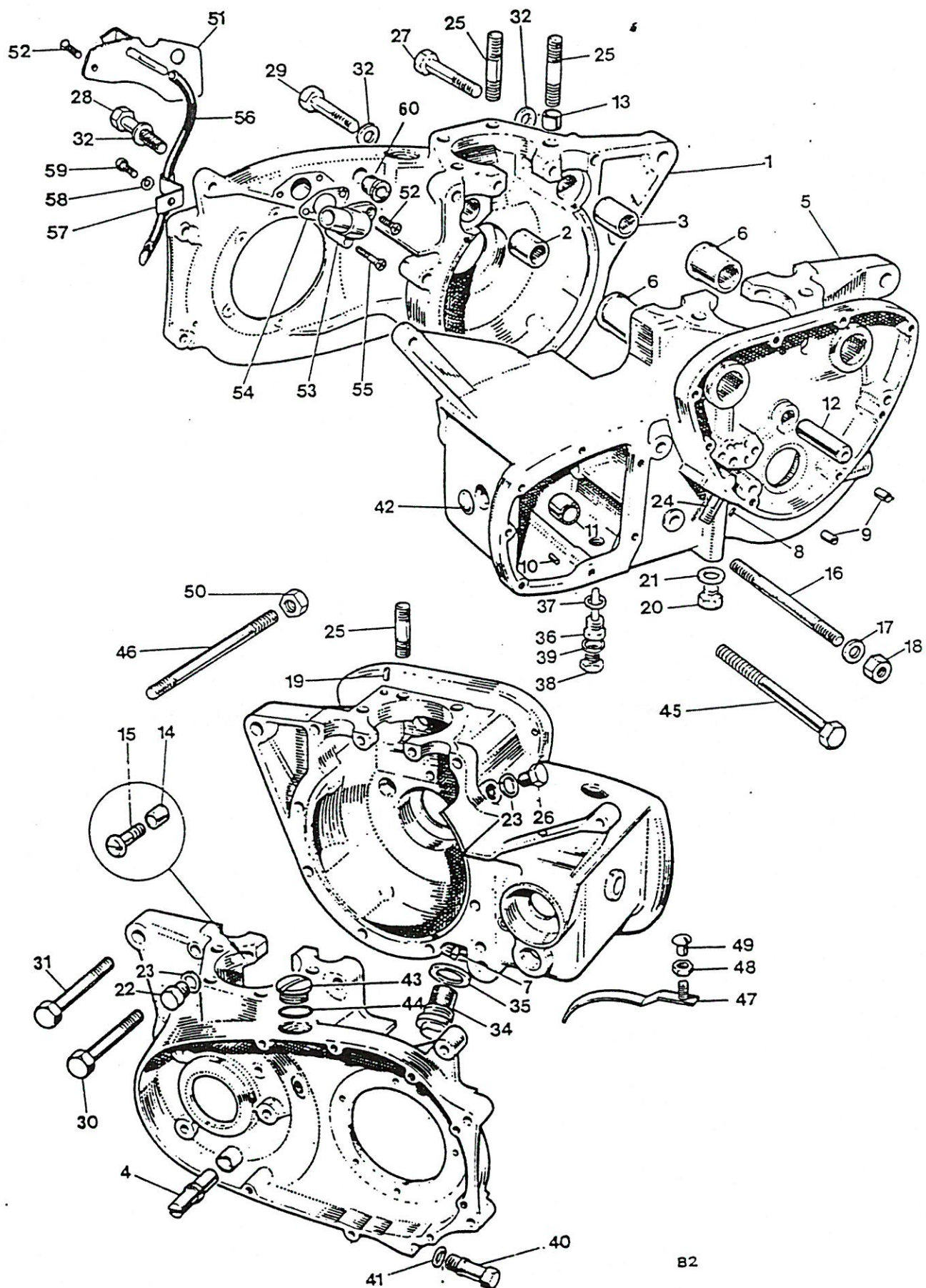
Fig. 2 CRANKCASE
