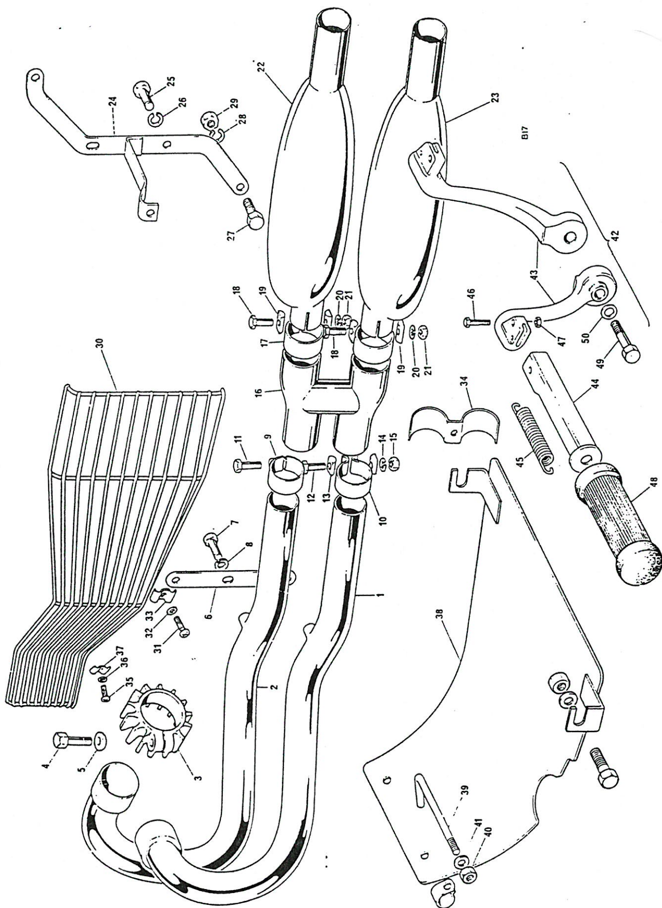
Fig. 18. EXHAUST PIPES AND MUFFLERS, TR6C
