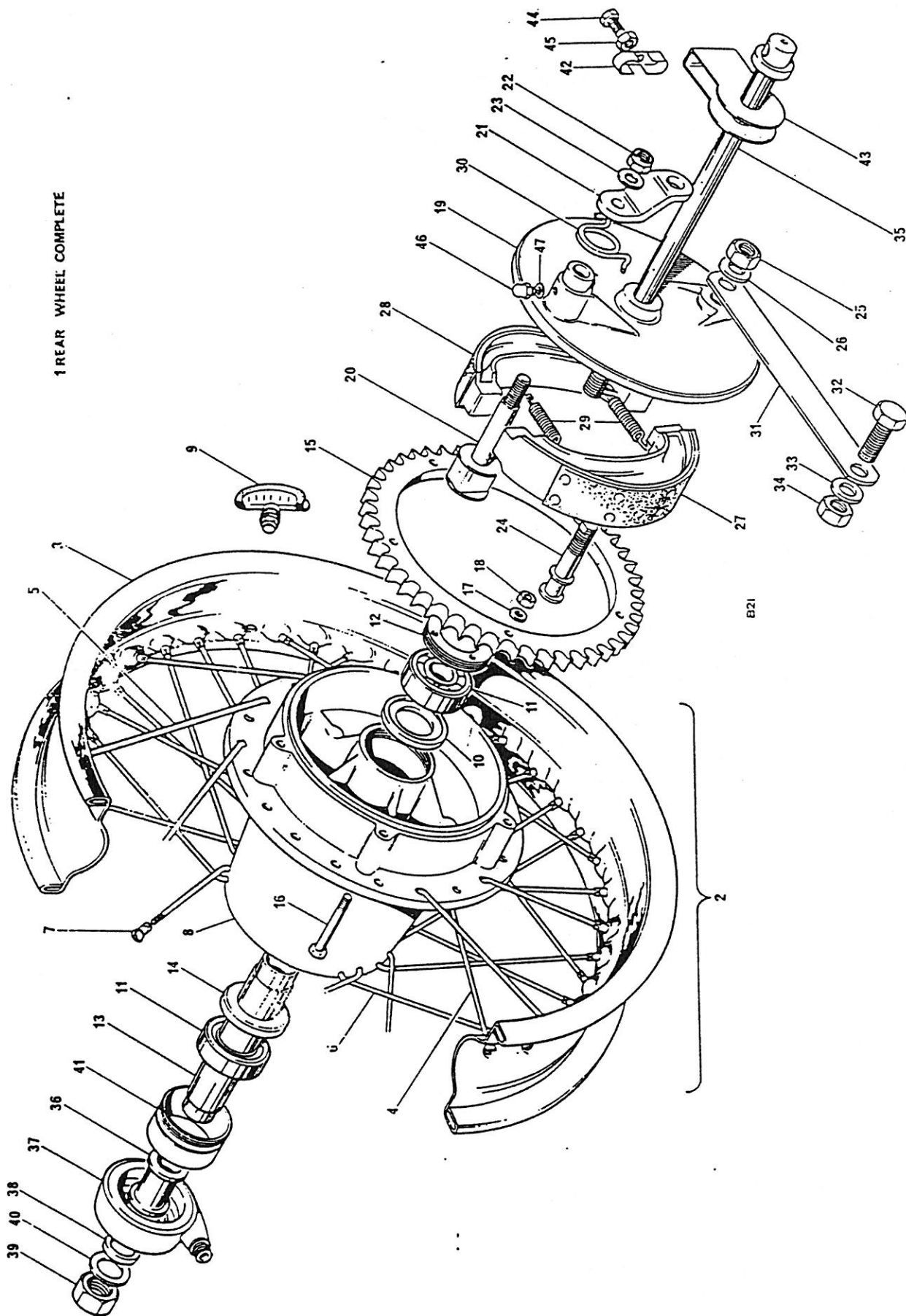
Fig. 22. REAR WHEEL
