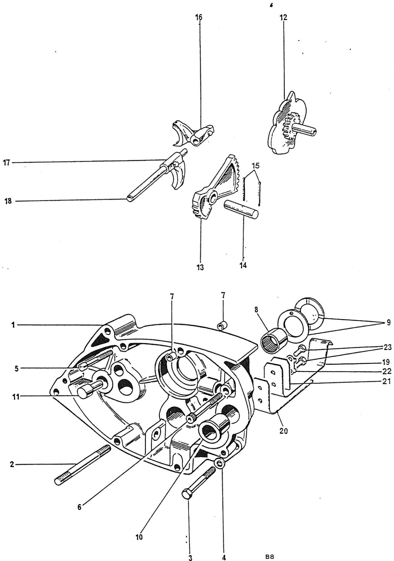
Fig. 9 GEARBOX INNER COVER AND SELECTORS
