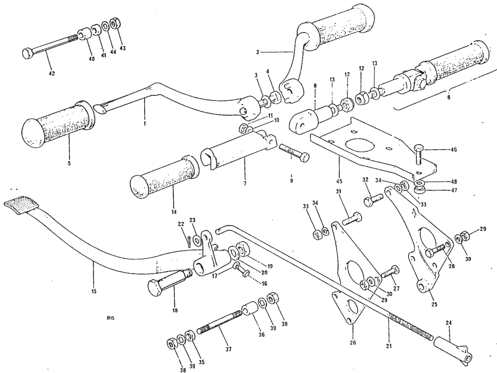
Fig. 16. MOTOR UNIT FITTING AND FOOTRESTS
