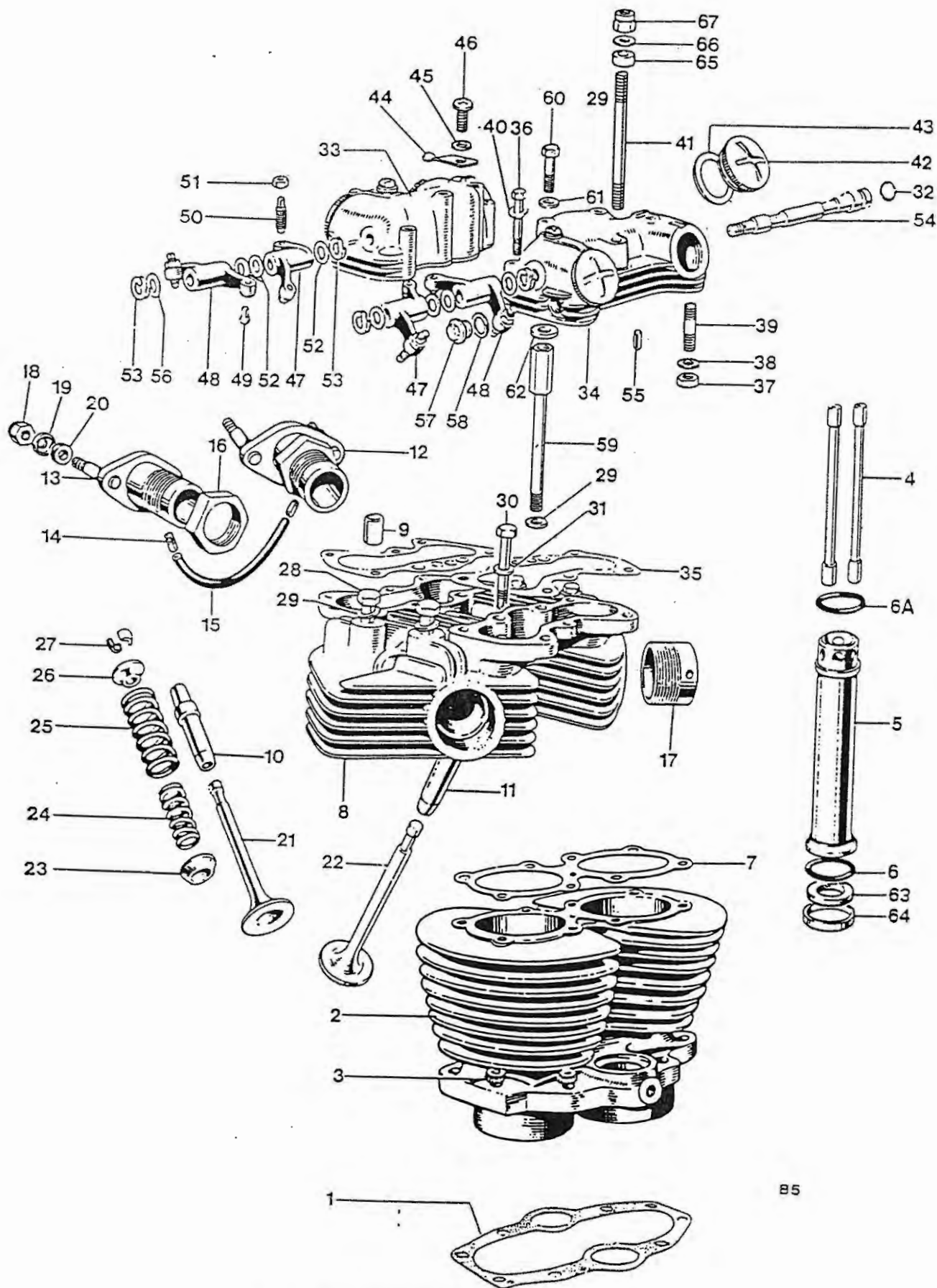
Fig. 5. CYLINDER BLOCK AND HEAD, T120R
