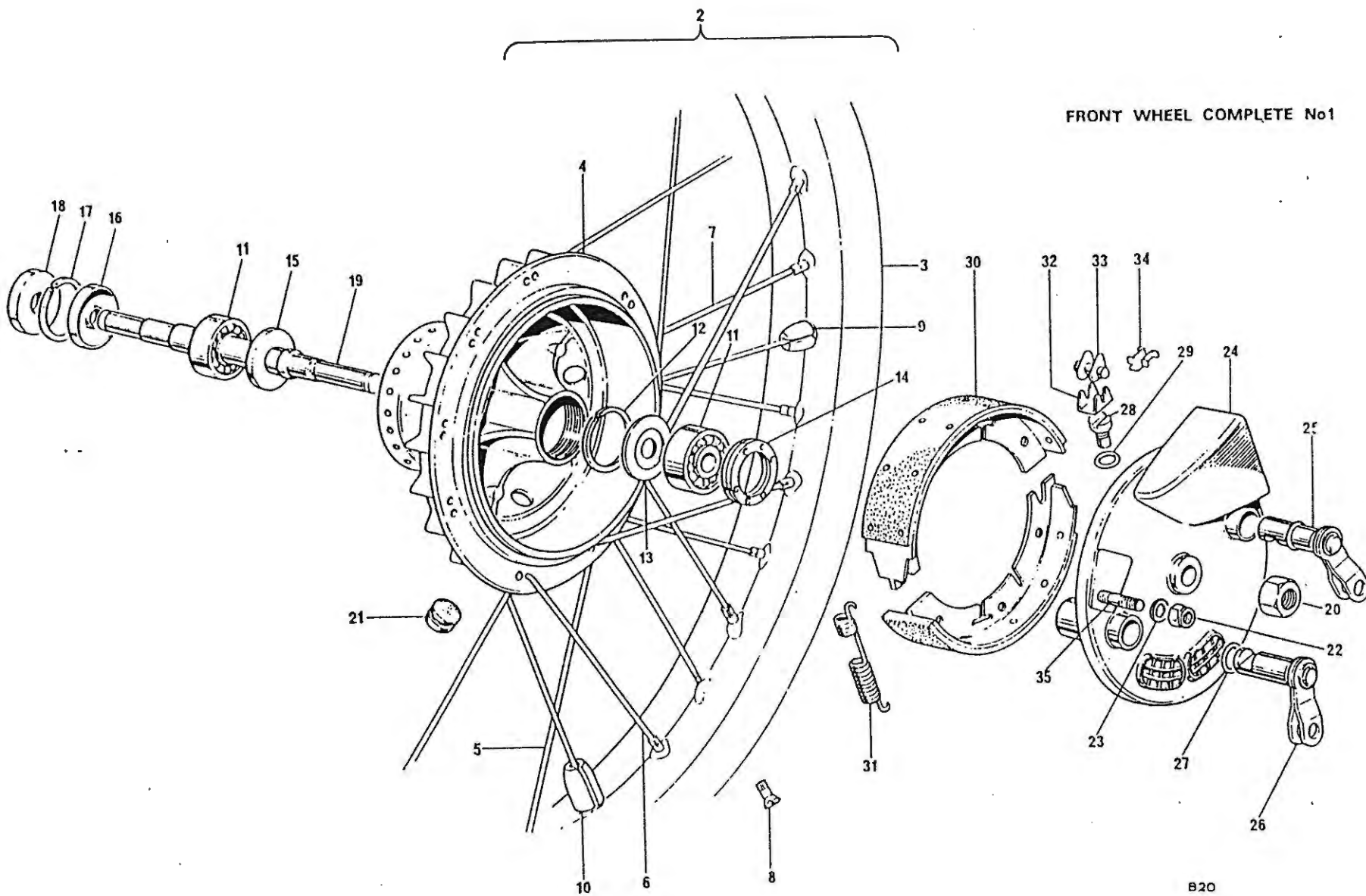
Fig. 21. FRONT WHEEL
