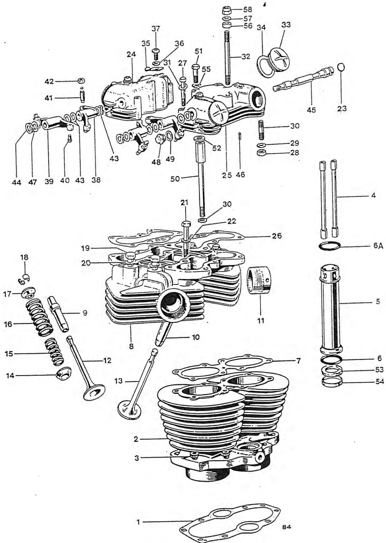
Fig. 4. CYLINDER BLOCK AND HEAD, TR6R, TR6C
