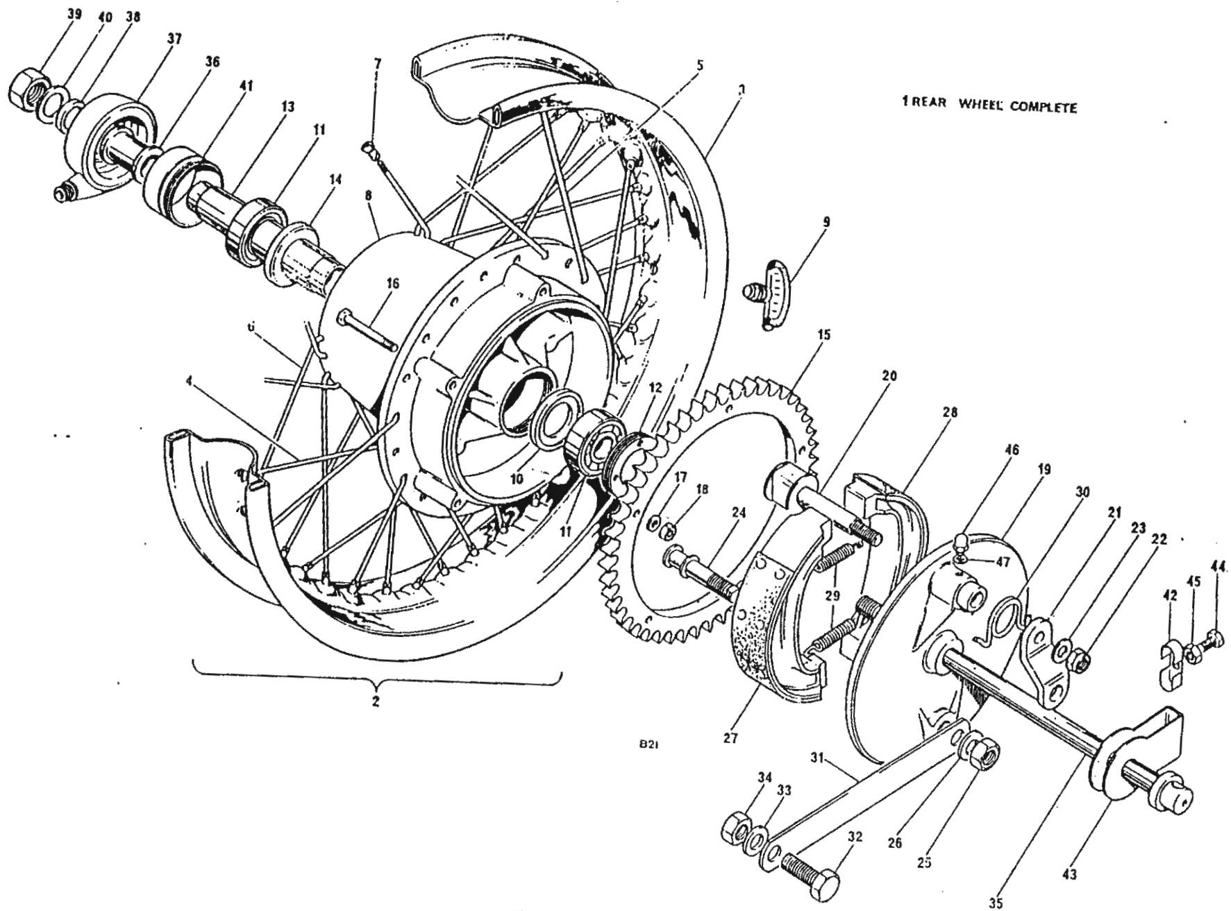
Fig. 22. REAR WHEEL
