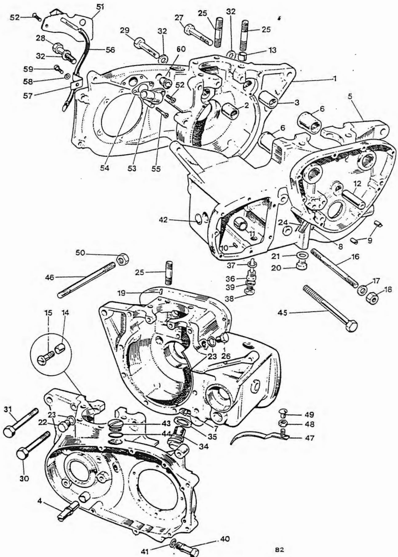
Fig. 2 CRANKCASE
