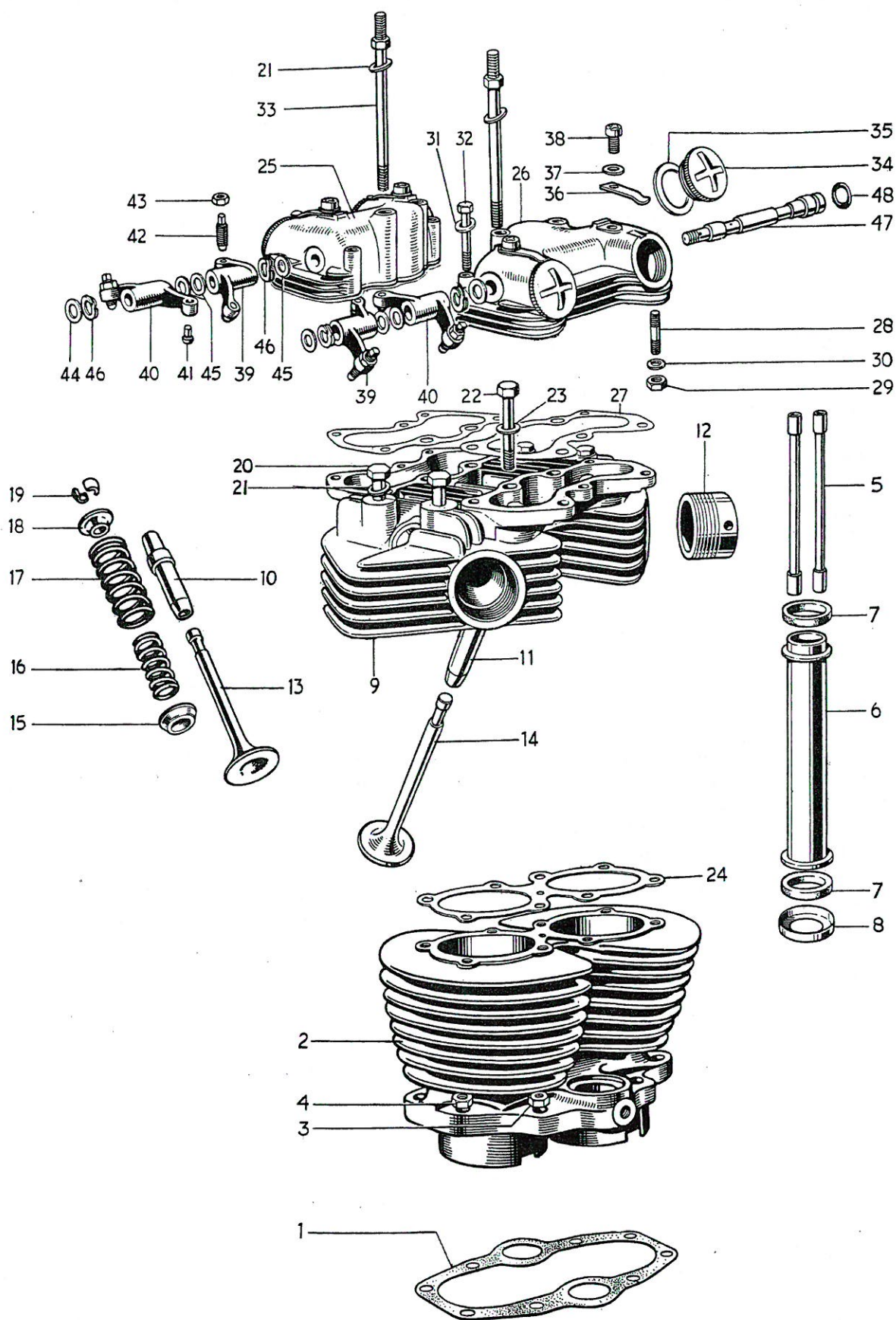
Fig. 4. CYLINDER BLOCK AND HEAD, 6T AND TR6
