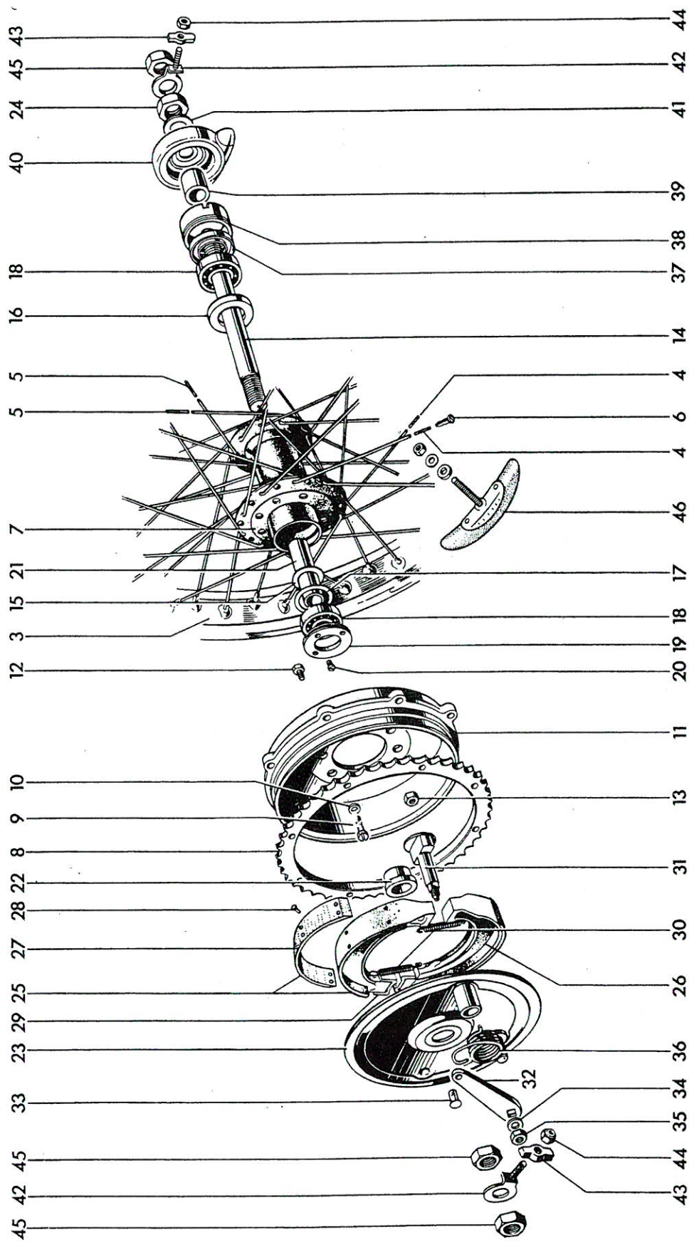
Fig. 23. REAR WHEEL
