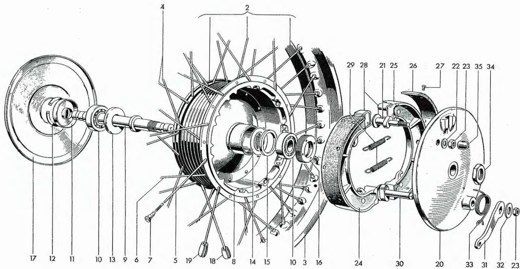
Fig. 22. FRONT WHEEL, TR6 AND U.S.A. T120
