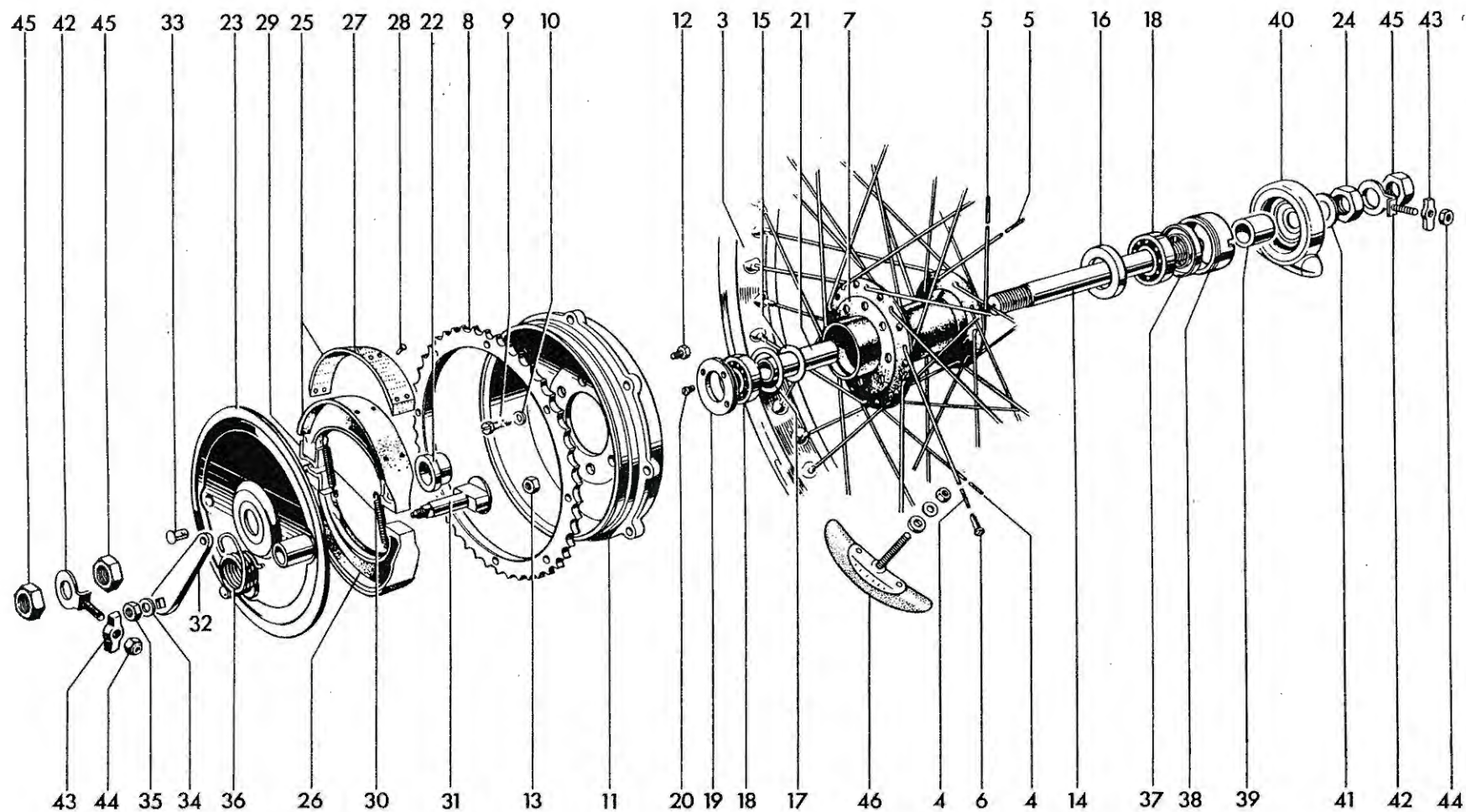
Fig. 23. REAR WHEEL
