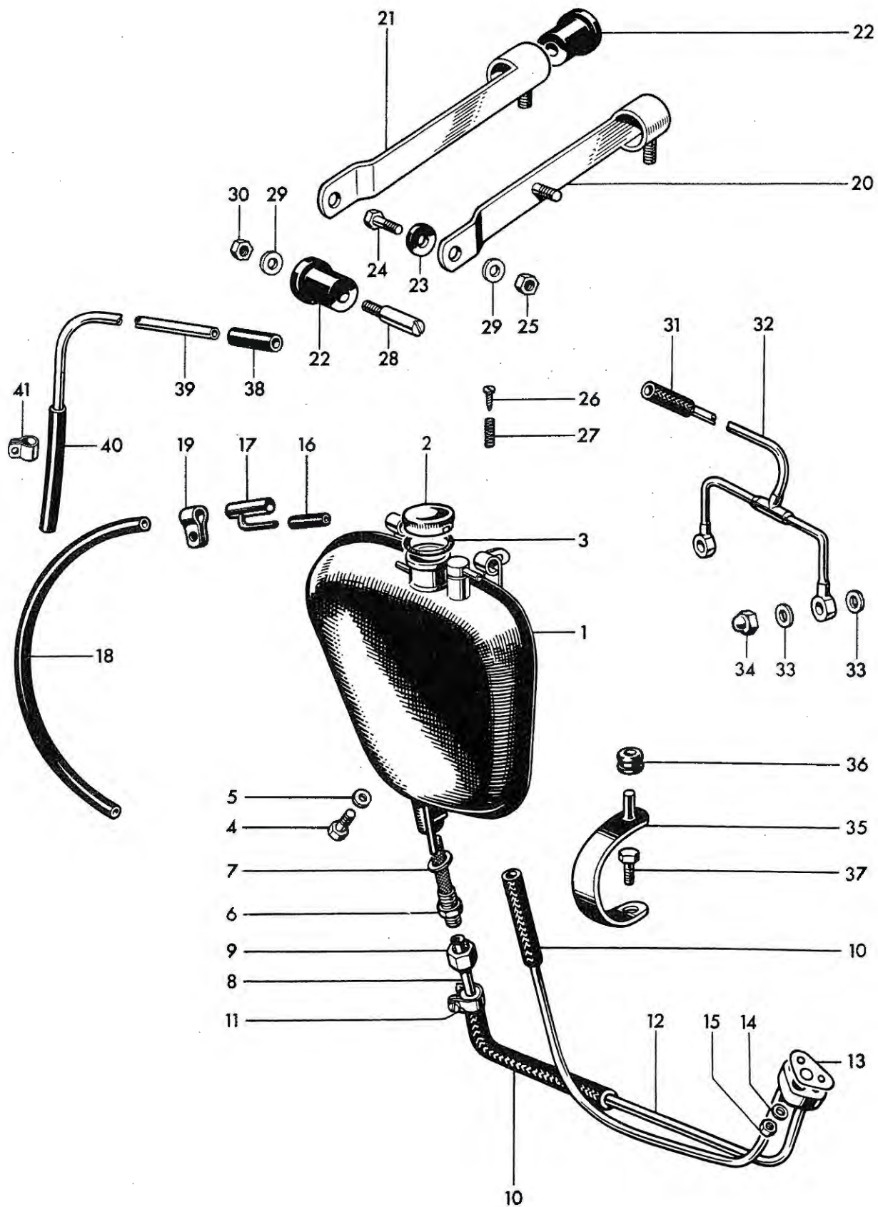
Fig. 26. OIL TANK
