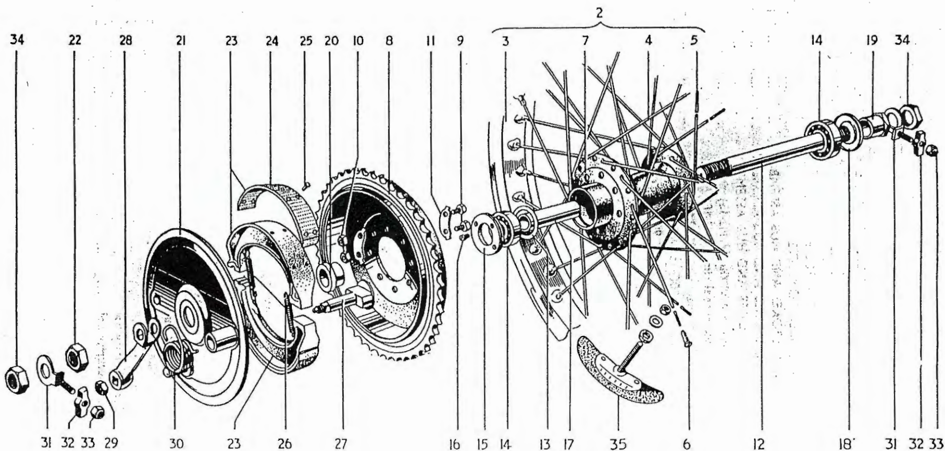
FIG. 21 REAR WHEEL
