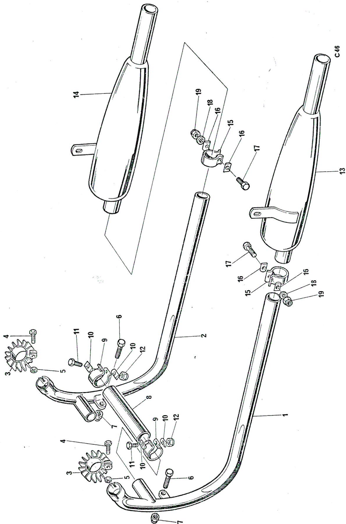
Fig. 12. EXHAUST SYSTEM
