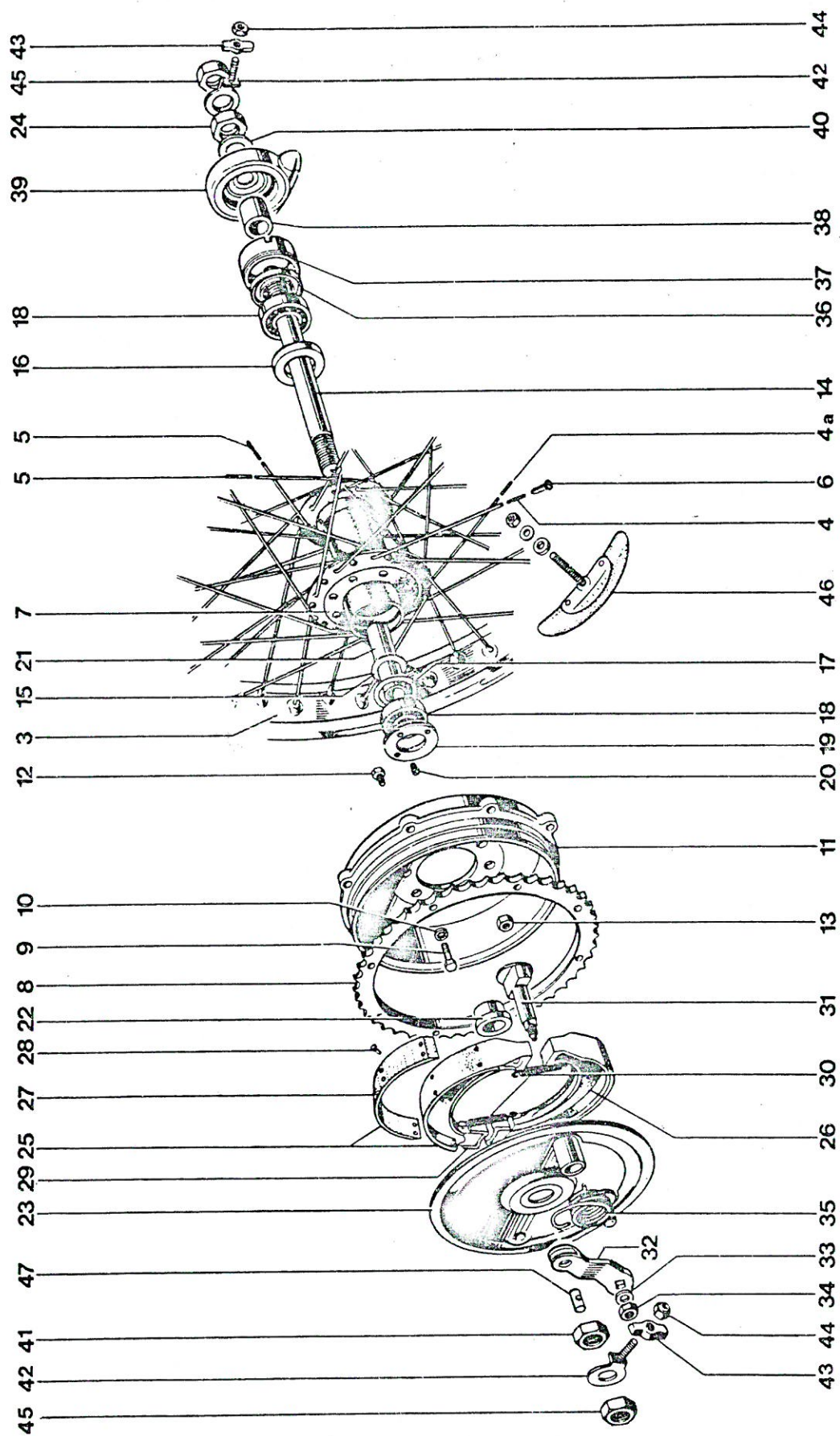
Fig. 18. REAR WHEEL
