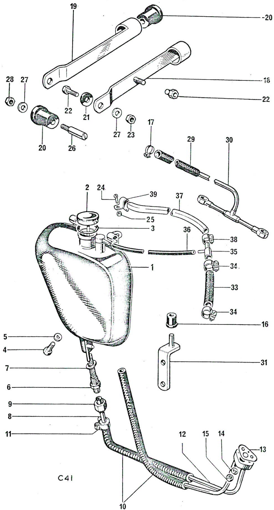
Fig. 23. OIL TANK
