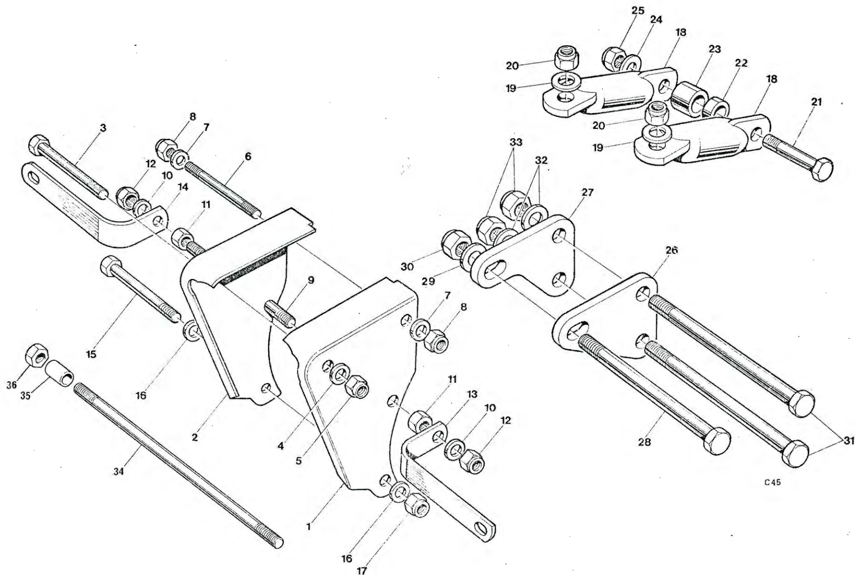
Fig. 13. MOTOR FITTINGS
