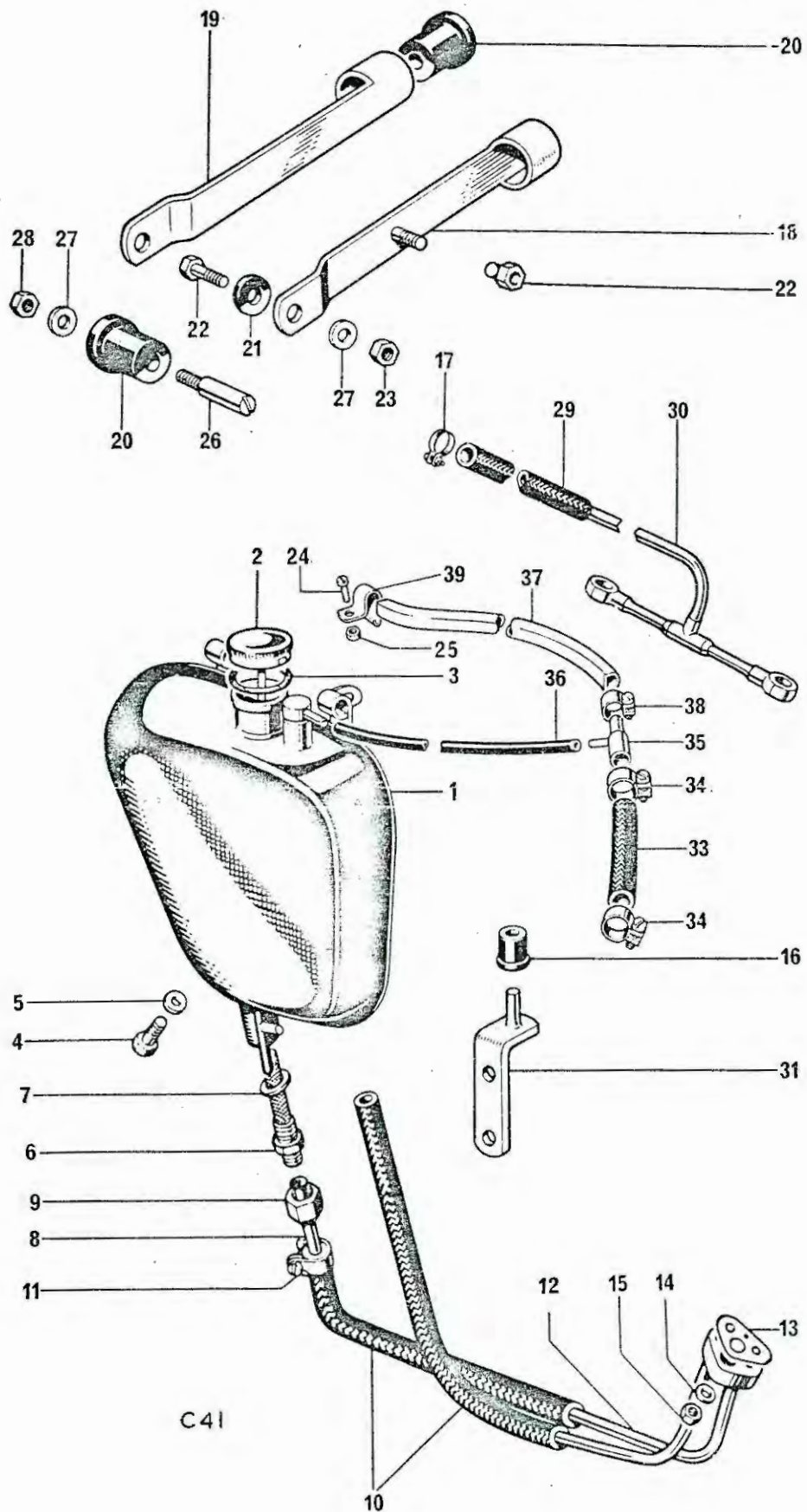
Fig. 23. OIL TANK
