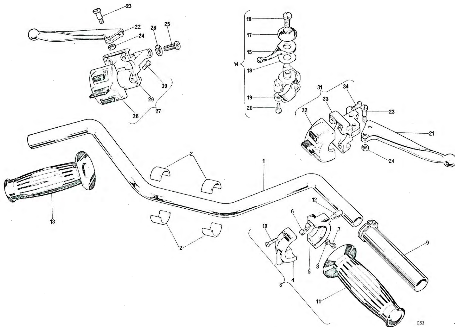
Fig. 25. HANDLEBAR AND CONTROL LEVERS
