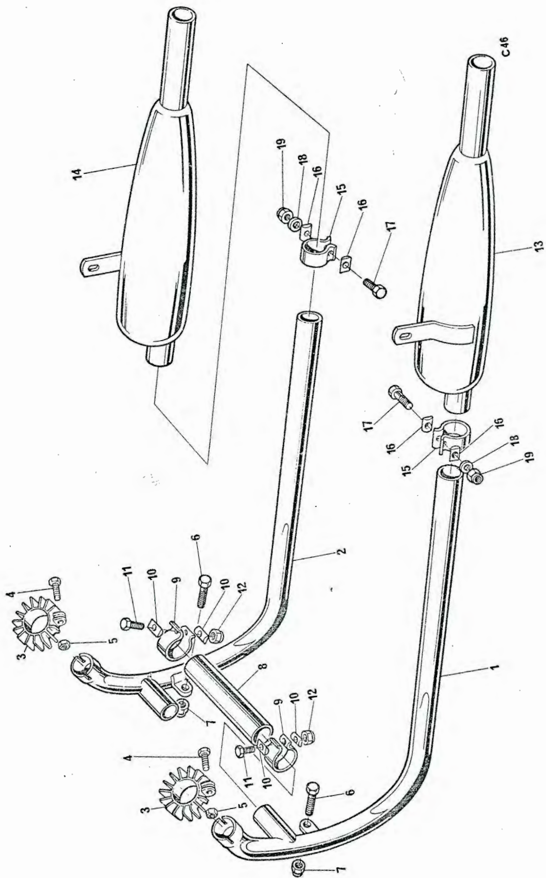
Fig. 12. EXHAUST SYSTEM
