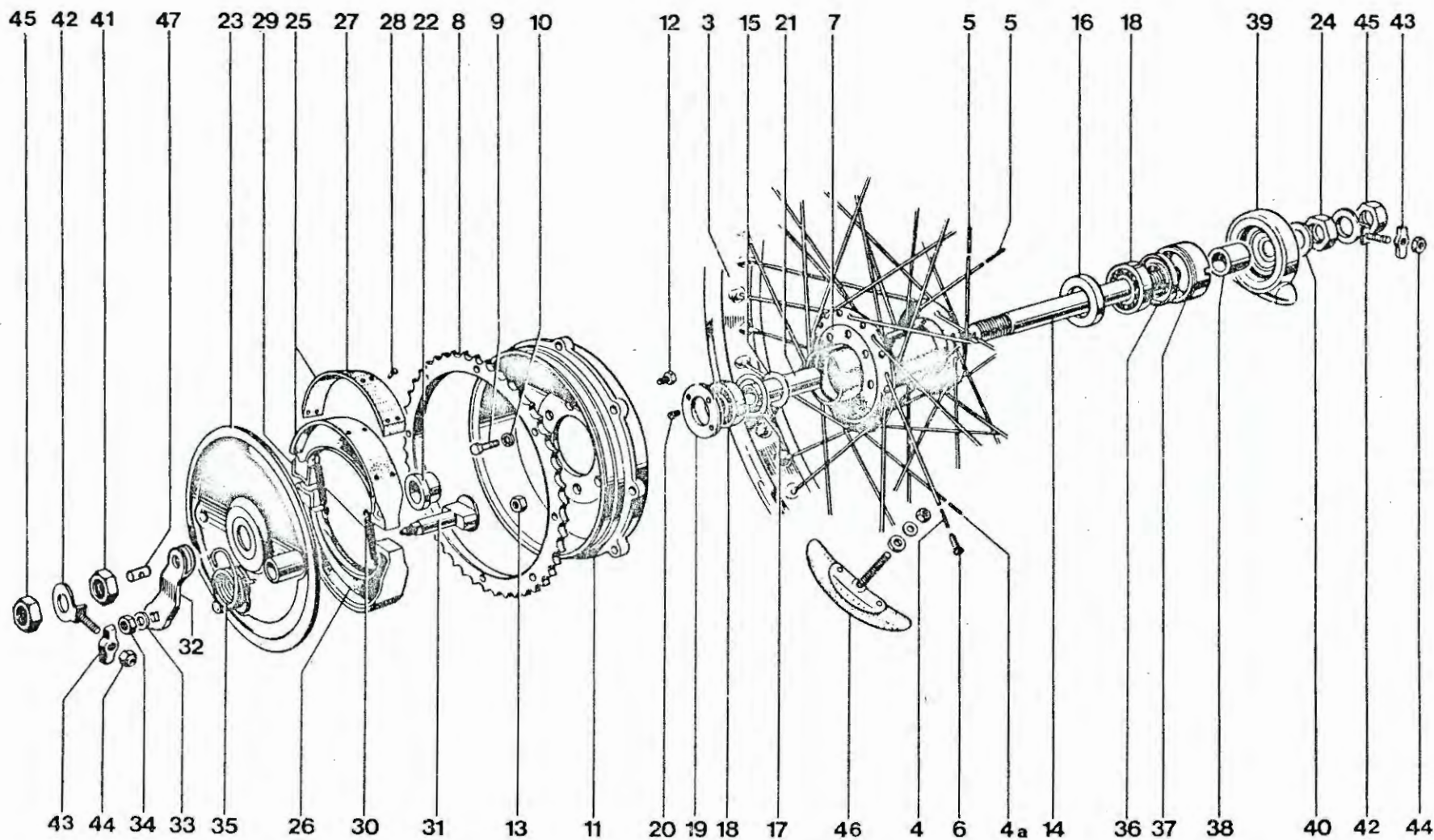
Fig. 18. REAR WHEEL
