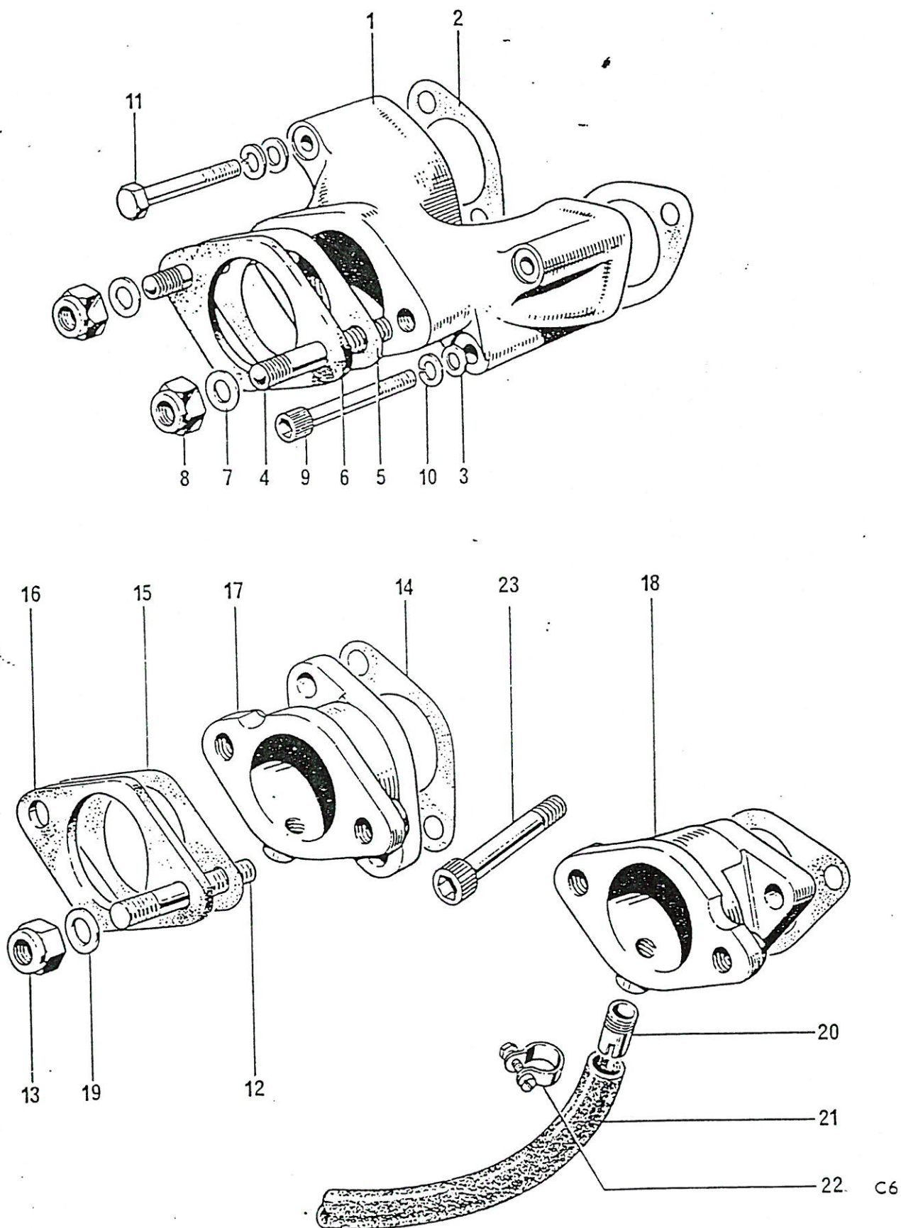
Fig. 4. INLET MANIFOLDS
