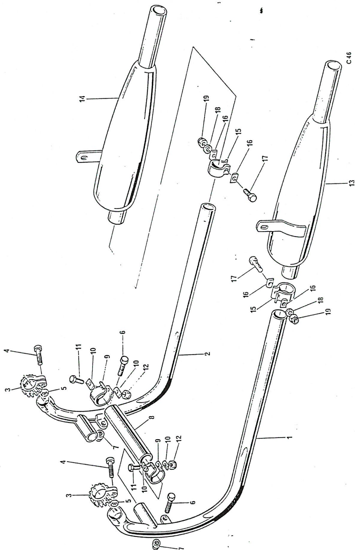
Fig. 15. EXHAUST SYSTEM
