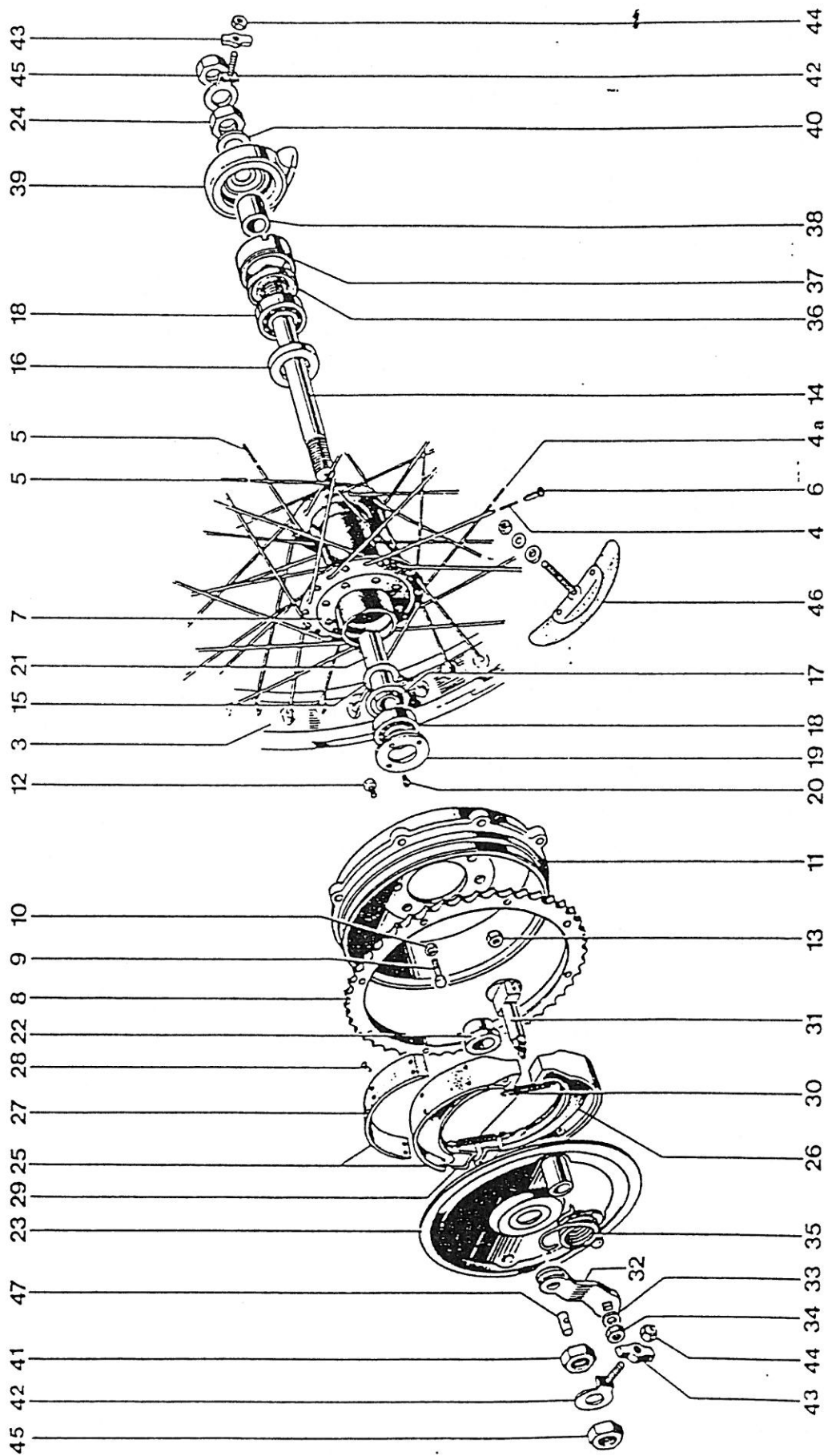
Fig. 23. REAR WHEEL
