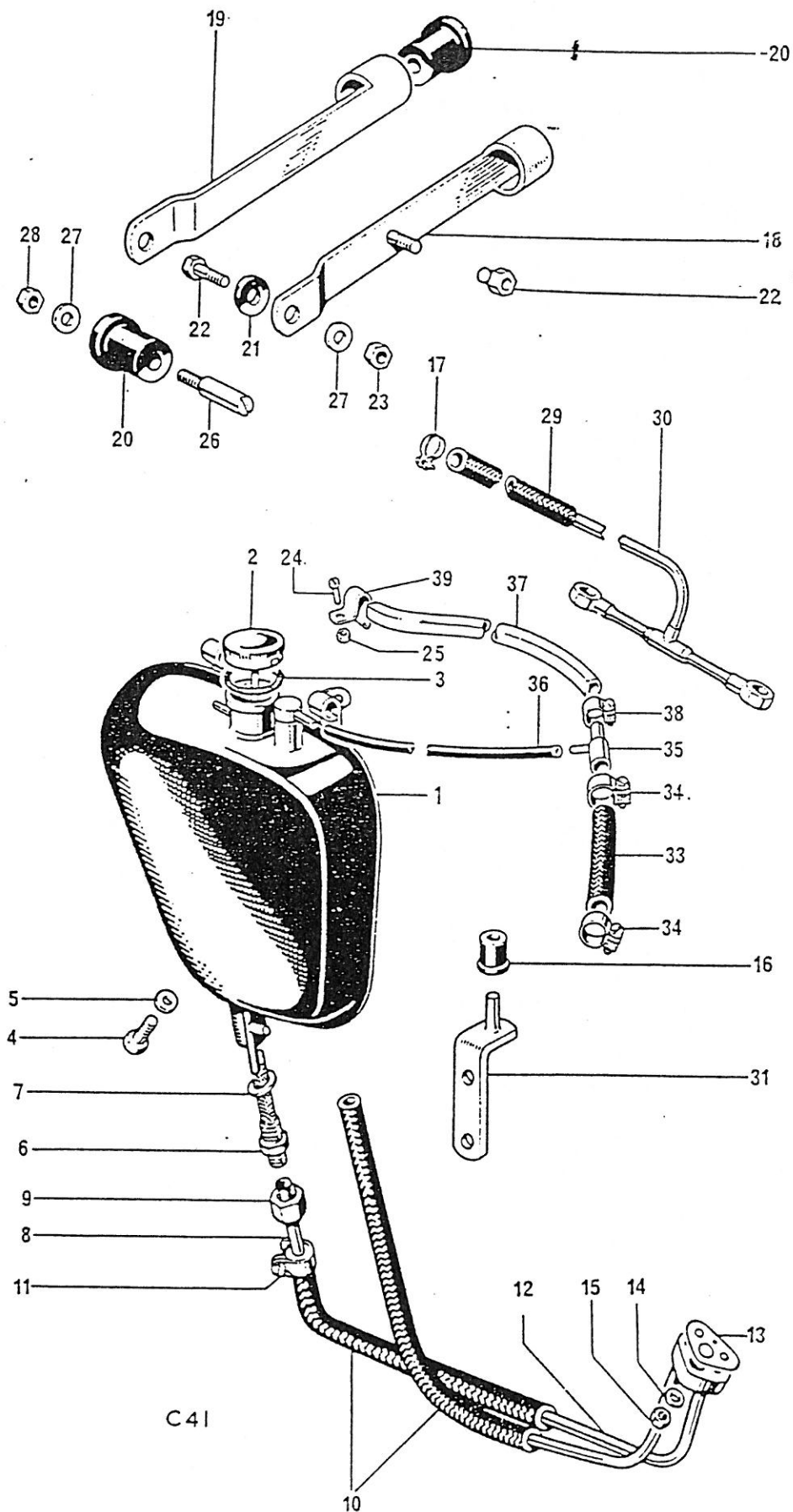
Fig. 28. OIL TANK
