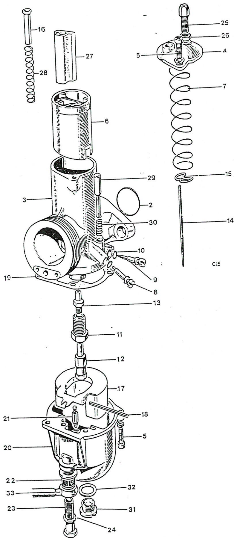
Fig. 5. CARBURETOR T100C
