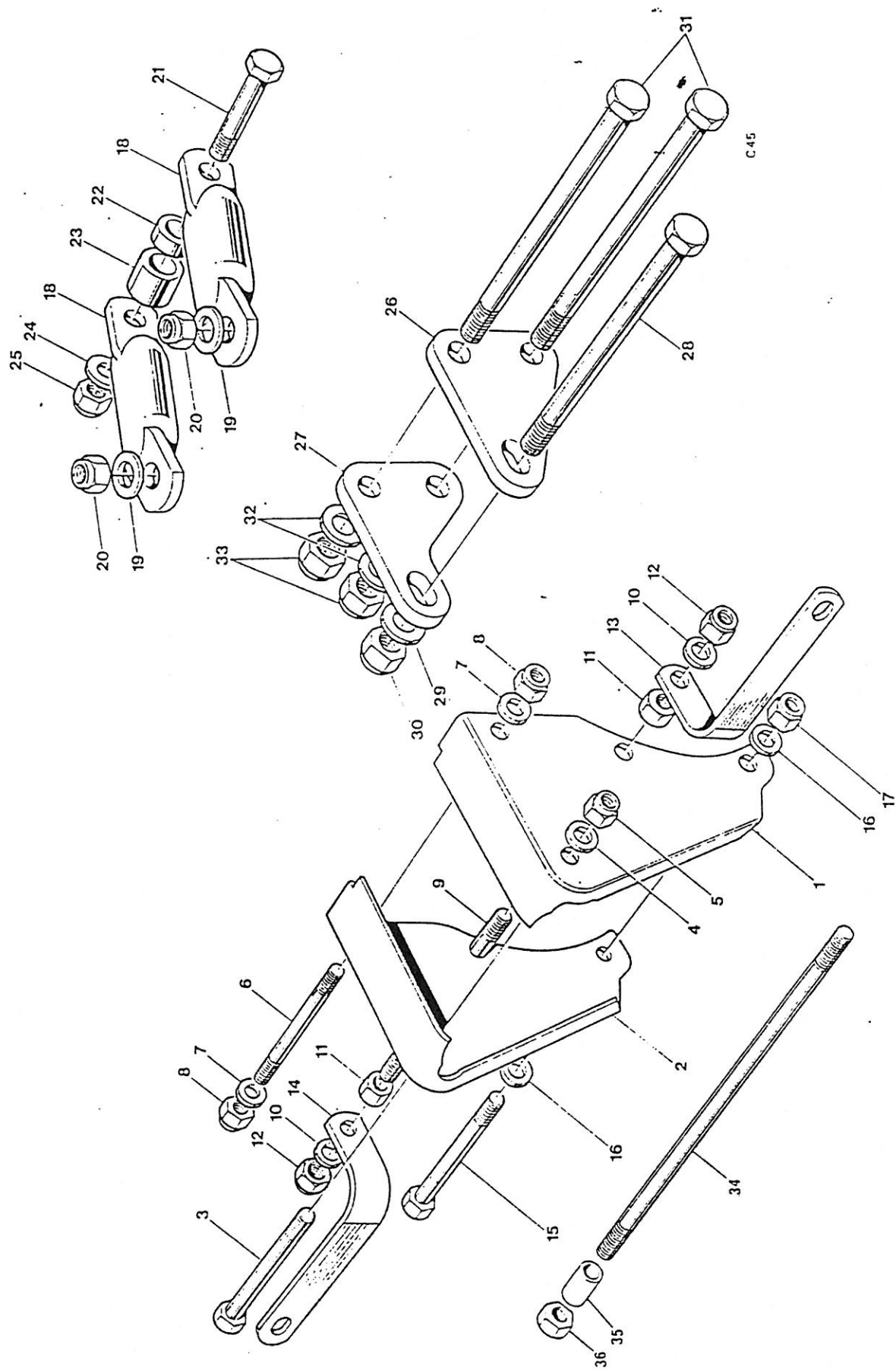
FIG. 16. MOTOR FITTINGS
