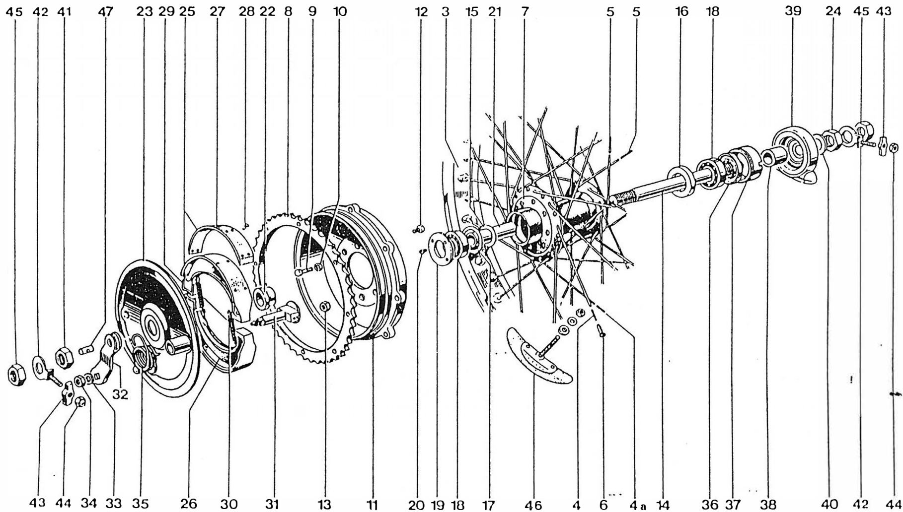
Fig. 23. REAR WHEEL
