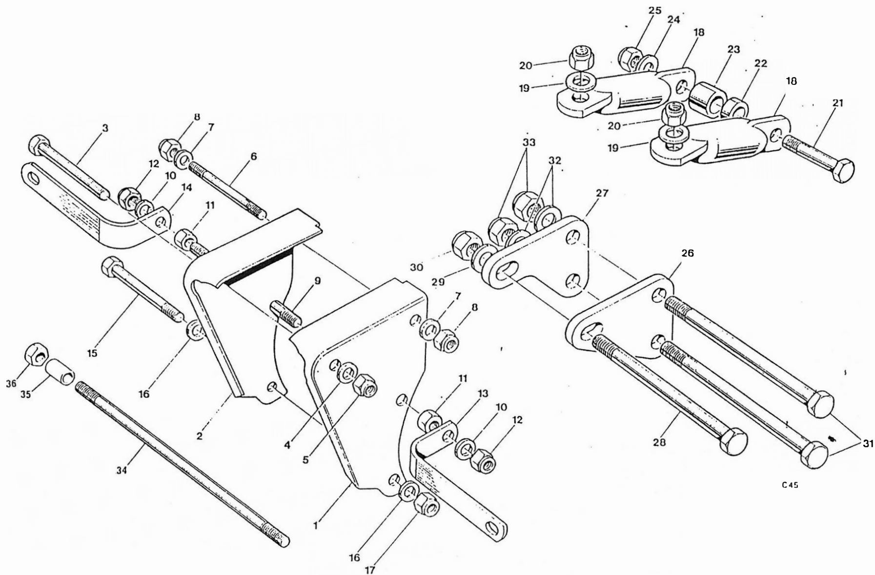
Fig. 16. MOTOR FITTINGS
