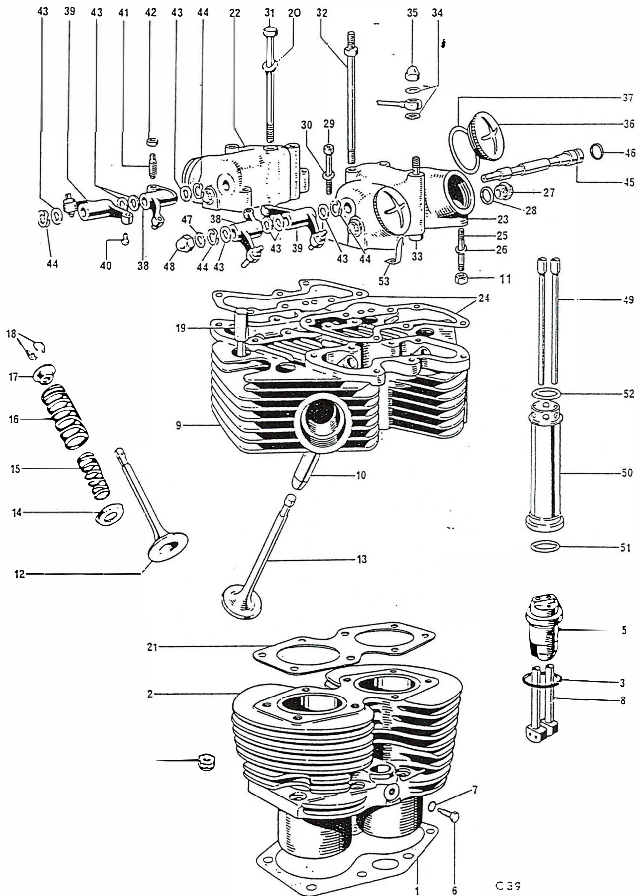
Fig. 7. CYLINDER BLOCK AND HEAD, T100C
