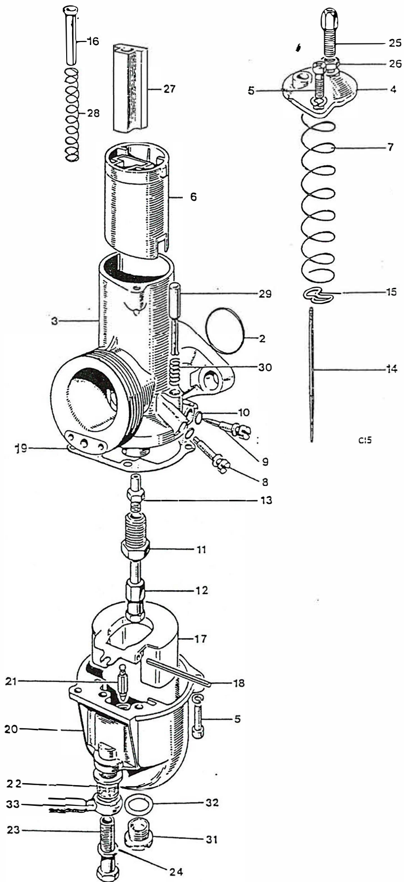
Fig. 6. CARBURETOR, T100R
