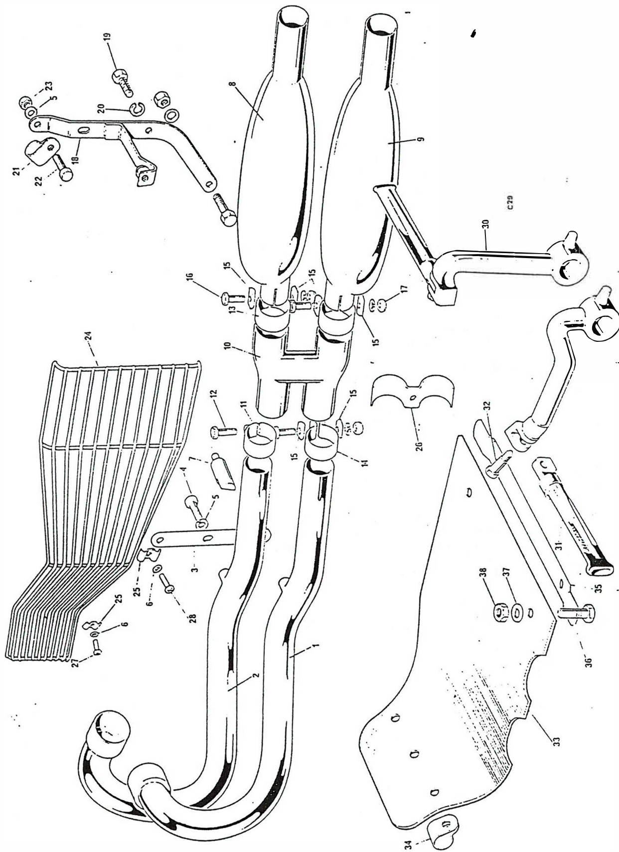
Fig. 17. EXHAUST P-PES UNDERSHIELD AND FOOTPEGS (T100C)
