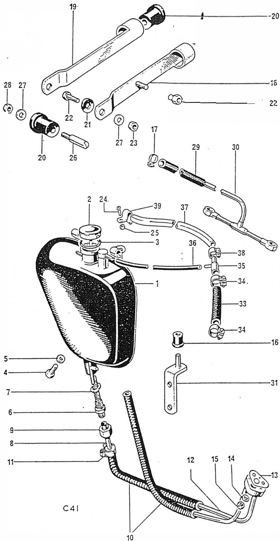
Fig. 28. OIL TANK
