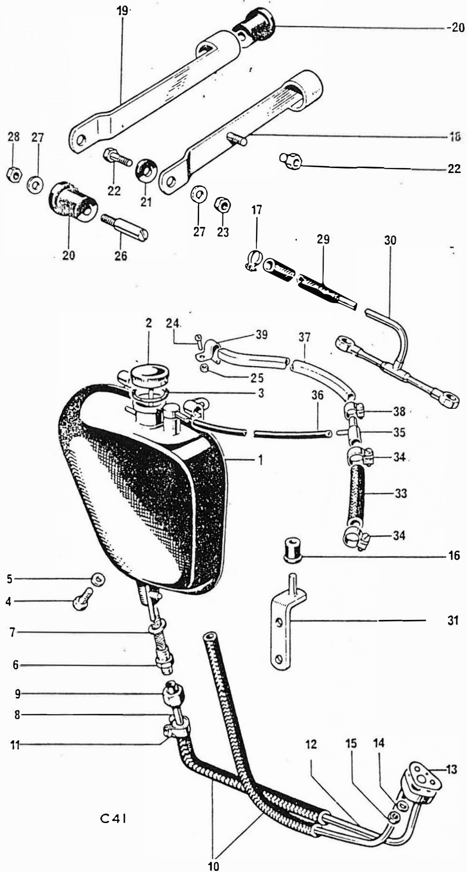
Fig. 28. OIL TANK
