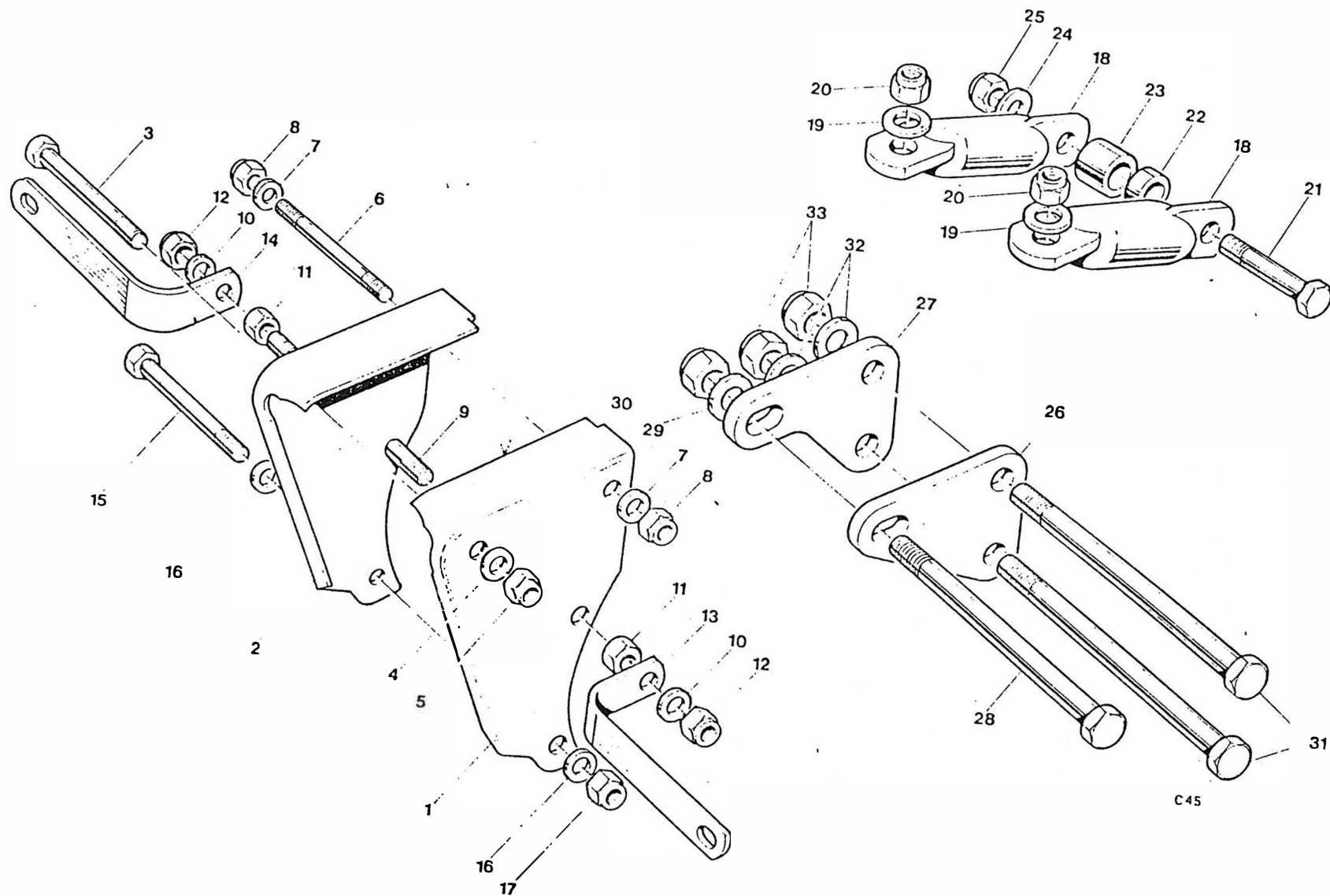
Fig. 16. MOTOR FITTINGS
